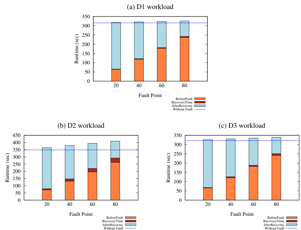
Figure 11. Recovery overhead analysis.
