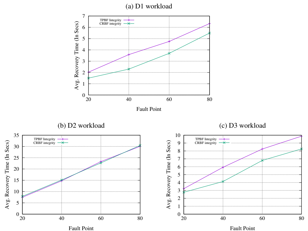
Figure 12. TPBF vs. CRBF recovery overhead analysis.
