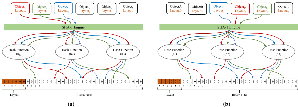
Figure 3. Data- and layout-aware Bloom filter. (a) DLBF insert operation. (b) DLBF query operation.
