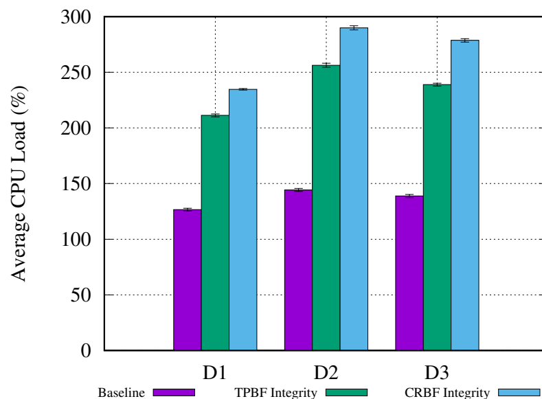
Figure 9. CPU load analysis.
