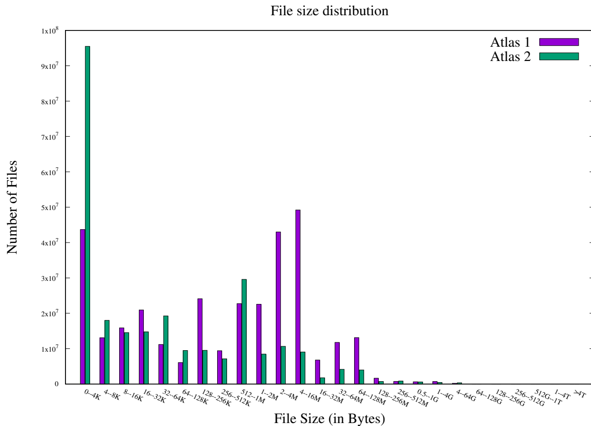
Figure 7. File size distribution.
