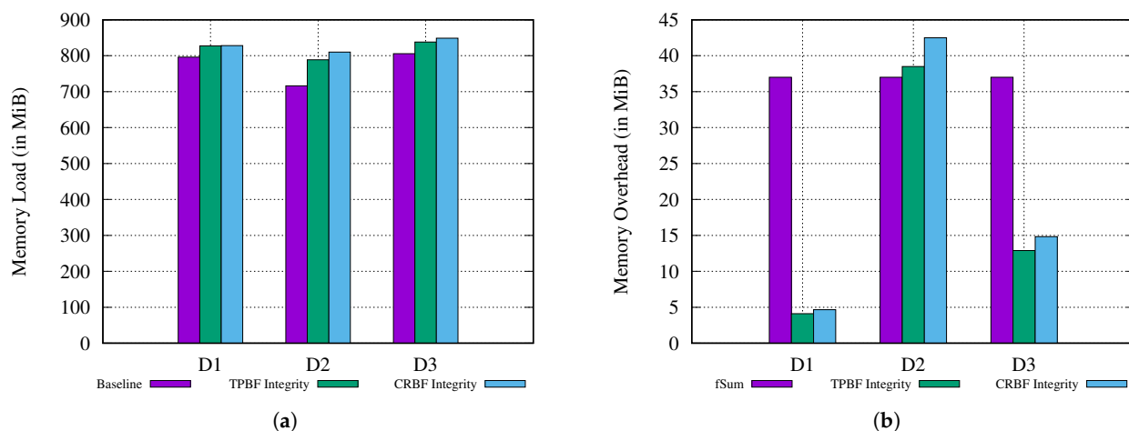
Figure 10. Memory load analysis. (a) Memory load comparison. (b) Bloom filter memory overhead comparison.
