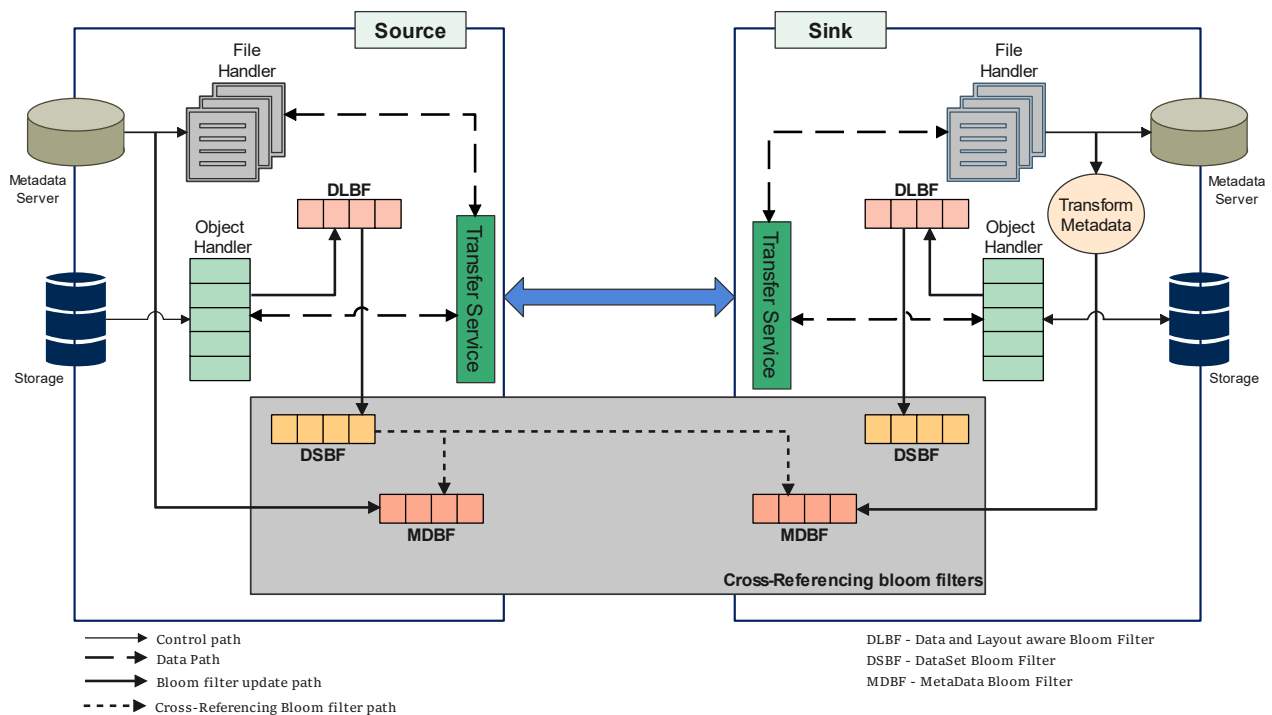
Figure 4. Cross-referencing Bloom-filter-based data integrity verification system.
