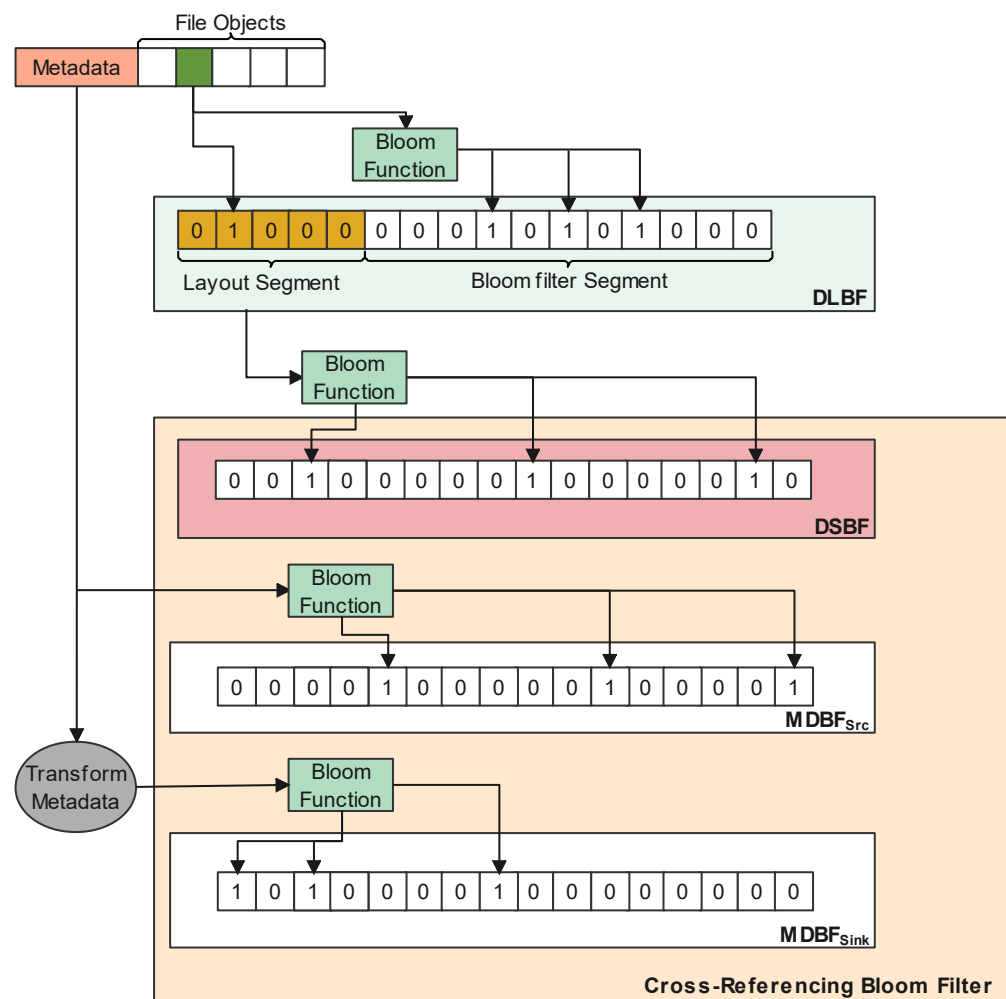
Figure 5. Cross-referencing Bloom filter data structure.
