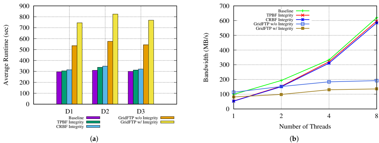
Figure 8. Data transfer performance analysis. (a) Data transfer time comparison. (b) Data transfer rate comparison for D3 workloads.
