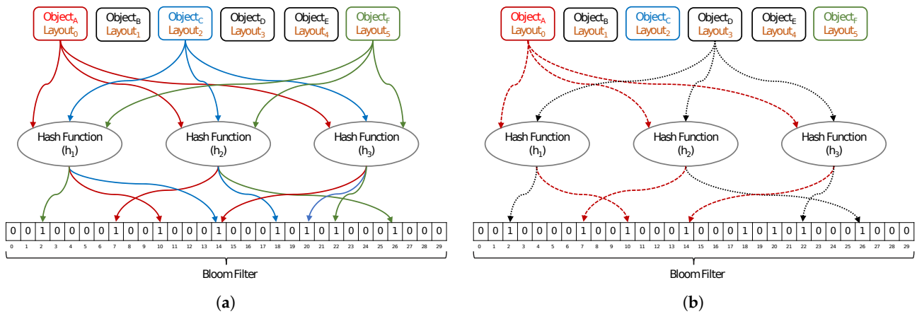
Figure 2. Standard Bloom filter. (a) Bloom filter insert operation. (b) Bloom filter query operation.
