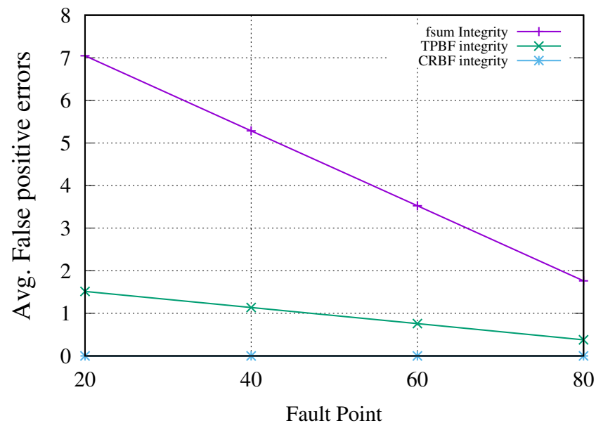
Figure 13. False-positive error analysis.
