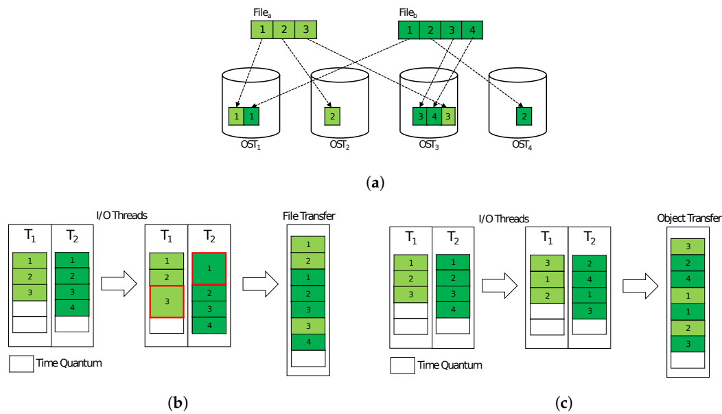
Figure 1. File distribution and transfer mechanisms. (a) File distribution. (b) State-of-the-art big data transfer mechanism. (c) Object-based big data transfer mechanism.
