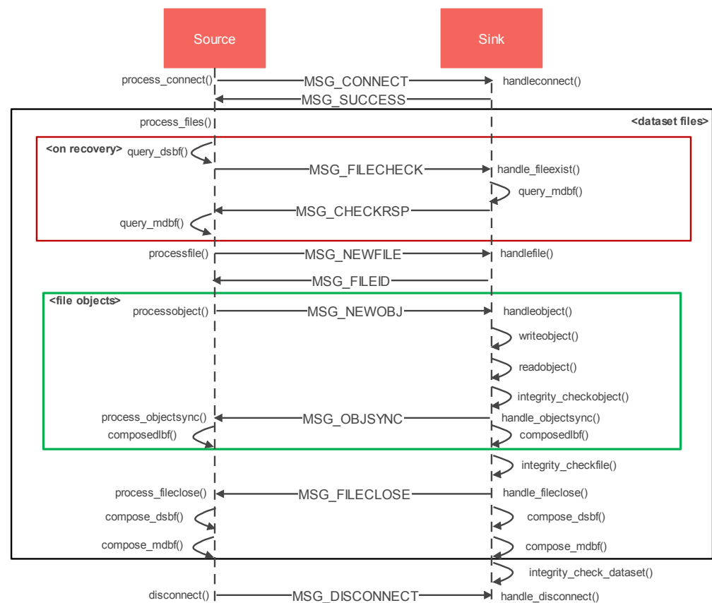
Figure 6. Communication sequence of the CRBF-based integrity framework.
