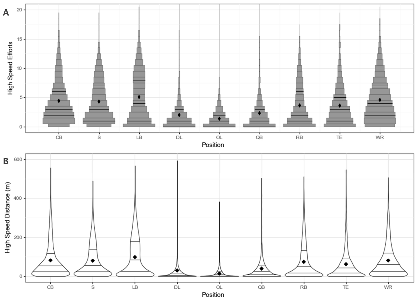
Figure 2. Distribution of high-velocity (A) efforts and (B) distance traveled by an NFL player during a regular season game based on position group. Horizontal lines represent the 25th, 50th, and 75th percentiles, and the diamond denotes the average value for each position group.
