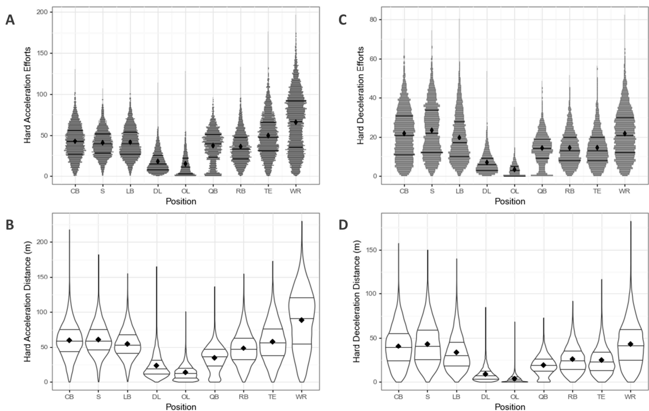
Figure 3. Distribution of (A) acceleration efforts, (B) acceleration distance, (C) deceleration efforts, and (D) deceleration distance accumulated by an NFL player during a regular season game based on position group. Horizontal lines represent the 25th, 50th, and 75th percentiles, and the diamond denotes the average value for each position group.
