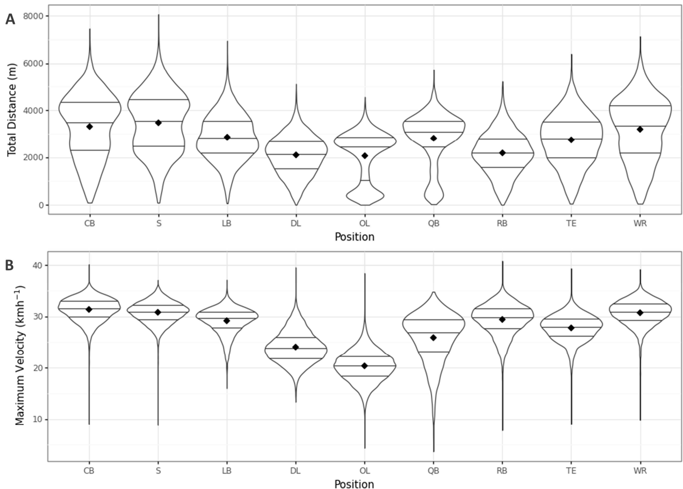
Figure 1. Distribution of (A) total distance and (B) maximum velocity by an NFL player during a regular season game based on position group. Horizontal lines represent the 25th, 50th, and 75th percentiles, and the diamond denotes the average value for each position group.
