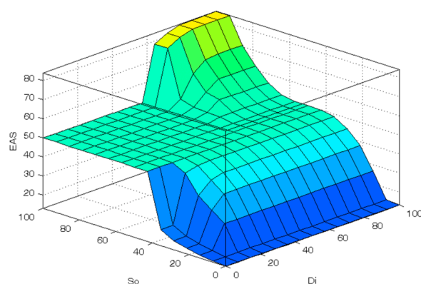
Figure 9. 3D graph of inputs (So: sulfate ion concentration, Di: concrete disintegration) and output (EAS: corrosion due to sulfate attack).
