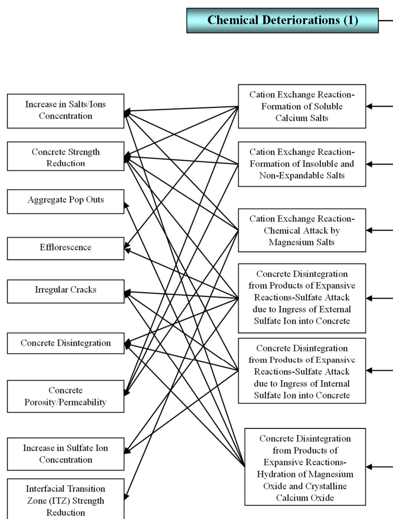
Figure 1. Symptoms and types of chemical deteriorations.
