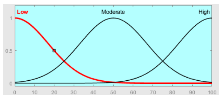
Figure 5. Membership function of chemical deterioration types.
