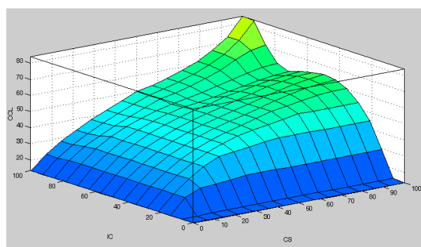
Figure 6. 3D graph of inputs (CS: steel corrosion, IC: chlorine ion), and output (CCL: reinforced concrete corrosion due to chlorine ion diffusion).
