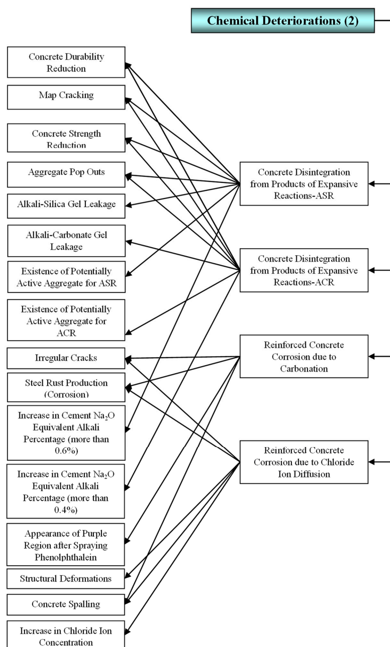
Figure 2. Symptoms and types of chemical deteriorations.
