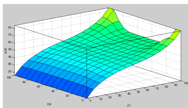
Figure 7. 3D graph of inputs (DS: reduction of concrete strength, JC: ACG leakage) and output (ACR: alkali-carbonate reaction of aggregates).
