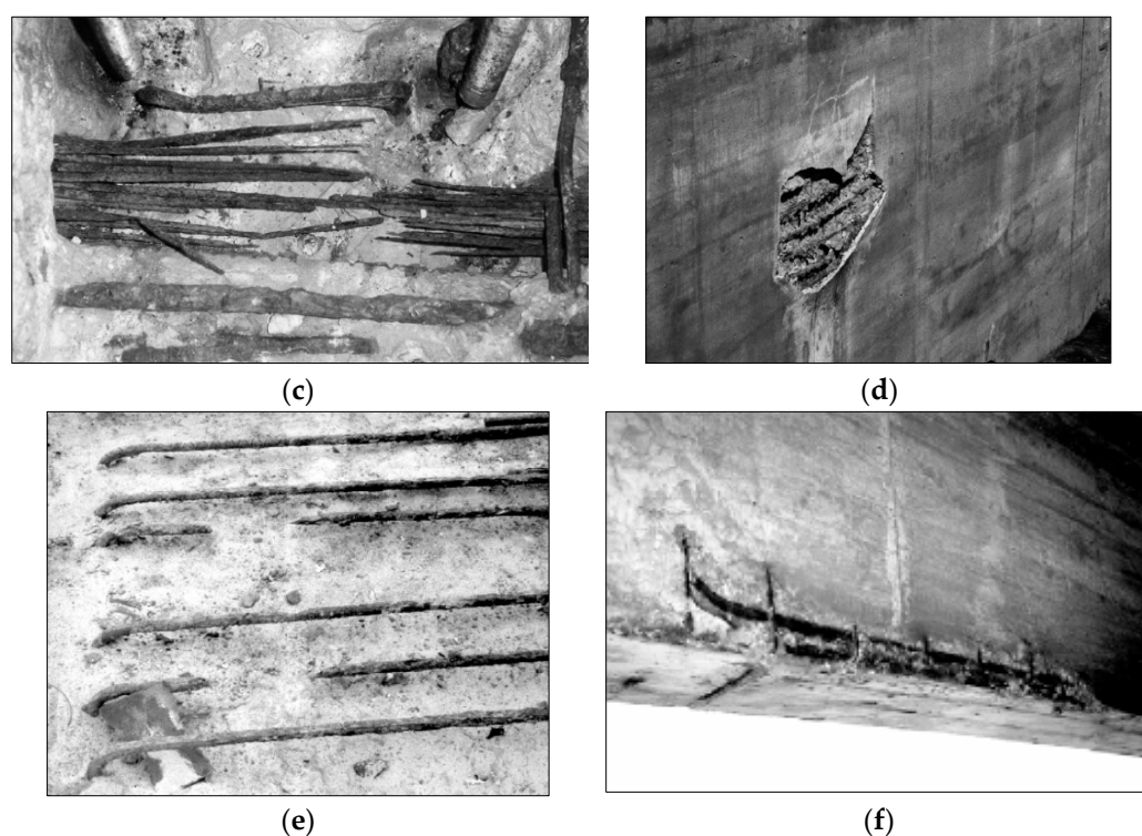
Figure 10. (a) Typical deterioration observed for a bridge in Sado River, Portugal in the splash and tidal zones; (b) concrete spalling in a construction joint; (c) corrosion of prestressing steel in ungrouted ducts; (d) macro-corrosion cell in dock walls; (e) bars with 25 mm diameter totally corroded; (f) concrete spalling in a low cover zone [35].
