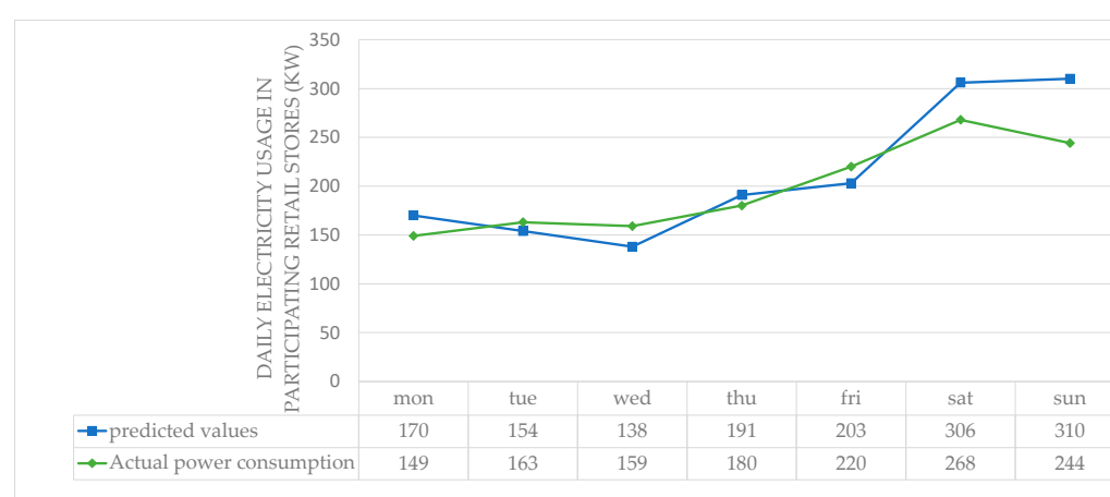
Figure 4. Daily electricity consumption prediction and comparison of actual power consumption in participating retail stores.
