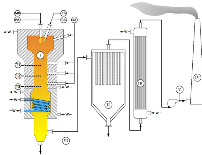
Figure 1. Scheme of a technical-scale installation used for combustion of liquid fuels. MB—main burner (liquid fuels: FADR and HFO), PB—pilot burner (fuel: natural gas), PA—primary air, SA—secondary air, W—water for cooling, I—combustion chamber, II—dust separator, III—exhaust gas cooler, IV—chimney, V—exhaust gas sampling point, VI—O 2 measurement in raw exhaust gas. Reprinted from [24] (upon permission of Elsevier, License Number 5656340853661).
