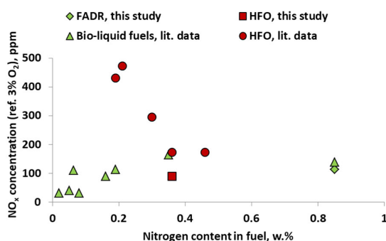
Figure 11. The emission of NO x in the function of N-fuel content, data from [9,12,16,18,43,47,50].
