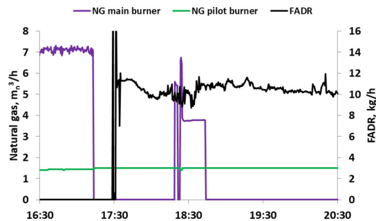
Figure 7. The flow rate of gaseous (natural gas, NG) and liquid (FADR) fuels as a function of time.
