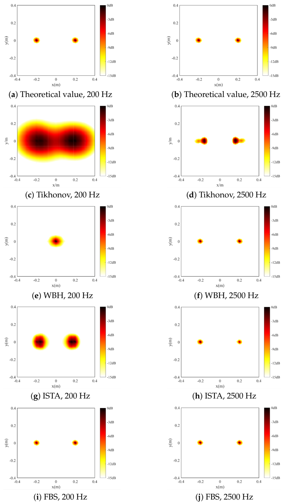
Figure 7. Calculated sound pressure level diagram of 200 Hz and 2500 Hz coherent sound sources.
