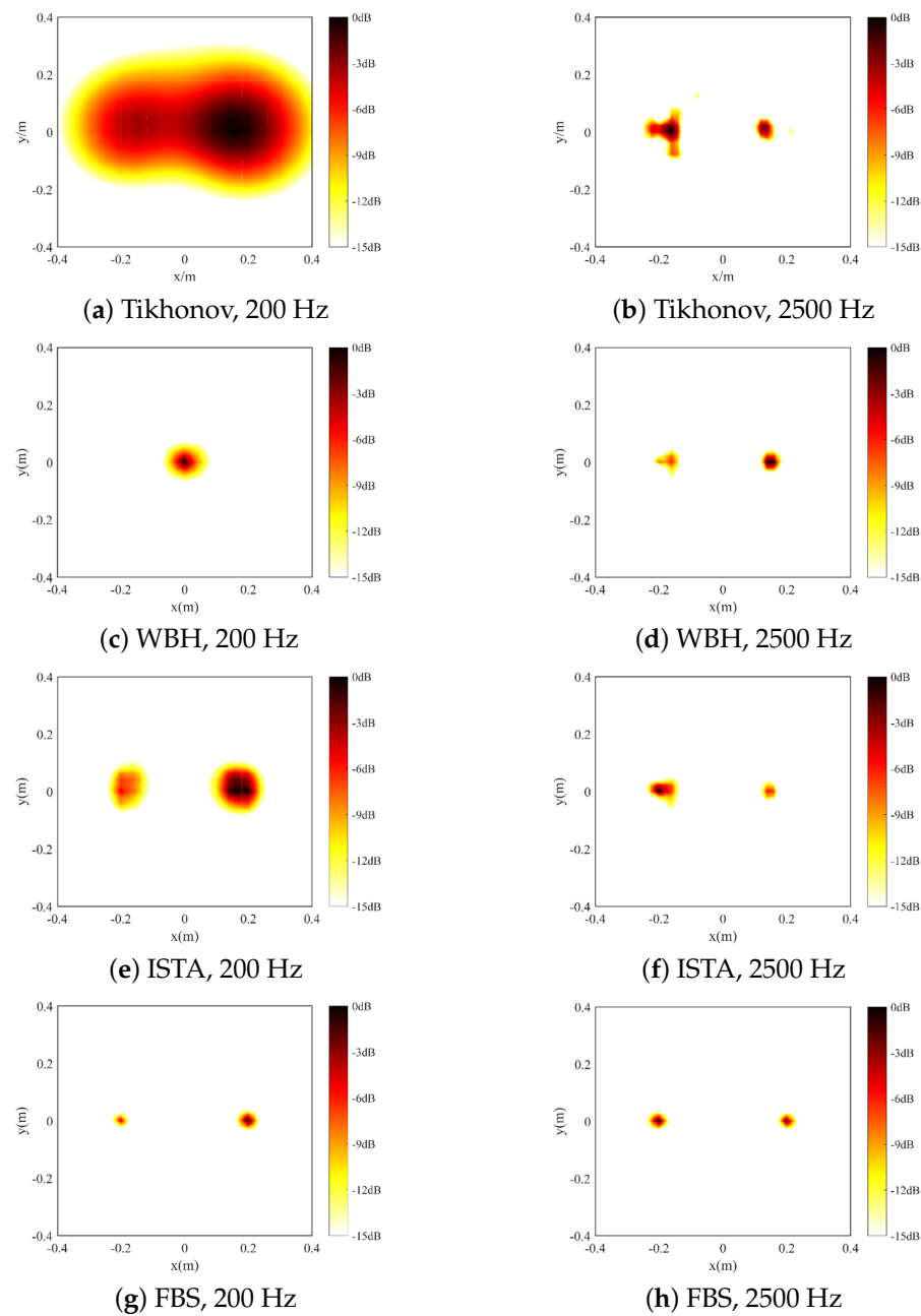
Figure 12. Reconstructed sound pressure level diagram of 200 Hz and 2500 Hz coherent sound sources.
