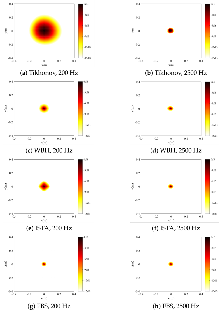
Figure 11. Reconstructed sound pressure level diagram of 200 Hz and 2500 Hz single sound source.
