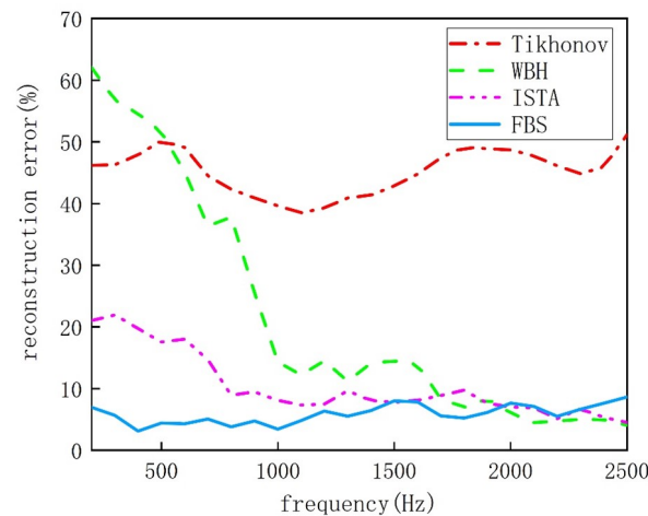
Figure 8. Coherent source reconstruction errors between Tikhonov, WBH, ISTA, and FBS.
