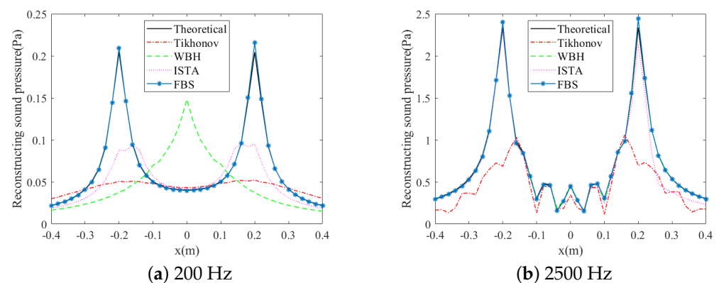
Figure 6. Reconstructed sound pressure amplitude of a single sound source along the middle row of the reconstructed surface.
