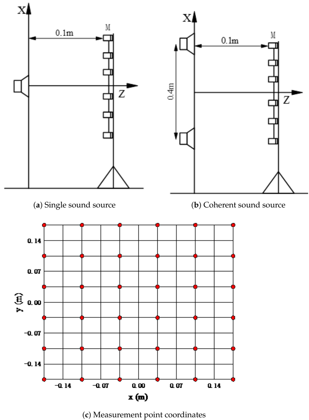
Figure 2. Schematic diagram of sound source layout.
