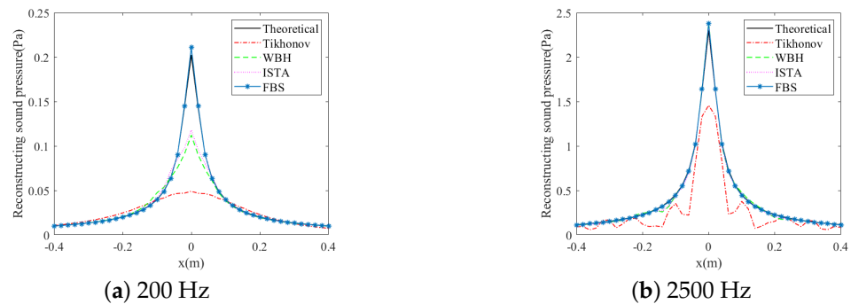
Figure 4. Reconstructed sound pressure amplitude of a single sound source along the middle row of the reconstructed surface.
