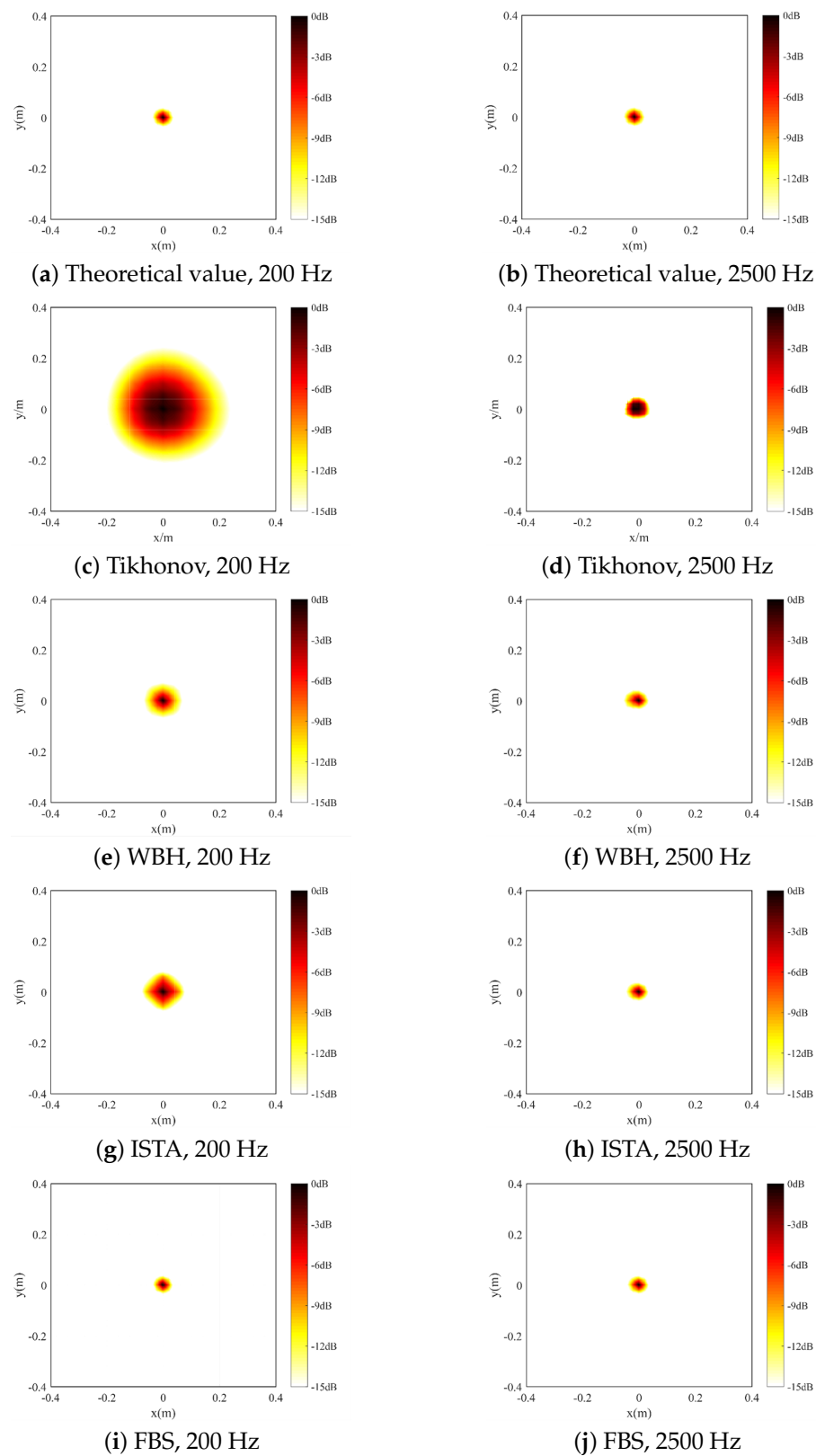
Figure 3. The calculated sound pressure level of single sound source at 200 Hz and 2500 Hz.
