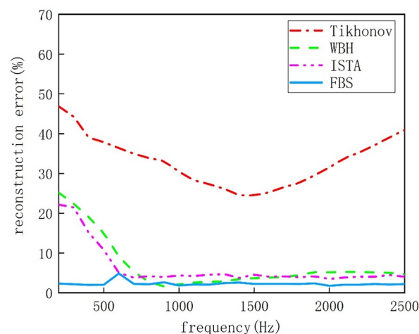
Figure 5. Single source reconstruction errors between Tikhonov, WBH, ISTA, and FBS.
