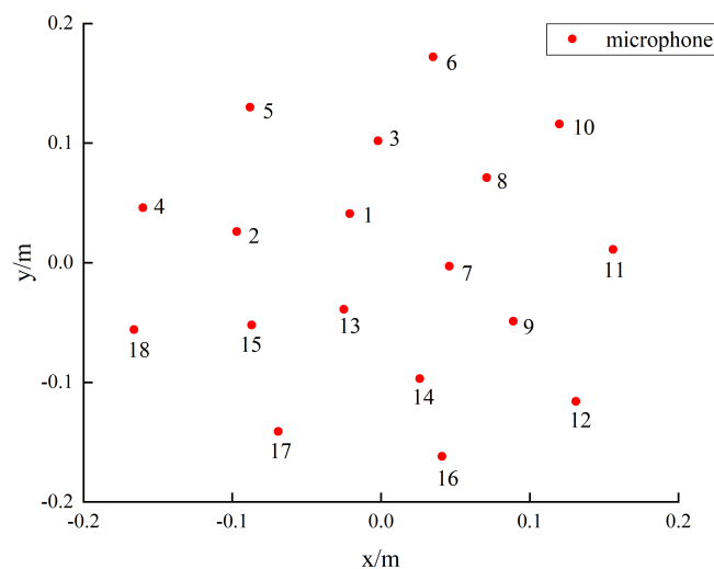
Figure 9. Microphone array coordinates.
