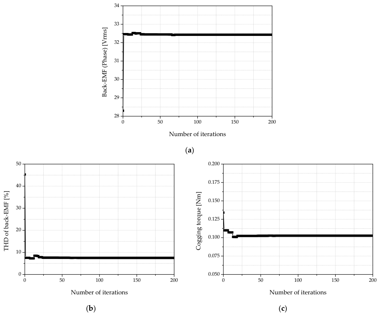
Figure 7. Convergence results of the objective function: (a) y1 (magnitude of back-EMF), (b) y2 (total harmonic distortion (THD)), (c) y3 (peak to peak value of cogging torque).
