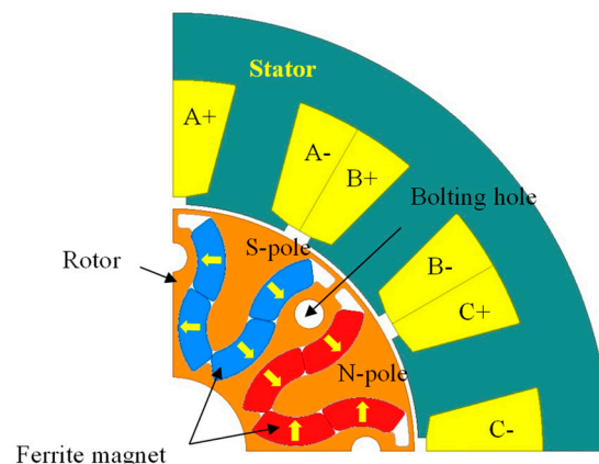
Figure 1. Typical structure of flared-shaped IPM motor (1/4 model).
