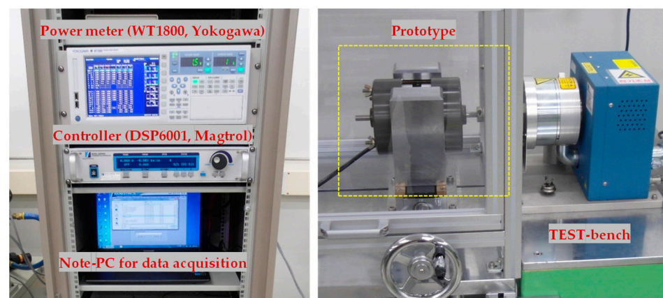
Figure 12. Experiment setup (test bench).
