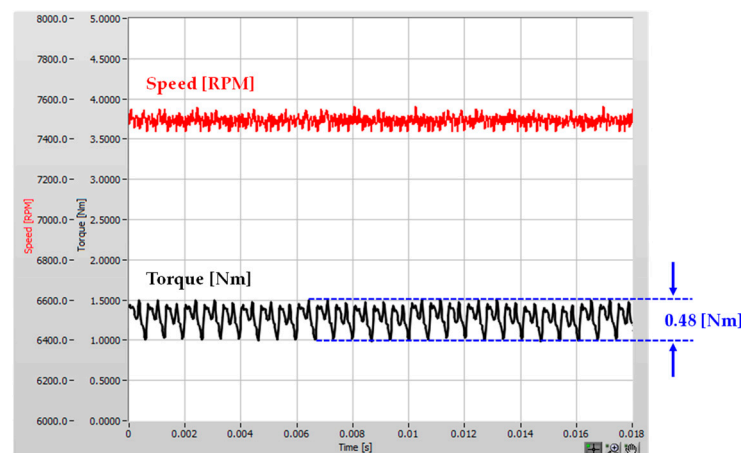
Figure 16. Experimental results of the prototype at the rated load.
