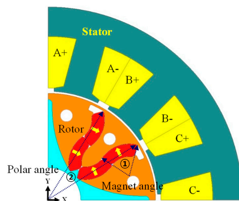
Figure 5. Design variables of basic FCPM model.
