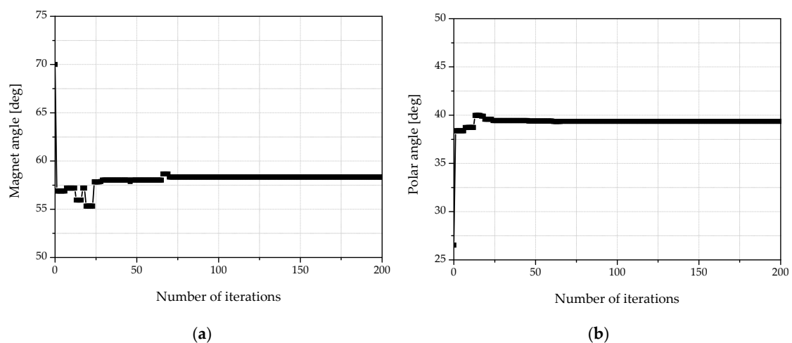
Figure 6. Convergence results of the design variables: (a) magnet angle, (b) polar angle.
