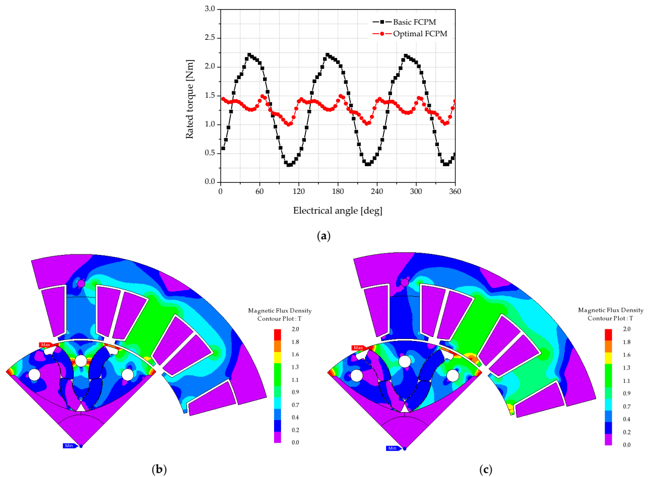
Figure 10. Rated load analysis result after optimization: (a) rated torque waveforms, (b) flux density of basic FCPM model, (c) flux density of optimal FCPM model.
