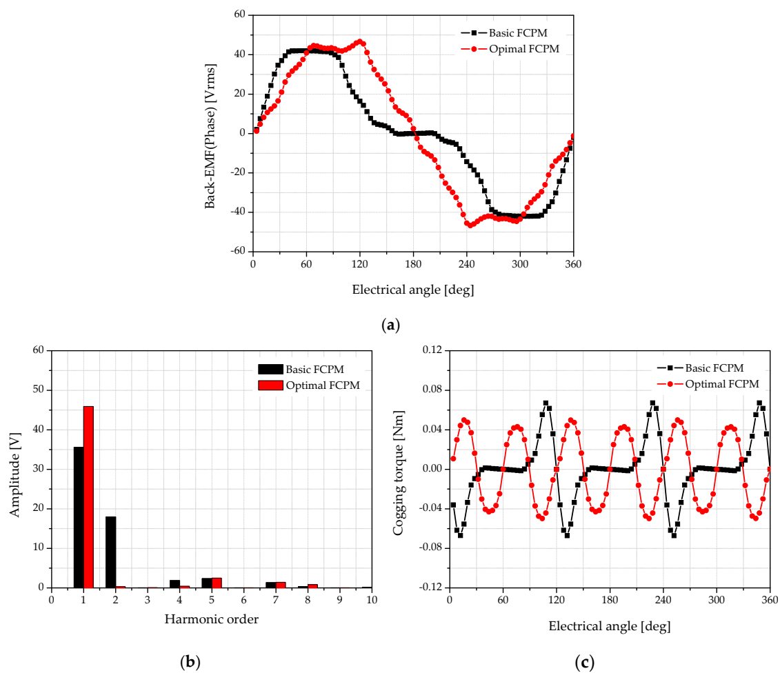
Figure 9. No-load analysis results after optimization: (a) back-EMF, (b) total harmonic order, (c) cogging torque.
