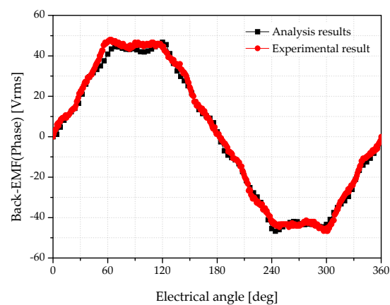
Figure 15. Comparison of back-EMF waveform for optimal model (at 900 rpm).
