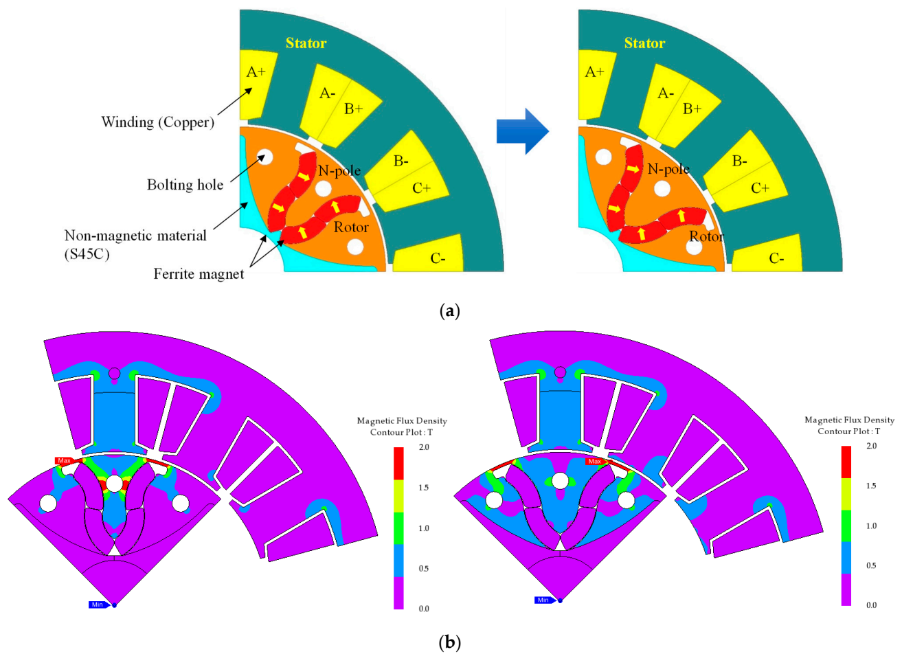
Figure 8. Comparison of rotor assembly shape and flux density under no-load condition: (a) the rotor assembly shape of basic FCPM model and optimal FCPM model (1/4 model), (b) flux density under no-load condition.
