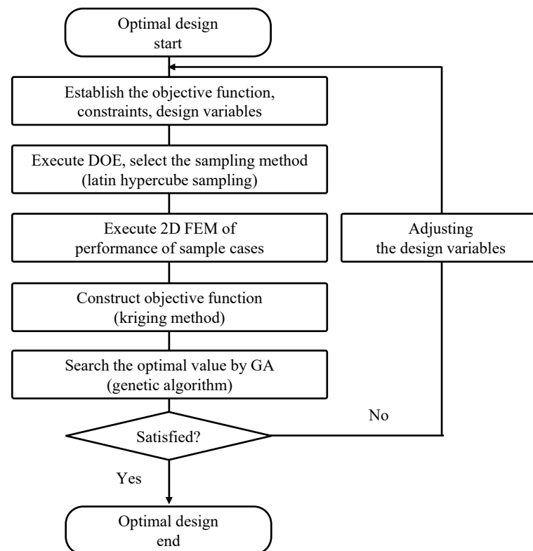
Figure 4. Optimal design process.
