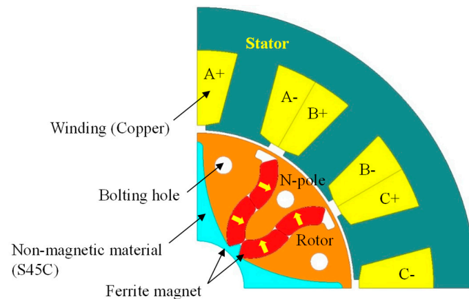
Figure 2. Proposed flared-type CP IPM motor (1/4 model).
