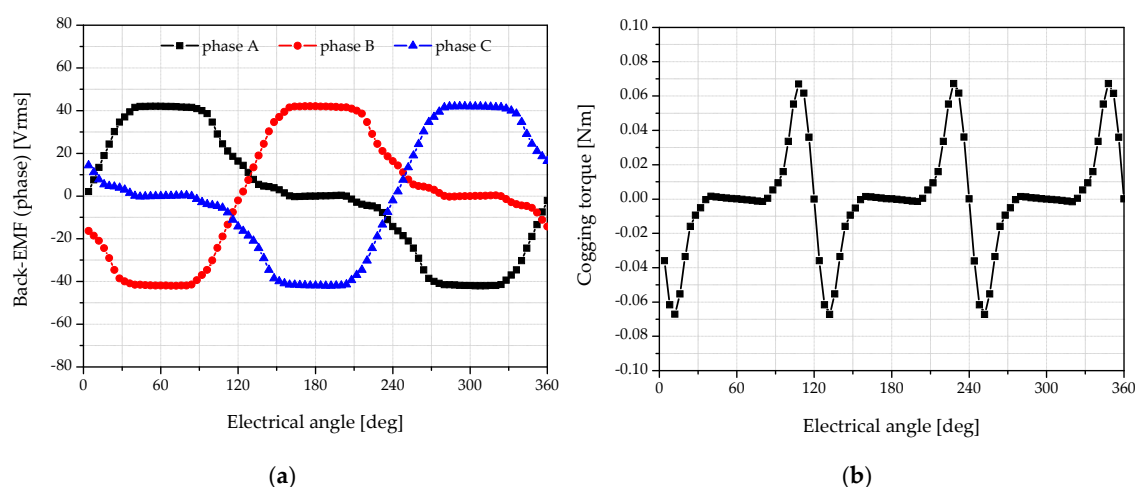
Figure 3. Analysis results of no-load conditions (7500 rpm): (a) back-EMF, (b) cogging torque.
