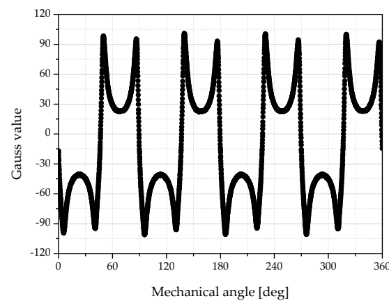
Figure 14. Surface gauss value of the optimal FCPM rotor assembly.
