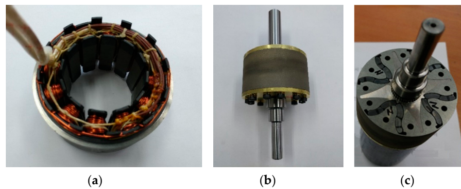
Figure 11. Prototype of the optimal FCPM model: (a) stator assembly, (b) rotor assembly, (c) the PM arrangement inside the rotor assembly.
