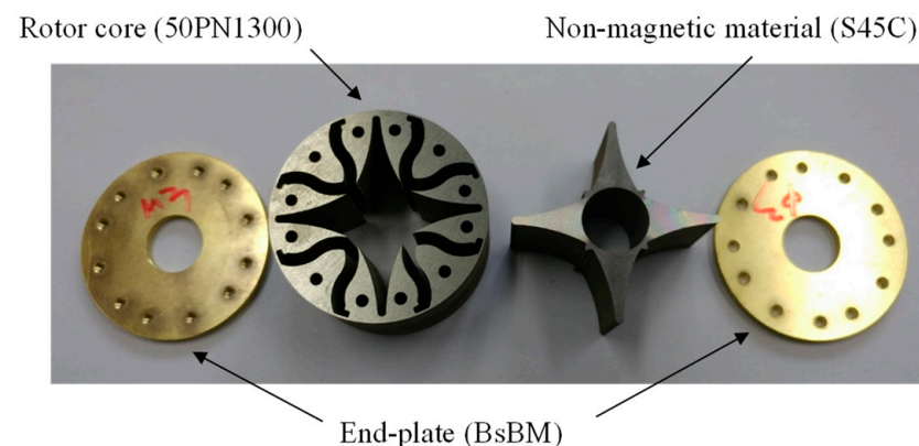
Figure 13. Rotor assembly of the prototype.
