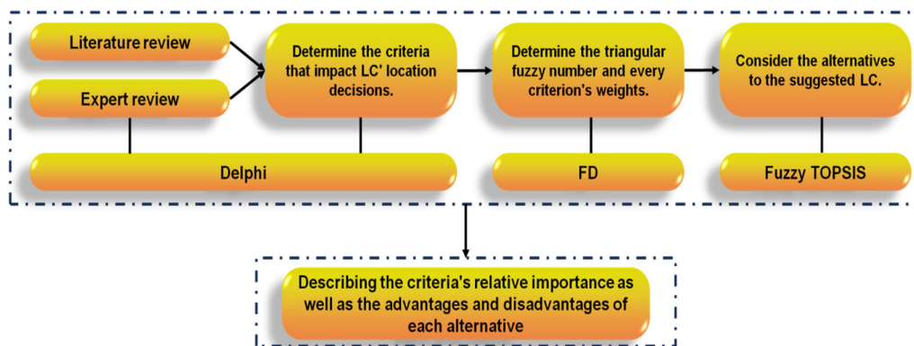
Figure 1. FD–TOPSIS methodology.
