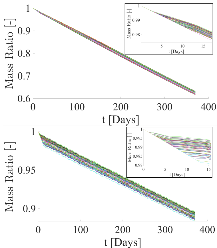
Figure 6. Time histories of the mass ratio for the first target orbit (in the insets, zoom on the acquisition phase). (top) Circular orbit. (bottom) Elliptic orbit with assigned r_{Pmin} / r_{Amax} .
