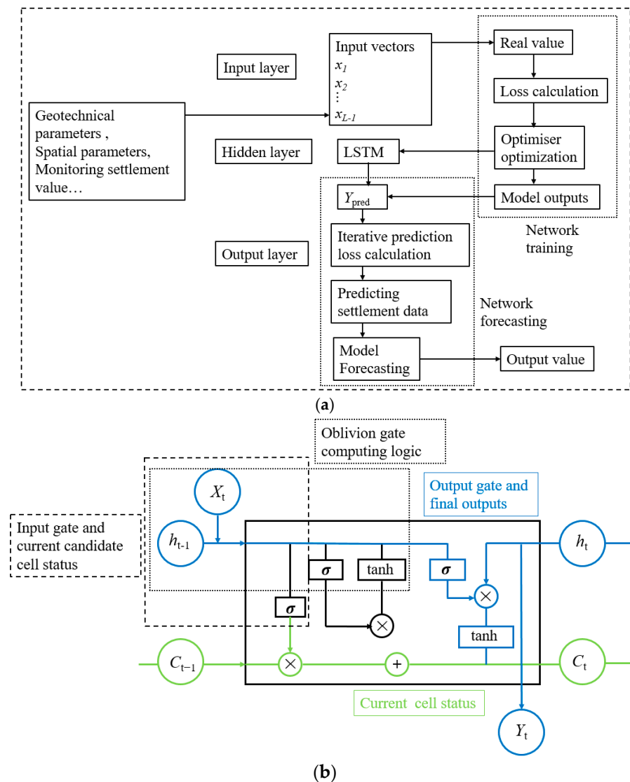
Figure 4. LSTM model. (a) Model prediction flowchart. (b) LSTM unit structure.
