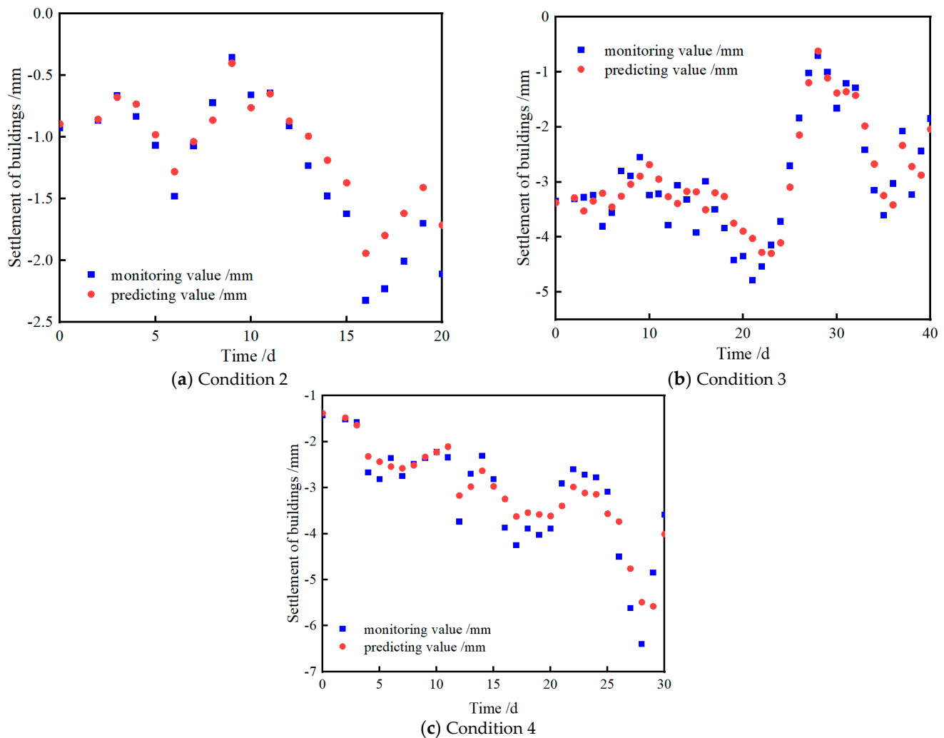
Figure 6. Comparison of settlement monitoring values and predicted values for various conditions of the open-cut method.
