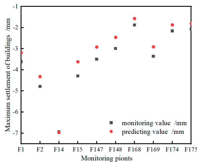
Figure 5. Predicted and monitoring of maximum settlements at measuring points.
