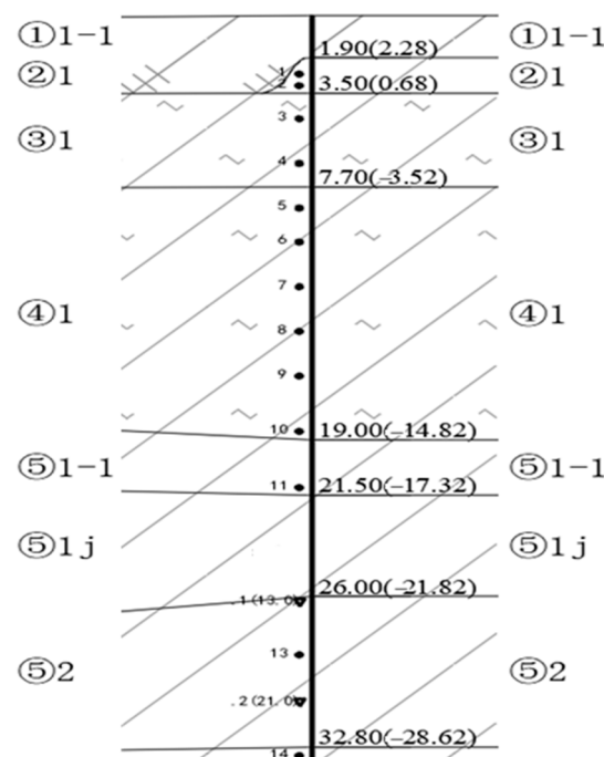
Figure 2. A cross section with geological geotechnical detailing.
