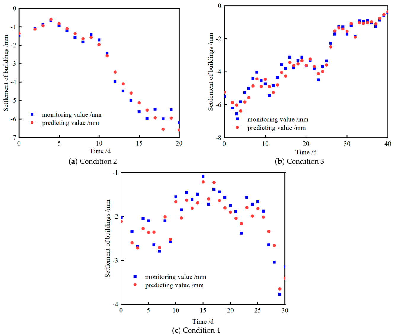
Figure 7. Comparison of settlement monitoring values and predicted values for various conditions of the total reverse method.
