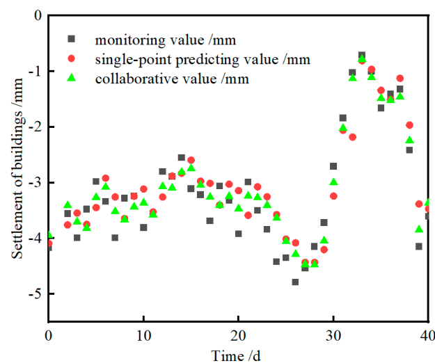
Figure 10. Comparison of single-point predicted and multi-point co-predicted and monitored values.
