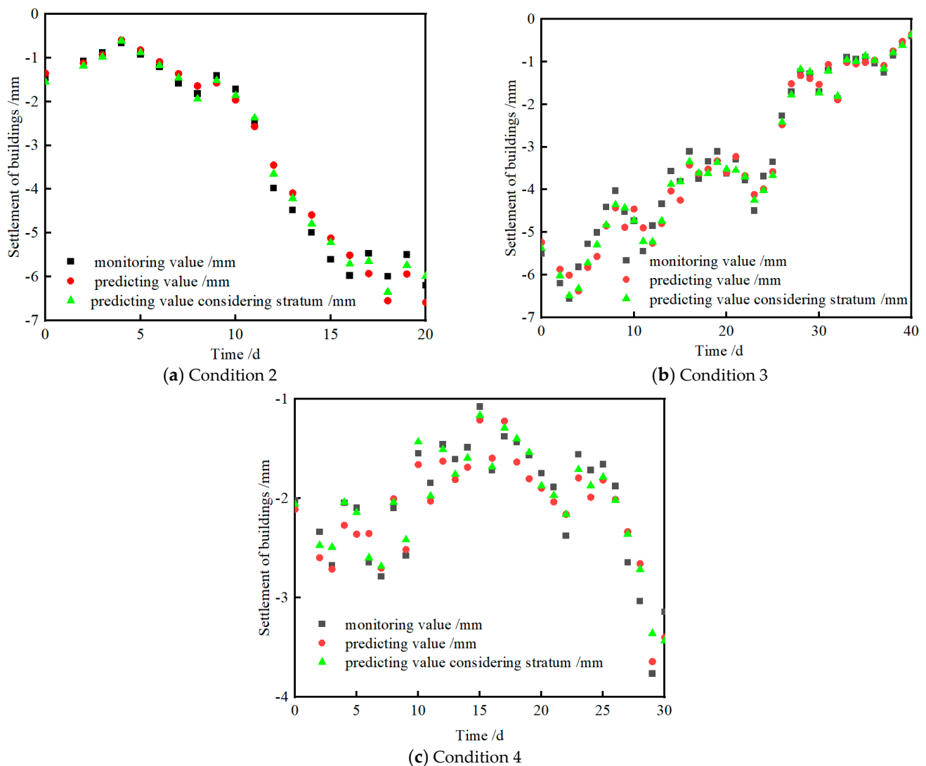
Figure 8. Predicted settlements with and without consideration of soil parameters.
