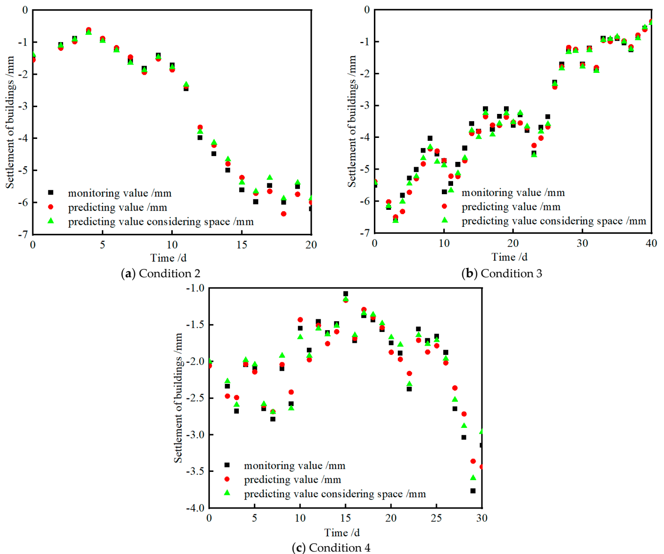
Figure 9. Settlement prediction considering spatial parameters under various working conditions.
