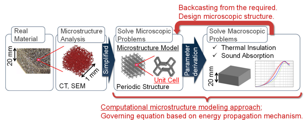
Figure 1. Development of high-performance multifunctional materials via materials model-based research.
