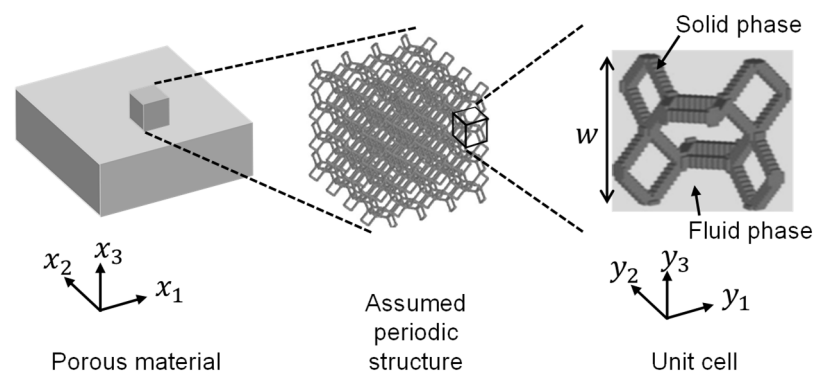
Figure 2. Schematic diagram of homogenization of sound-absorbing poroelastic material.
