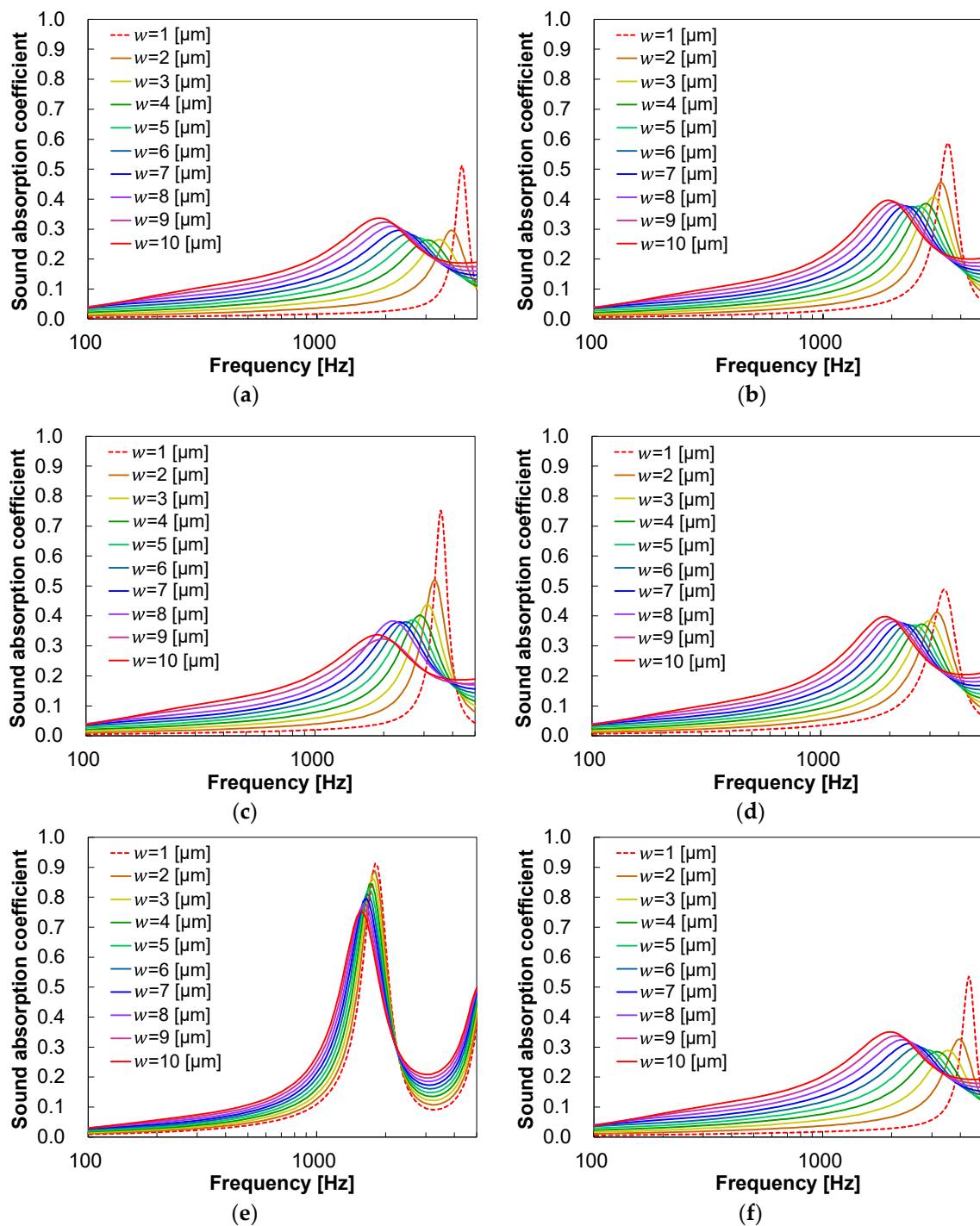
Figure 7. Spectra of predicted sound absorption coefficients of simulated porous material: (a) glass; (b) rubber 1; (c) rubber 2; (d) rubber 3; (e) rubber 4; and (f) rubber 5.
