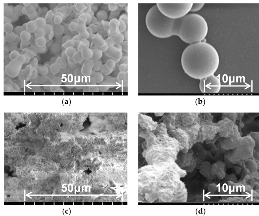
Figure 10. SEM images of synthesized PMS xerogels: (a) original PMS xerogel; (b) original PMS xerogel; (c) hydrophobic CNF-PMS xerogel; (d) hydrophobic CNF-PMS xerogel.
