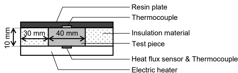
Figure 5. Simple thermal conductivity measurement apparatus.
