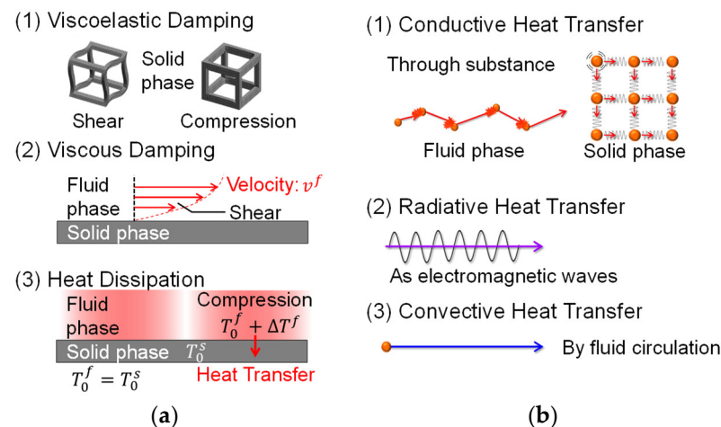
Figure 4. Mechanisms inside porous materials: (a) sound absorption and (b) heat transfer.
