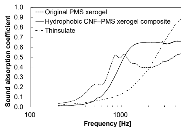
Figure 11. Measured normal-incidence sound absorption coefficients of synthesized PMS xerogels.
