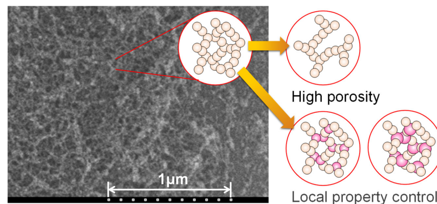
Figure 8. Scanning electron microscopy image of poly(methylsiloxane) (PMS) xerogel.
