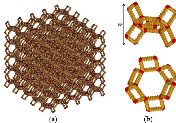
Figure 6. Calculation model of the microstructure of simulated porous material: (a) periodic structure and (b) unit cell.
