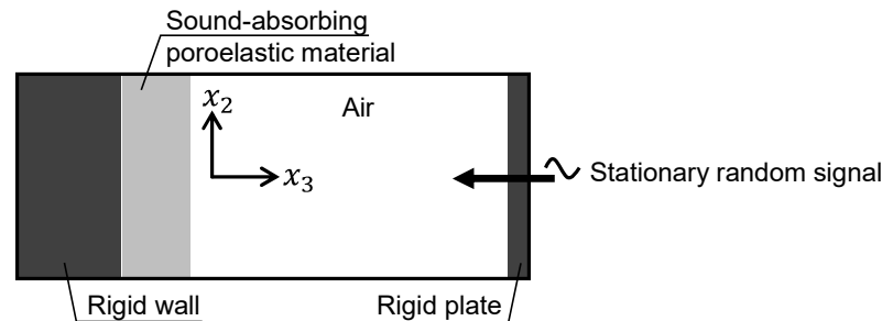
Figure 3. Acoustic tube model for calculating sound absorption coefficients at normal incidence.
