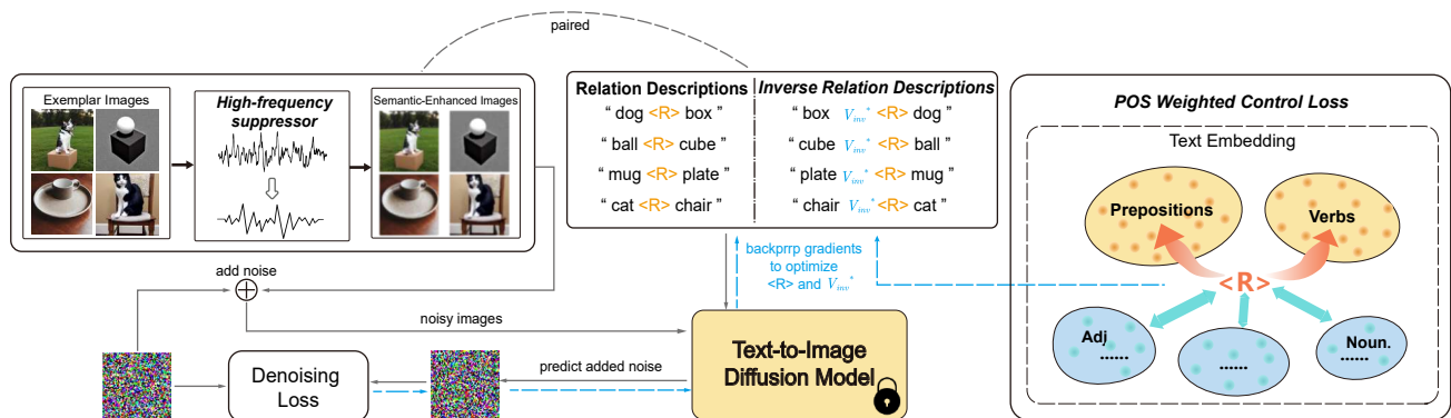
Figure 2. Inv-ReVersion framework : This framework processes exemplar images with a high-frequency suppressor to obtain semantically enhanced images. These images are then input to the model along with text prompts that have undergone inverse relation text expansion. The optimization process of the feature vector is steered by both denoising loss and part-of-speech weighted contrastive loss. In the inference phase, the optimized feature vector can be used as a new word in the text prompt to guide the model in generating images with specific relation concepts.
