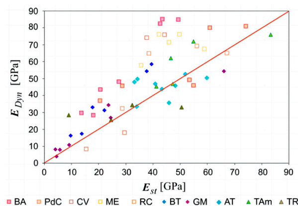
Figure 4. Relationship between E_d and E_s in the studied specimens. The straight line corresponds to the ideal ratio E_d/E_s = 1 [32].
