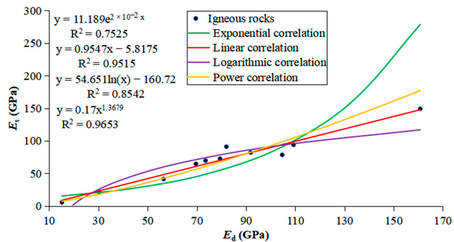
Figure 9. Relationship between different curve fits of dynamic and static elastic moduli of igneous rocks.
