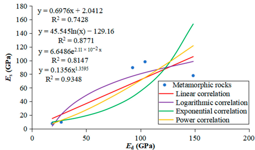
Figure 10. Relationship between different curve fits of dynamic and static elastic moduli of metamorphic rocks.
