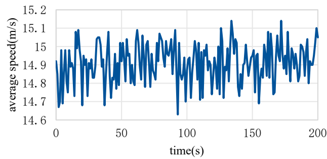
(a) Average speed of traffic flow
