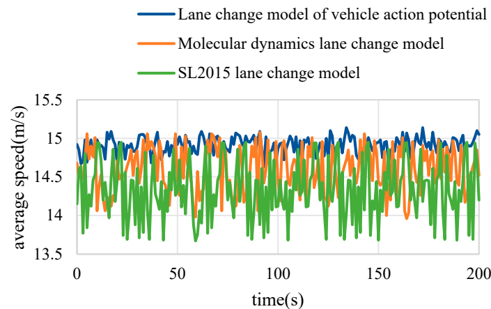
Figure 15. Comparison of average speeds of different models.
