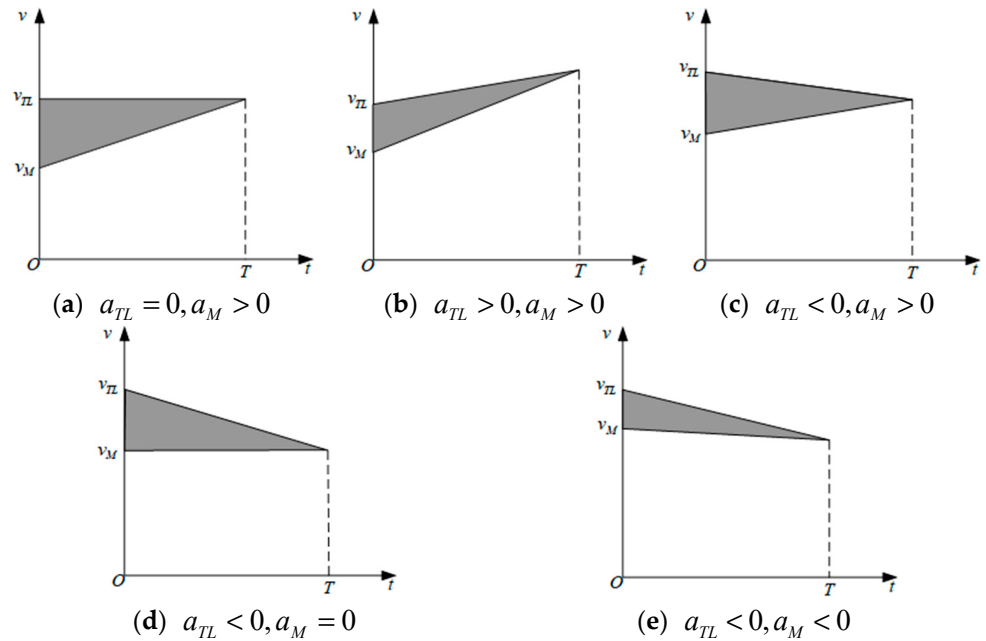
Figure 6. Safe critical time of lane changing under different motion states.
