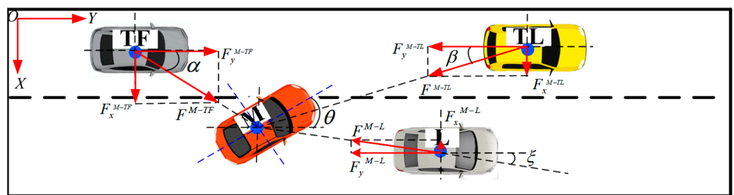
Figure 9. Force analysis of lane changing vehicle M.
