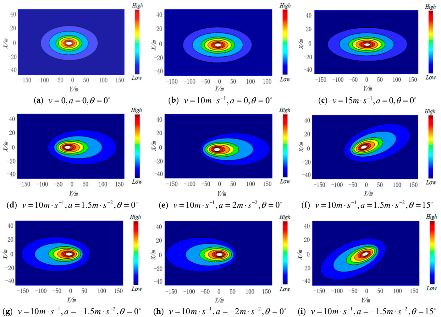
Figure 3. Distribution diagram of vehicle potential field under different motion states.
