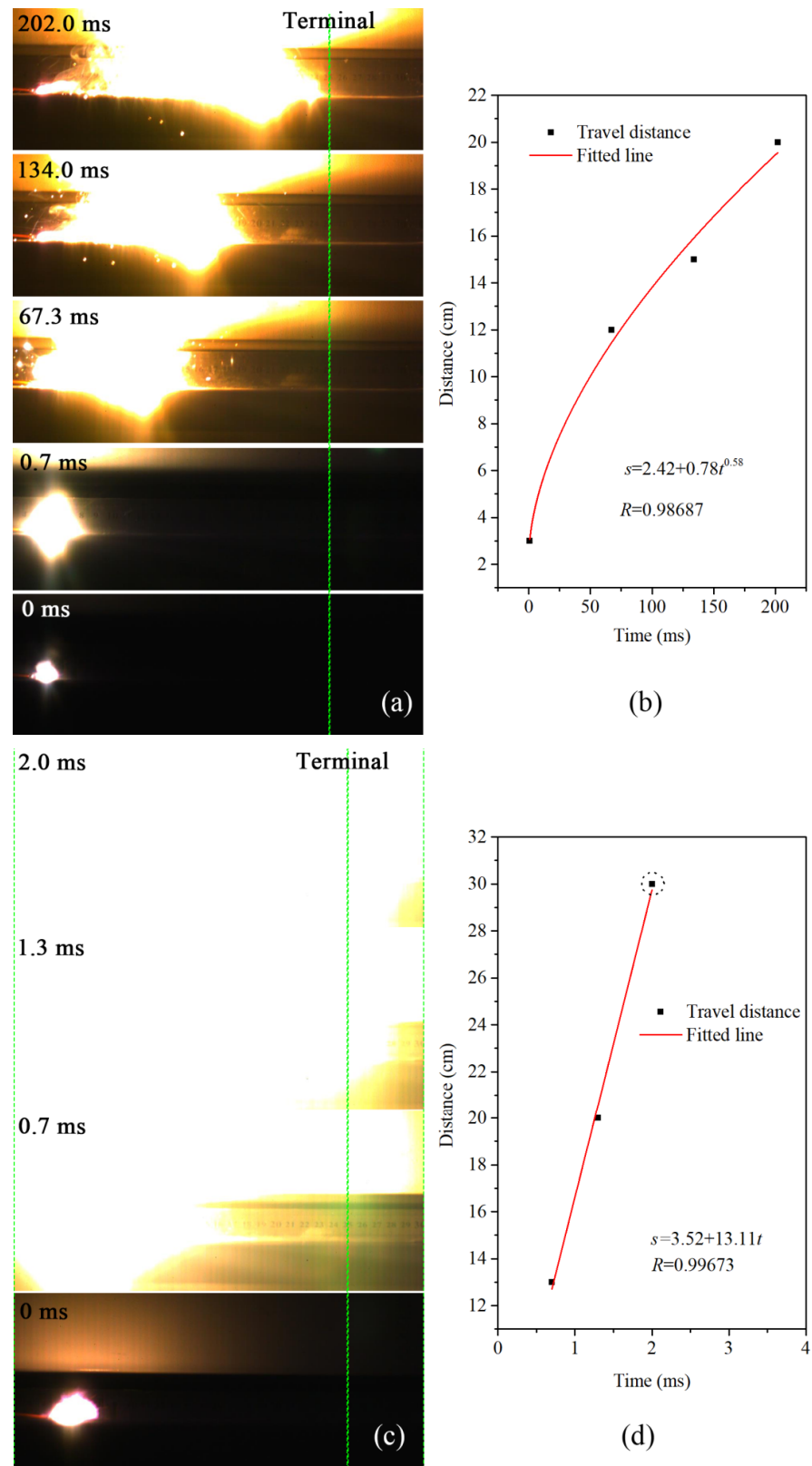
Figure 9. Combustion history of (a) Al/MoO 3 -M and (c) Al/MoO 3 -E in an open environment, and their corresponding travel distance vs. time relations: (b) Al/MoO 3 -M; (d) Al/MoO 3 -E. (The green dot lines in (a,c) indicate the ends of the samples).
