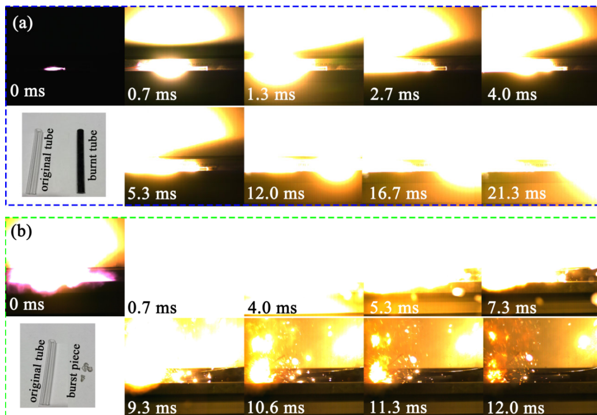
Figure 8. Combustion performance of (a) Al/MoO 3 -M and (b) Al/MoO 3 -E under confined conditions ((a,b) are the comparison of the tube conditions before and after the combustion of Al/MoO 3 -M and Al/MoO 3 -E, respectively).
