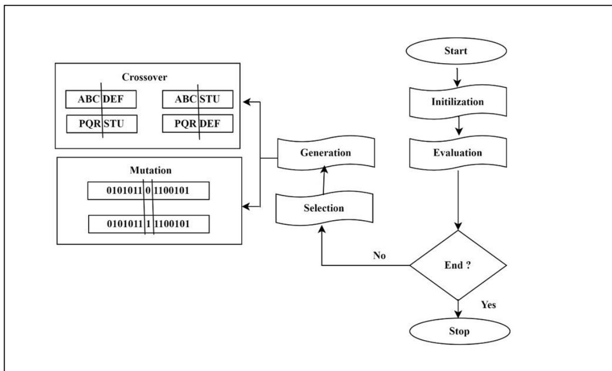
Figure 2. A fundamental operational premise of a genetic algorithm.
