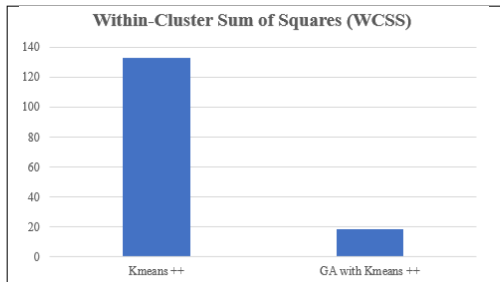
Figure 6. Graph showing the WCSS metrics for Kmeans ++ and GA-KMeans++.
