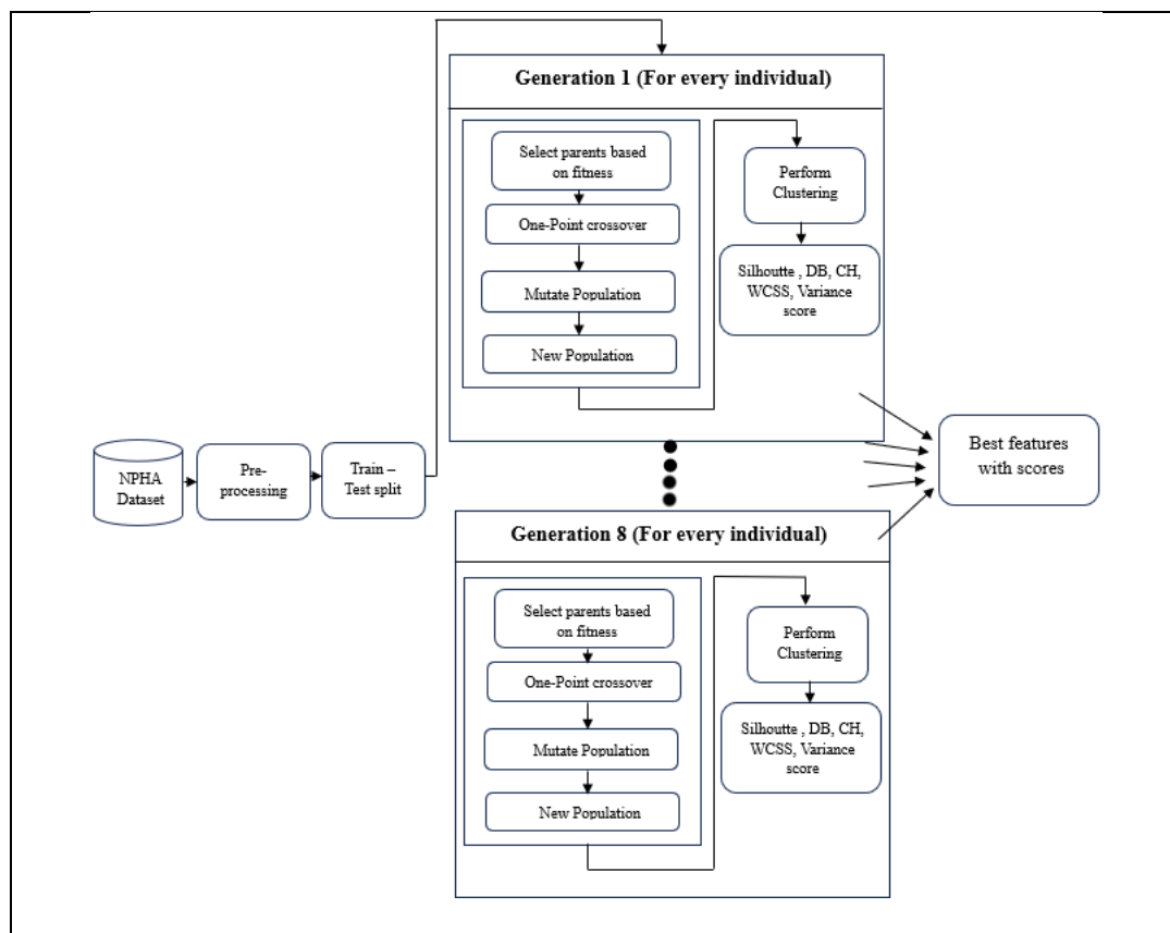
Figure 3. Workflow of the proposed model.
