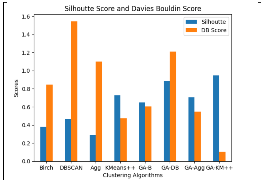
Figure 4. Graph displaying the silhouette scores and Davies–Bouldin scores for all clustering algorithms.
