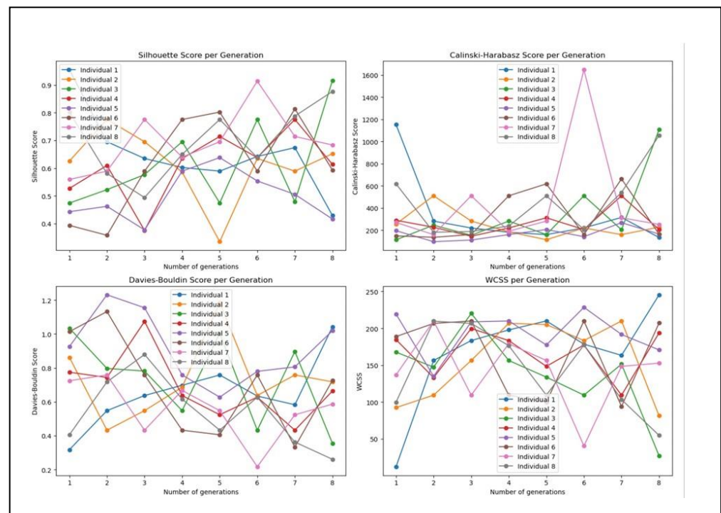
Figure 7. Graph representing the score of GA-KMeans ++ clustering for 8 generations.
