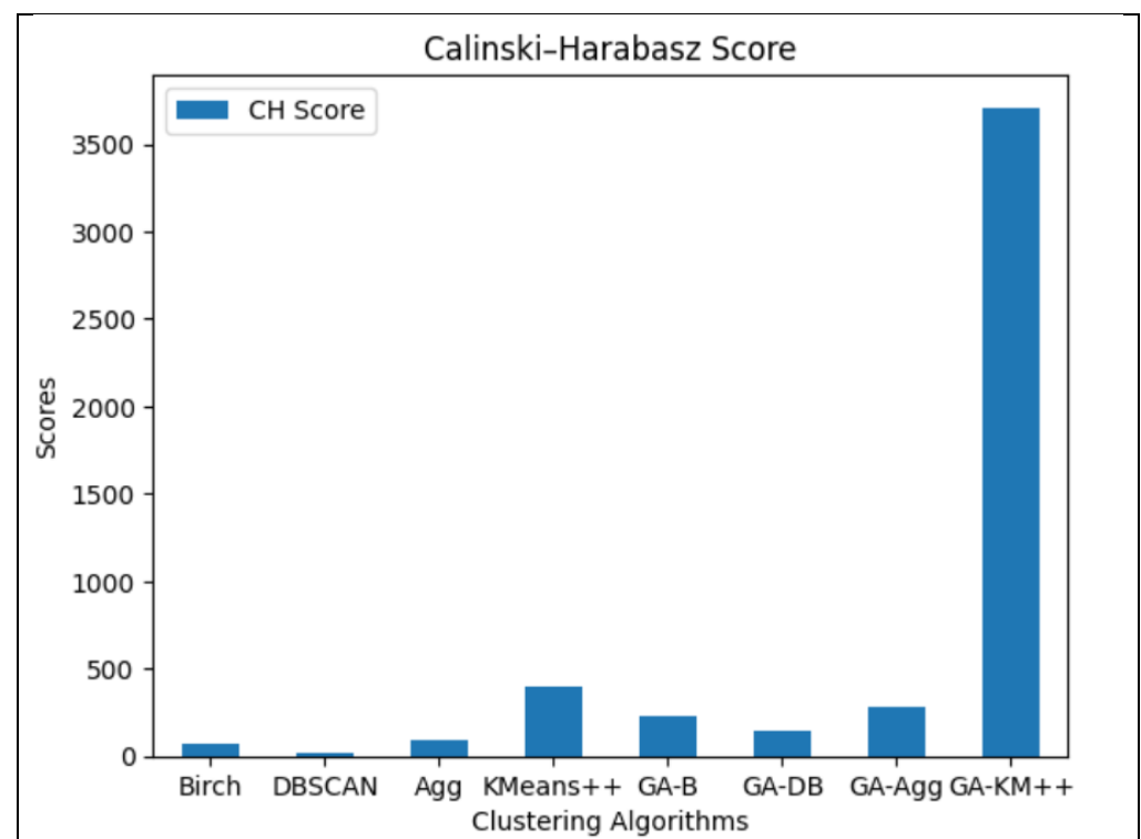
Figure 5. Graph displaying the Calinski–Harabasz scores for all clustering algorithms.
