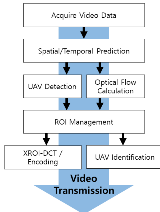
Figure 1. Operation flow diagram of the proposed system.
