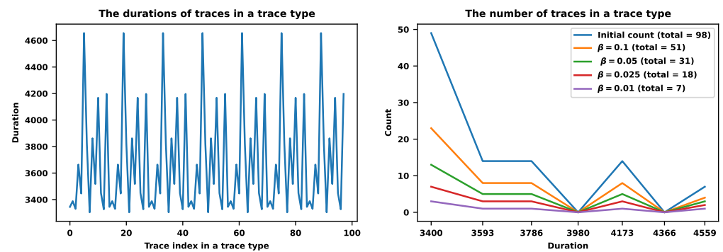
Figure 9. The hybrid approach for a specific trace type (N17 in Figure 10). The left figure shows the plot of durations. The right figure shows the counts of traces for \alpha = \beta .
