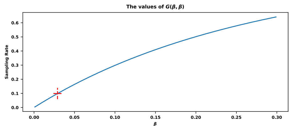
Figure 11. The sampling rates corresponding to different values \alpha = \beta . The red cross corresponds to 10% with \beta = 0.03 .
