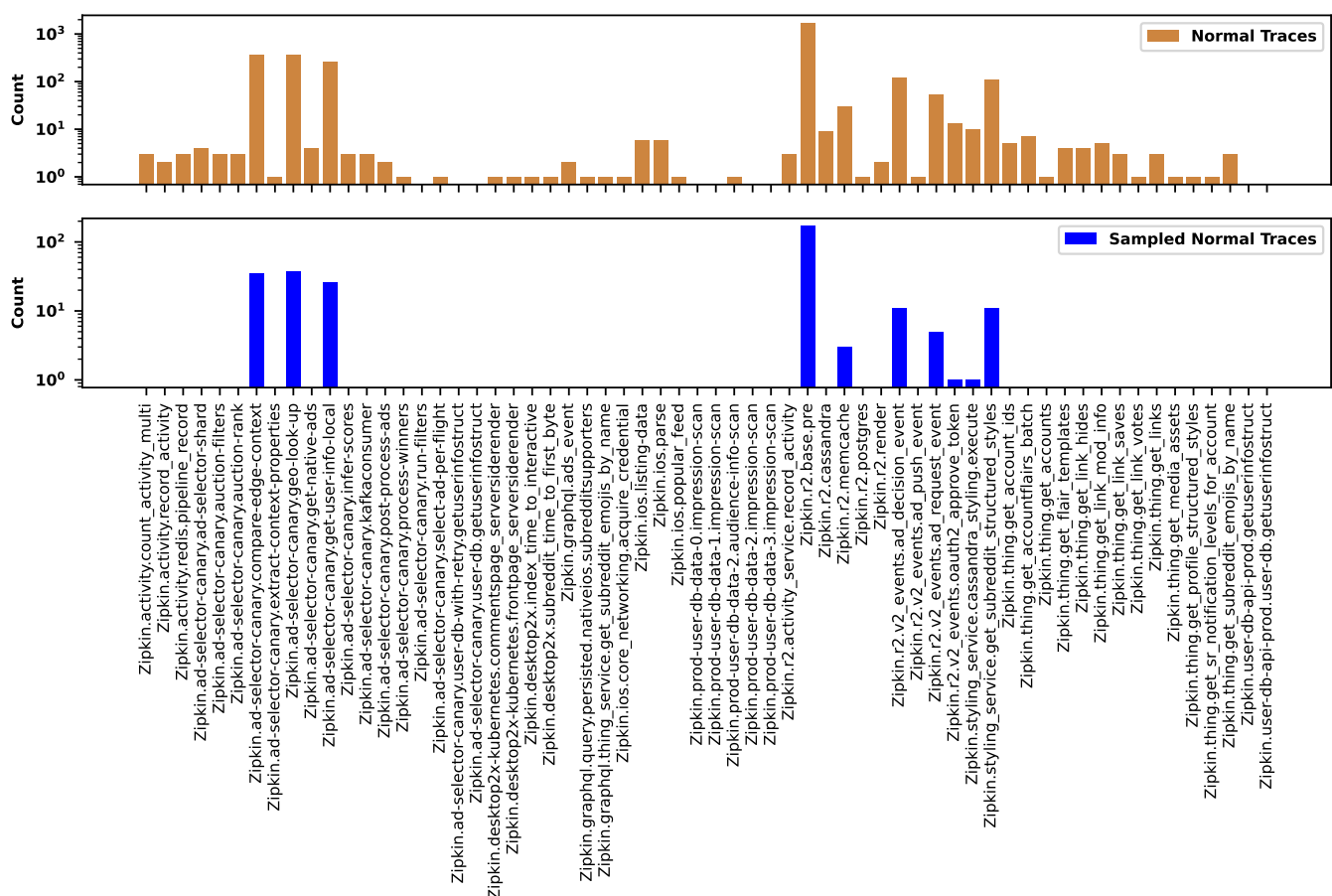
Figure 17. The distribution of normal traces across the types before and after the sampling.
