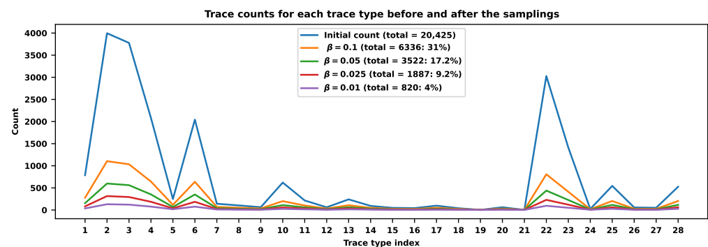
Figure 10. The hybrid sampling approach for \alpha = \beta .
