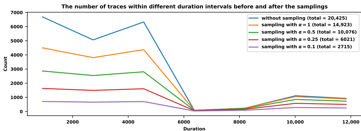
Figure 6. The sampling of traces of Figure 5 for different values of the parameter \beta .
