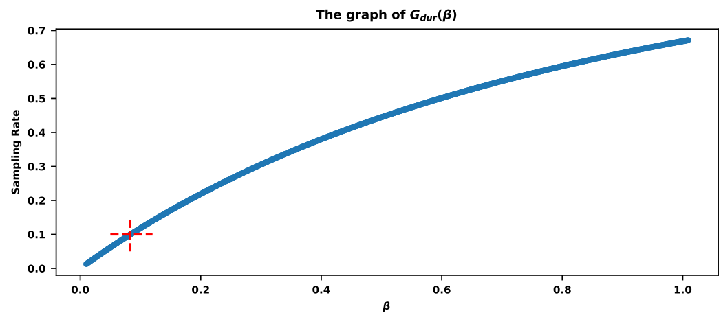
Figure 7. The values of G_{dur}(\beta) show the sampling rates for the different parameter values \beta . The red cross corresponds to \beta = 0.083 with a total sampling rate of 0.0996 (around 10%).
