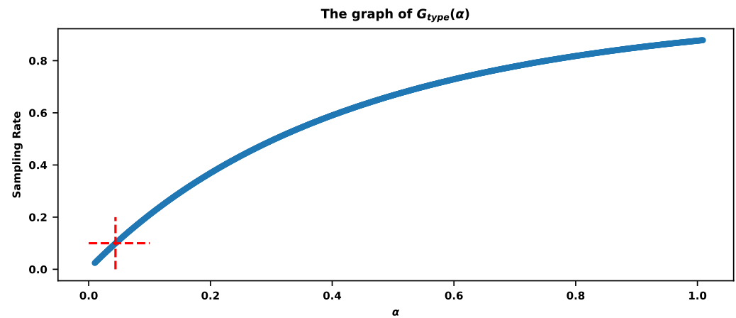
Figure 4. The values of G_{type}(\alpha) show the final sampling rates for different \alpha . The red-cross corresponds to \alpha = 0.044 with the final sampling rate r = 0.099 (around 10%).
