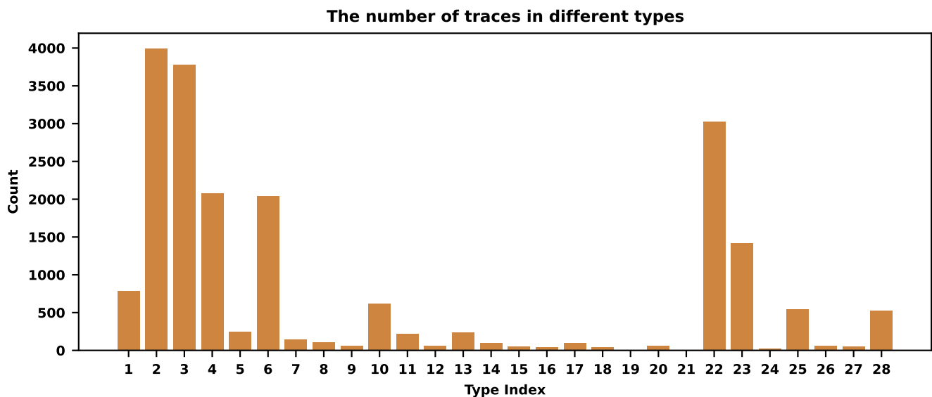
Figure 2. The distribution of traces across different types for a specific application.
