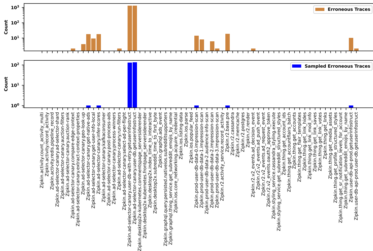
Figure 18. The distribution of erroneous traces across the types before and after the sampling.
