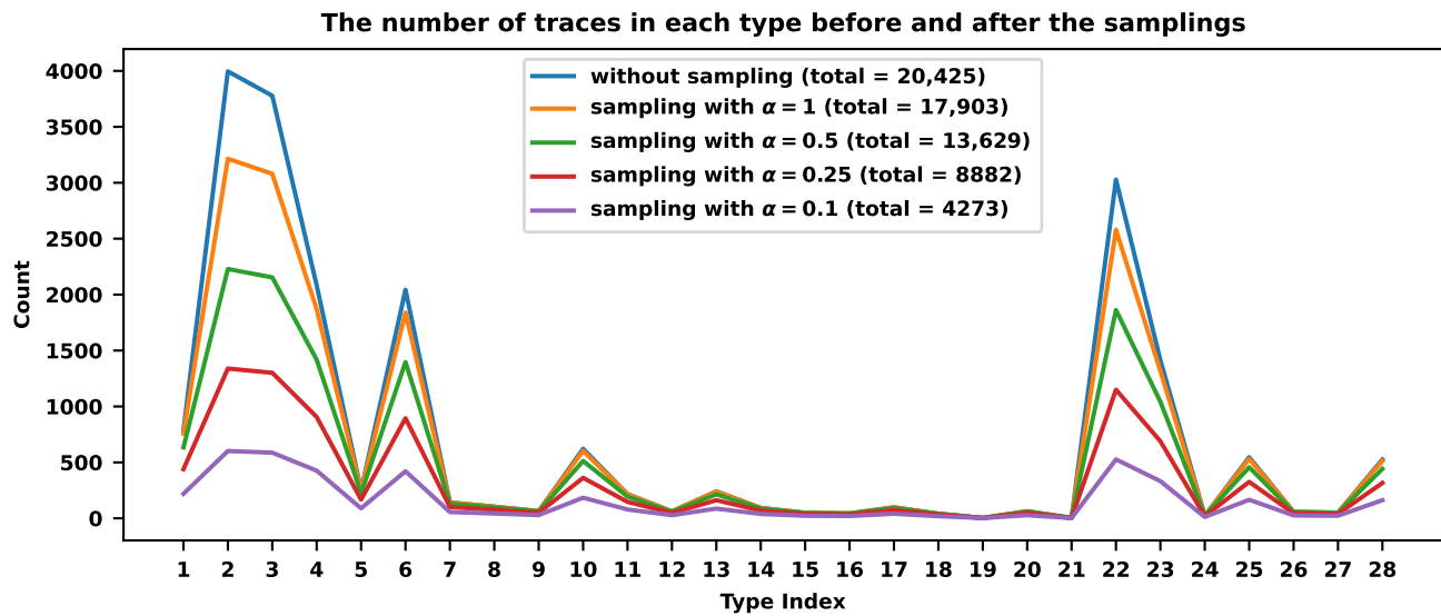
Figure 3. The sampling of traces of Figure 2 for different values of the parameter \alpha .
