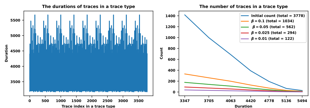
Figure 8. The hybrid approach for a specific trace type (N2 in Figure 10). The left figure shows the plot of durations. The right figure shows the counts of traces in different bins before and after sampling corresponding to different values of \alpha = \beta .
