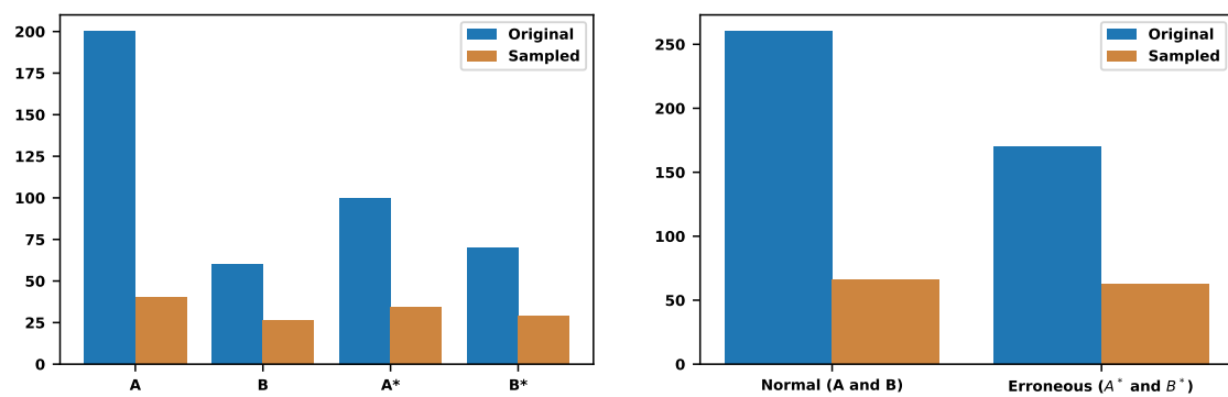
Figure 14. The sampling of two trace types also counts the errors.
