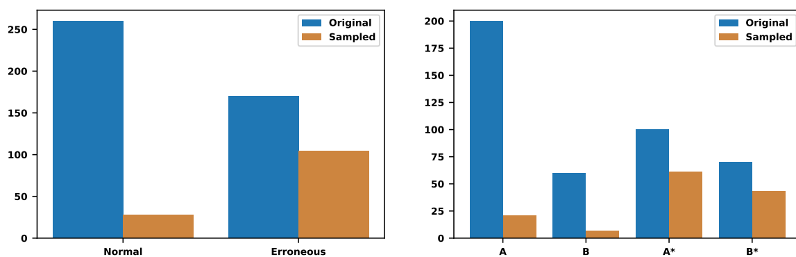
Figure 15. The sampling of two trace types with stricter requirements on the percentage of erroneous traces. Now, we preserve 10% of normal traces and 60% of erroneous ones. The final sampling rate is 30%.
