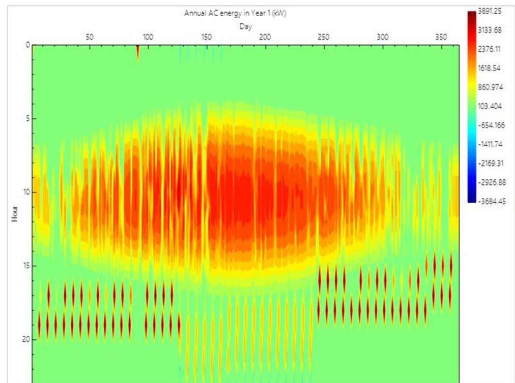
Figure 6. Annual AC energy in Year 1 (kW).
