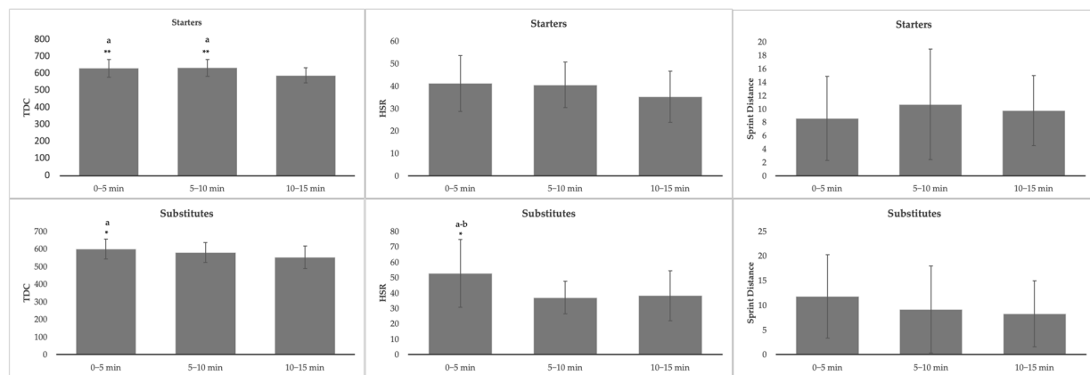
Figure 2. Comparison of 5-Min periods within starters and within substitutes. TDC = total distance covered (meters); HSR = distance covered between 19.8 and 25.2 km·h −1 ; sprint distance = distance covered above 25.2 km·h −1 . a = different from 10–15 period; b = different from 5–10 period. * p < 0.05 ; ** p \leq 0.01 .
