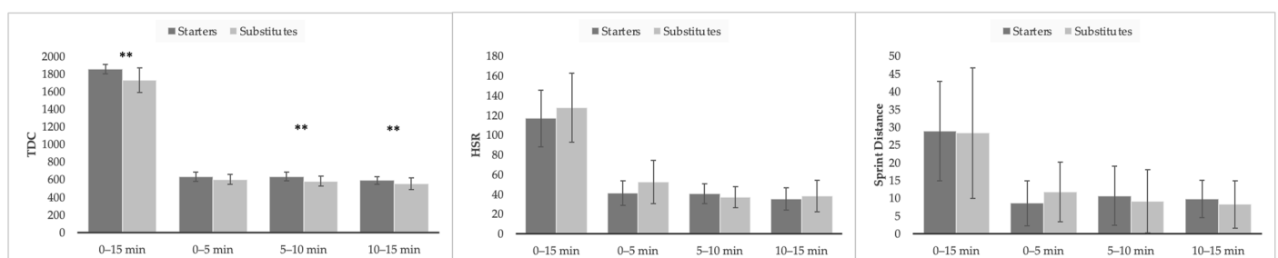
Figure 1. Comparison of the different periods when participating as starters vs. as substitutes. TDC = total distance covered; HSR = distance covered between 19.8 and 25.2 km·h −1 ; sprint distance = distance covered above 25.2 km·h −1 . ** p \leq 0.01 .
