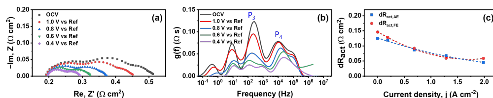
Figure 5. Determination of the charge-transfer coefficients \alpha_{an} and \alpha_{cat} : (a) EIS spectra measured at various cell voltages ( V = 0.4, 0.6, 0.8, 1.0 V, and OCV) under P_{H_2,FE}/P_{ref} = 1 atm and P_{O_2,AE}/P_{ref} = 1 atm, and at T = 700 °C; (b) corresponding DRTs; (c) dR_{act,AE} and dR_{act,FE} [ \Omega \cdot cm^2 ] plotted against current density j , along with corresponding second-order polynomial fits.
