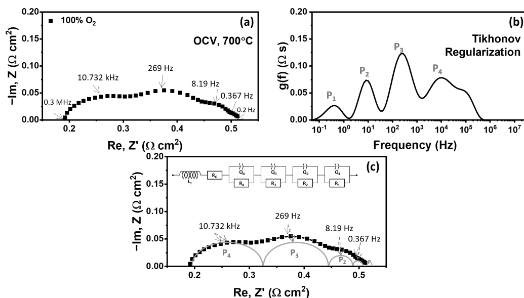
Figure 2. (a) Impedance spectrum measured at 700 °C, 100% H 2 , and 100% O 2 at OCV, with peak frequencies identified from the DRT spectrum; (b) the corresponding DRT showing four resolved processes; and (c) EIS fit using the ECM constructed from the DRT assignments.
