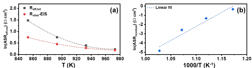
Figure 7. (a) Area-specific ohmic and total resistances based on non-idealities, showing the growing discrepancy between effective total resistance and the electrolyte contribution as temperature decreases. (b) Arrhenius plot of the residual non-ideal resistance contribution ( ASR_{\text{residual}}(T) ); the linear fit yields a slope of 30.4357 with R^2 = 0.944 , supporting the chosen \kappa(T) model.
