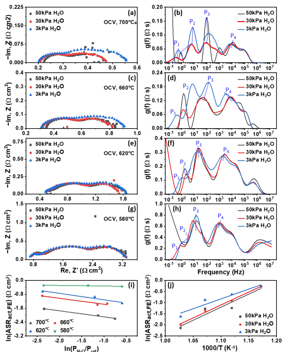
Figure 3. EIS spectra and corresponding DRTs from reversible SOC experiments at 700 °C (a,b), 660 °C (c,d), 620 °C (e,f), and 580 °C (g,h) under controlled vapor fractions P_{\text{H}_2\text{O}}^{\text{FE}}/P_{\text{ref}} = \{0.03, 0.3, 0.5\} and P_{\text{O}_2}^{\text{FE}}/P_{\text{ref}} = \{0.21\} . (i) Determination of parameter ‘b’. \ln \text{ASR}_{\text{act,FE}} [\Omega \cdot \text{cm}^2] as a function of vapor partial pressures obtained from OCV values, \ln(P_{\text{H}_2\text{O}}^{\text{FE}}/P_{\text{ref}}) . (j) Determination of the fuel-electrode activation energy E_{\text{act,FE}} in Equation (15).
