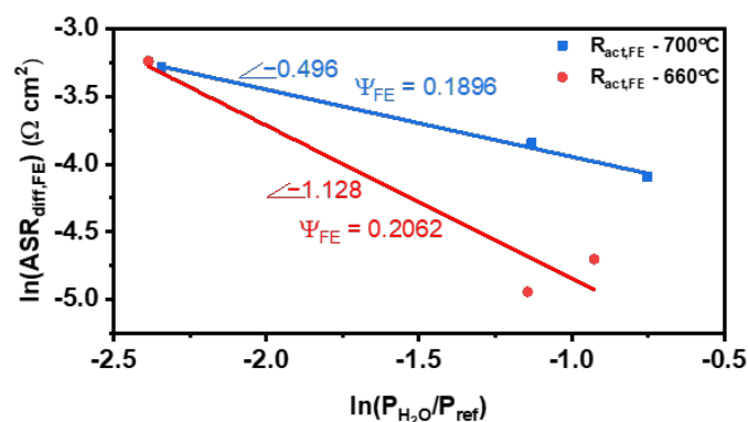
Figure 8. Fuel-electrode diffusion resistance from EIS regression: ASR_{\text{diff,FE}} at 660 and 700 °C, 50, 30, and 3 kPa \text{H}_2\text{O} and 21% \text{O}_2 .
