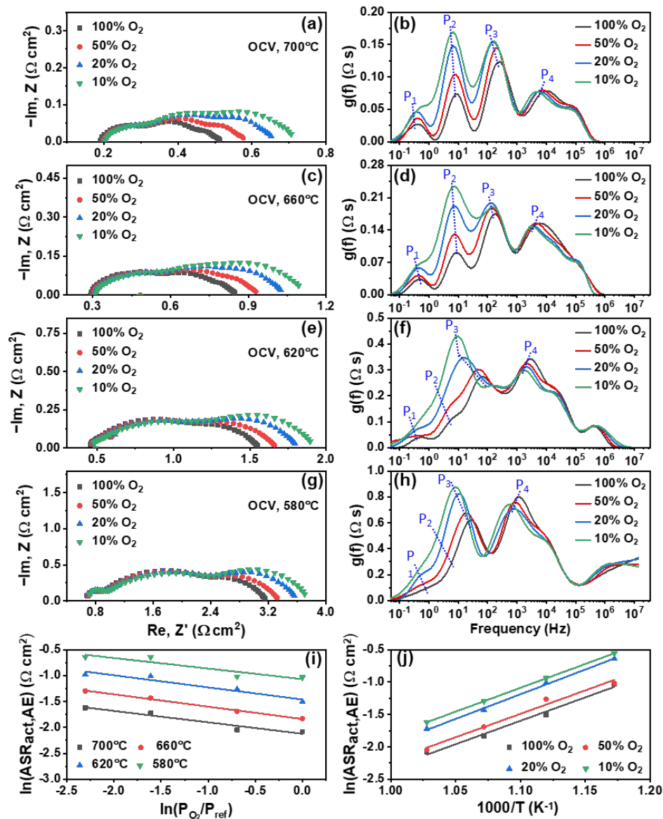
Figure 4. EIS spectra and corresponding DRTs from SOFC experiments at 700 °C (a,b), 660 °C (c,d), 620 °C (e,f), and 580 °C (g,h) for P_{O_2}^{AE}/P_{ref} = \{0.1, 0.2, 0.5, 1\} and P_{H_2}^{AE}/P_{ref} = \{1\} . (i) Determination of parameter 'm' at different oxygen concentrations ( P_{O_2}^{AE}/P_{ref} = 0.1, 0.2, 0.5, 1 ). (j) Determination of the air-electrode activation energy E_{act,AE} , based on DRT peak shifts extracted from the EIS spectra.
