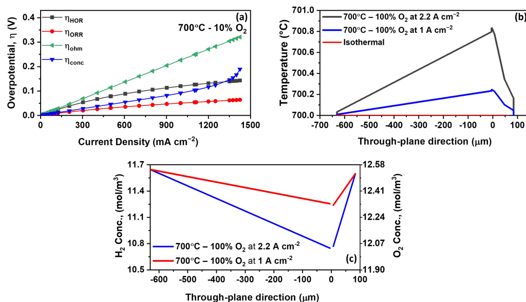
Figure 10. (a) The individual overpotential contributions under SOFC operation, namely, the ohmic overpotential \eta_{ohm} , the activation overpotential \eta_{act} , and the concentration (gas diffusion) overpotential \eta_{conc} , are shown as functions of current density j . The operating conditions were 100% \text{H}_2 (dry) and 10% \text{O}_2 at T = 700^\circ\text{C} . (b) Temperature distribution within the cell. (c) Concentration distribution within the cell.
