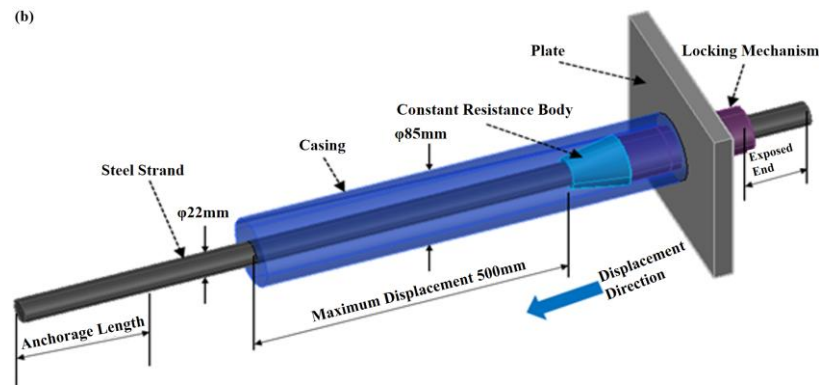
Figure 2. Schematic of constant-resistance large-deformation anchor cable structure: (a) schematic; (b) structural diagram.
