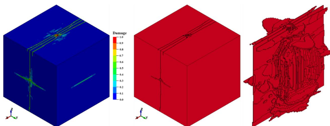
Figure 11. Crack evolution.
