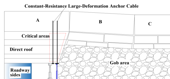
Figure 8. Position of constant-resistance large-deformation anchor cable support.
