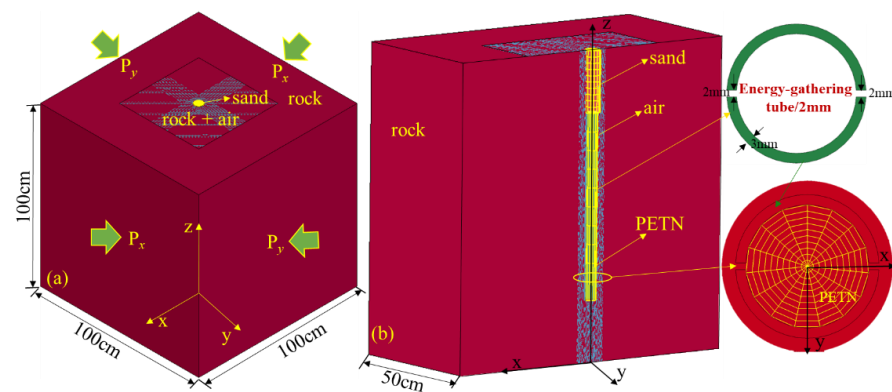
Figure 4. Modeling of concentrated-energy blasting.
