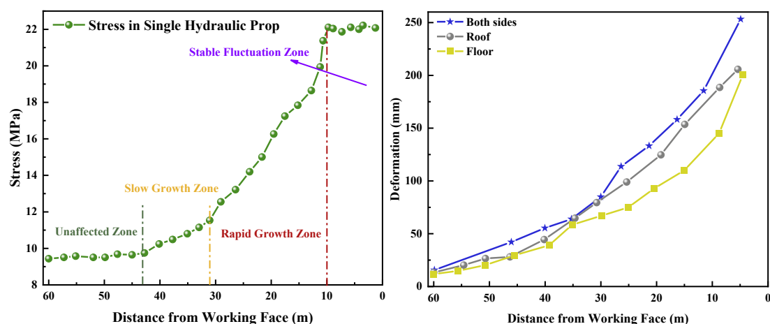
Figure 22. Rock pressure manifestation characteristics during the reuse period: (a) individual pressure; (b) rock mass deformation.
