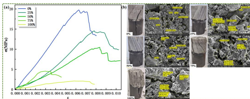
Figure 5. Mechanical properties and microstructural changes diagram: (a) stress–strain curve; (b) failure mode of coal–rock assembly and SEM test results.
