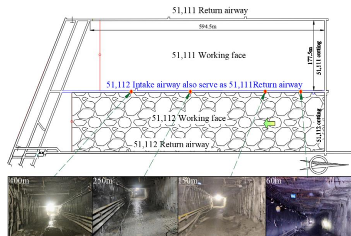
Figure 23. Actual photo of the retained roadway.
