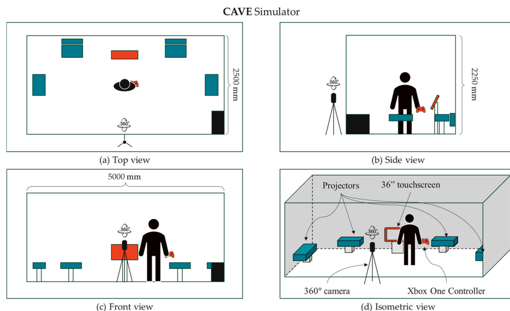
Figure 2. Arrangement of CAVE system (FULmax VR-Hub Wide) from (a) top view, (b) side view, (c) front view and (d) isometric view.
