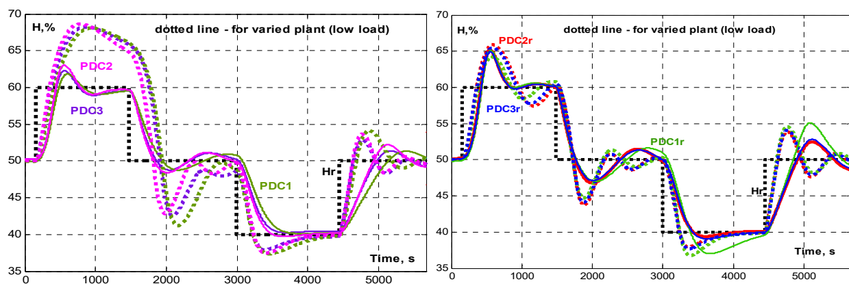
Figure 6. Reference step responses of level of MPDC systems designed for F = \min (left) and F_{rob} = \min (right).
