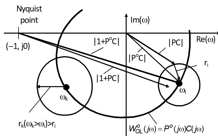
Figure 1. Nyquist plot for plant model's family.
