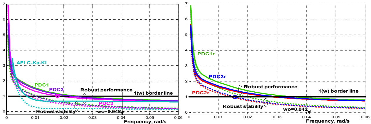
Figure 4. Robust stability and robust performance curves of investigated MPDC and AFLC systems.
