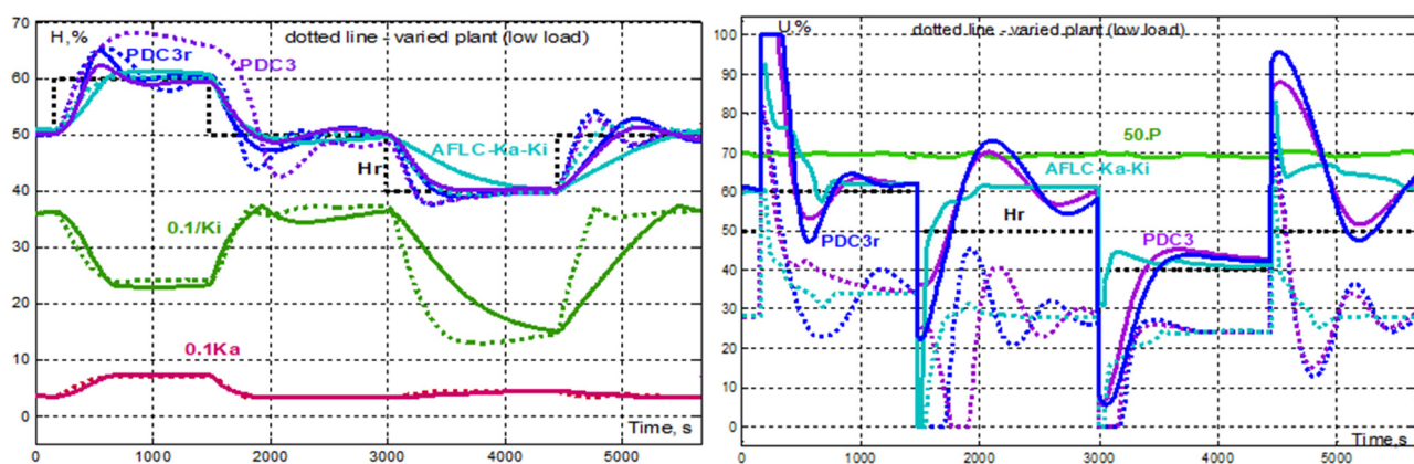
Figure 8. Reference step responses of level (left) and control action (right) of MPDC systems PDC3, PDCr3 and AFLC.
