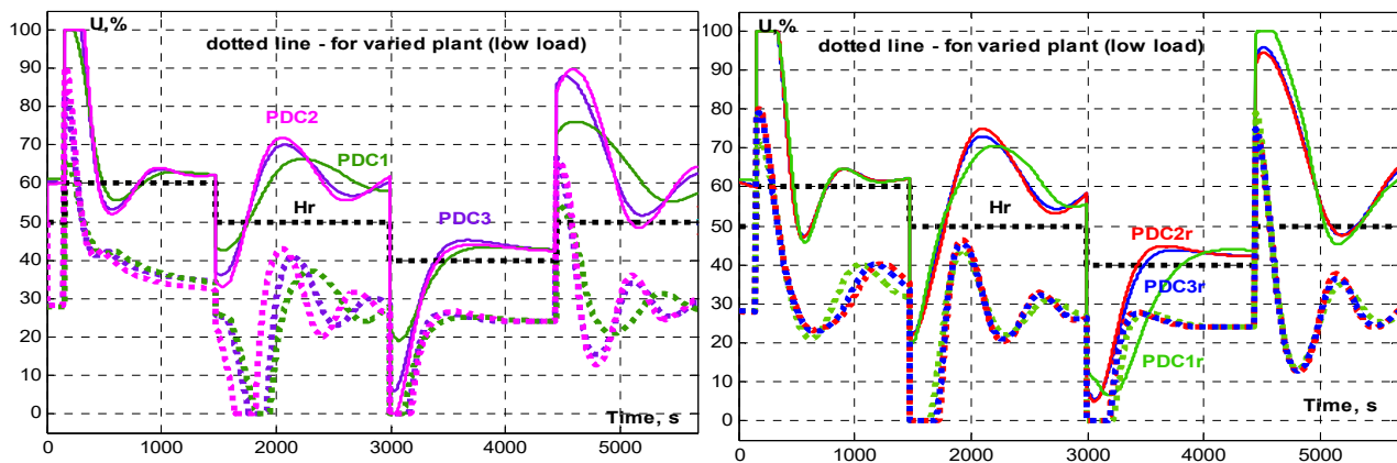
Figure 7. Reference step responses of control action of MPDC systems designed for F = \min (left) and F_{\text{rob}} = \min (right).
