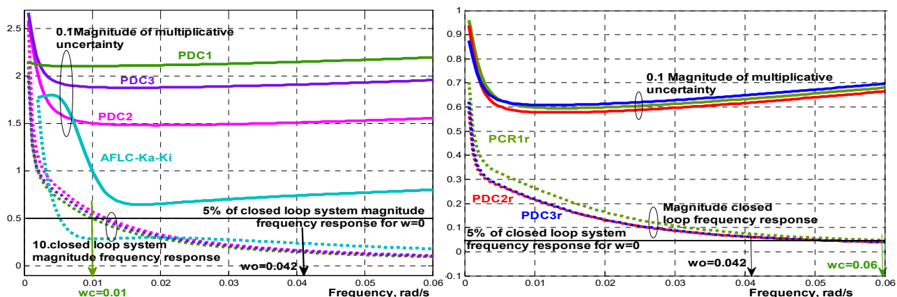
Figure 5. Magnitudes of multiplicative uncertainties and magnitude frequency responses of closed-loop AFLC and MPDC.
