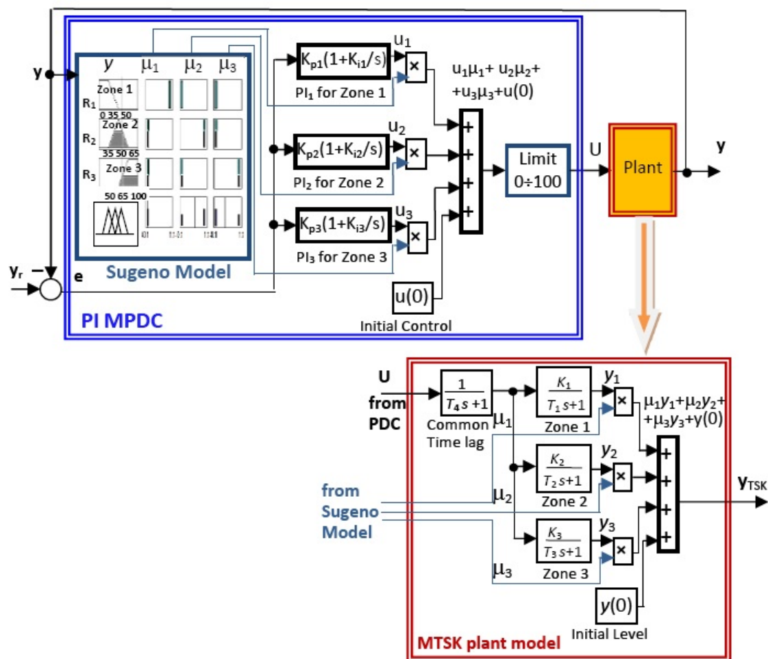
Figure 2. Block diagram of control system MPDC based on MTSK plant model which replaces the plant in simulation.
