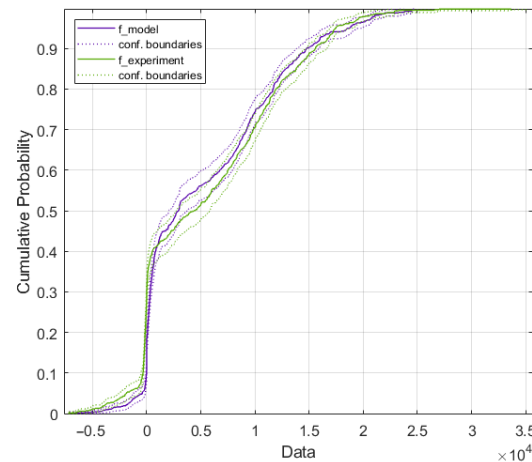
Figure 7. Cumulative probability of the traction force samples.
