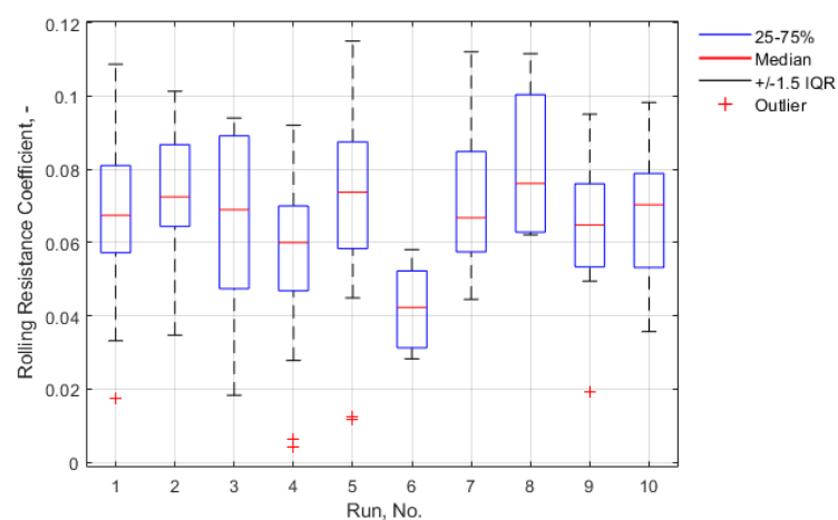
Figure 5. Rolling resistance coefficient values determined through the rolling experiment.
