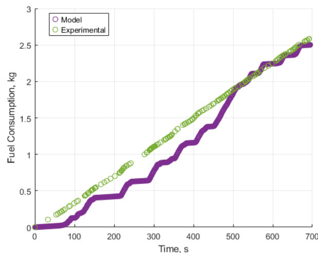
Figure 8. Comparison of Theoretical and Experimental Fuel Consumption.
