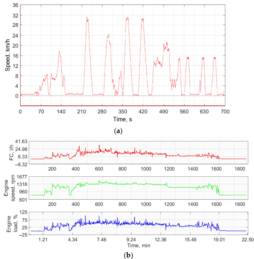
Figure 3. The experimental driving test runs: (a) data logger-recorded drive for the determination of rolling characteristics; (b) engine operating parameters in steady-state mode. TEXA report.
