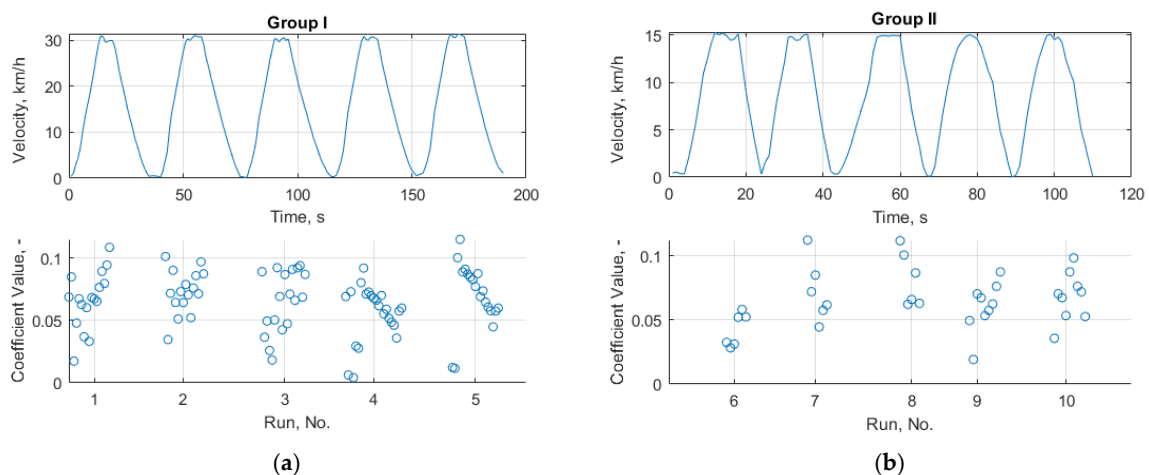
Figure 4. Instantaneous values of rolling resistance determined during the rolling experiment: (a) coasting after reaching 30 km/h; (b) coasting after reaching 15 km/h.
