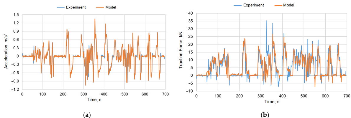
Figure 6. Comparison of Experimental and Simulation Results of Vehicle Movement: (a) Vehicle acceleration during the test; (b) Traction force attainable by the vehicle.
