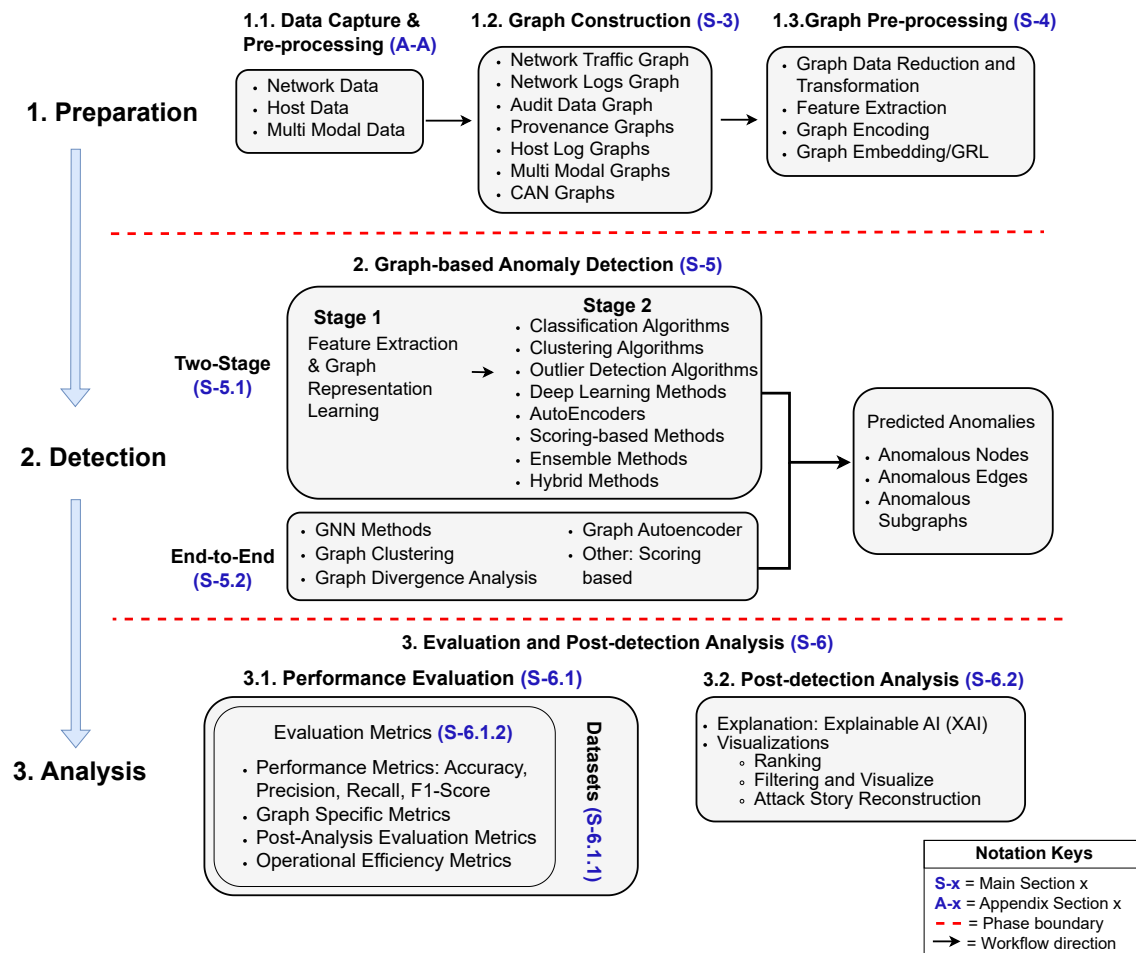
Figure 2. GBAD workflow for intrusion detection. The workflow is organized into three main phases: (1) Preparation—comprising data capture and pre-processing (Section A-A), graph construction (Section 3), and graph pre-processing (Section 4). (2) Detection—applying either two-stage (Section 5.1) or end-to-end (Section 5.2) anomaly detection methods to identify anomalous nodes, edges, or subgraphs. (3) Analysis—including performance evaluation (Section 6.1) and post-detection analysis such as XAI explanations and attack story reconstruction (Section 6.2). Benchmark datasets are summarized in Subsection 6.1.1. The notation key within the figure defines all abbreviations and symbols used.
