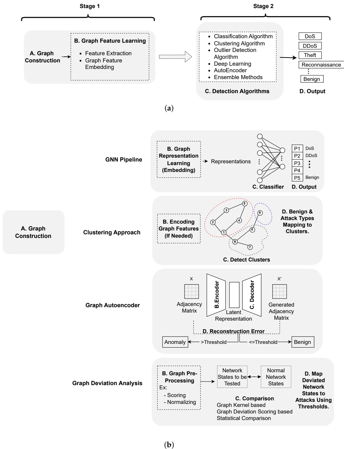
Figure 3. Categories of graph-based anomaly detection for intrusion detection. (a) Two-stage approaches (i.e., first stage includes feature extraction and GRL for embedding; the second stage is anomaly detection). (b) End-to-end approaches for anomaly detection. The labels (A–D) denote the sequential stages of the detection pipeline within each respective approach.
