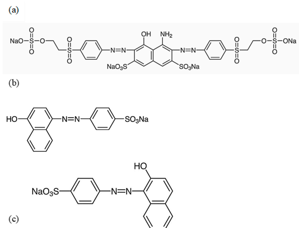
Figure 1. (a) Reactive Black 5, (b) Acid Orange 20 (Orange I), (c) Acid Orange 7 (Orange II).
