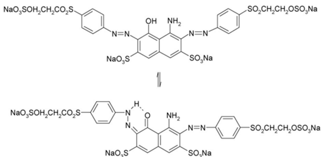
Figure 3. Azo-hydrazone tautomerism of RB5 (analogously for AO7).
