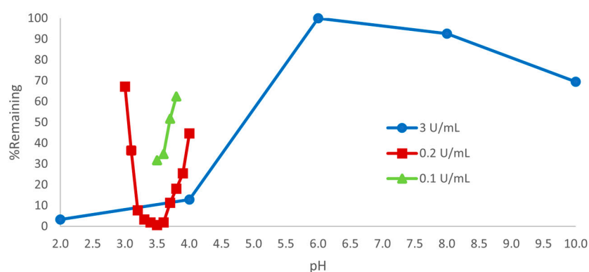
Figure 2. pH optimization of RB5. Reaction conditions: 50 \mu M dye, 1.5 mM \text{H}_2\text{O}_2 , 40 mM buffers for 3 h; analysis by UV-Vis (596 nm) for the wide pH range and by HPLC for narrow ranges. Results presented as mean \pm SD, where error bars represent the SD of triplicate determinations, not visible here because they are smaller than the symbols.
