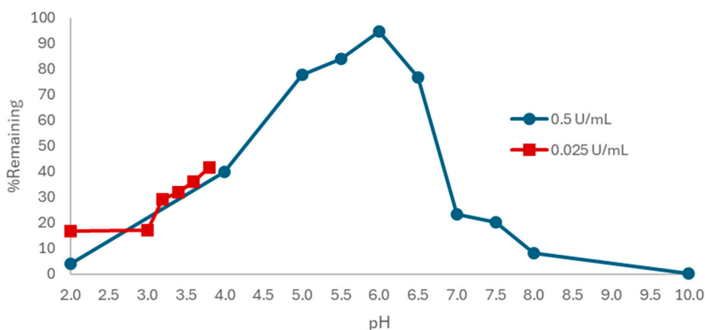
Figure 4. pH optimization of AO7. Reaction conditions: 50 \mu M dye, 1.5 mM \text{H}_2\text{O}_2 , 40 mM buffers for 3 h; analysis by HPLC. Results presented as mean \pm SD of triplicate determinations, error bars not visible because they are smaller than the symbols.
