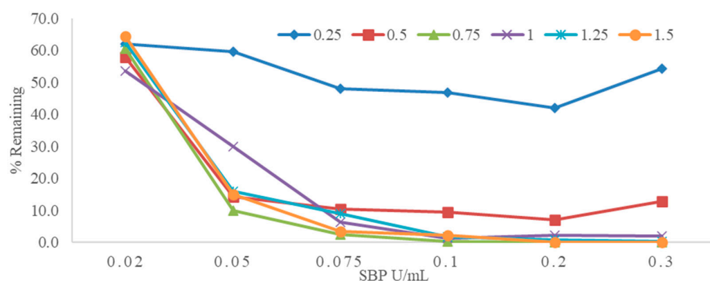
Figure 6. SBP and peroxide optimization for RB5. Reaction conditions: 50 \mu\text{M} dye, 40 mM citrate buffer, pH 3.5, varying concentration of peroxide for 3 h; analysis by HPLC. Numbers in the legend are molar ratios, [peroxide]/[dye]. Results presented as mean \pm SD of triplicate determinations, error bars not visible because they are smaller than the symbols.
