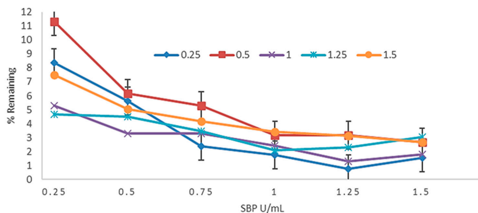
Figure 7. SBP and peroxide optimization for AO7. Reaction conditions: 50 \mu M dye, 40 mM citrate buffer, pH 3.5, varying amount of \text{H}_2\text{O}_2 for 3 h; analysis by HPLC. Numbers in the legend are molar ratios, [peroxide]/[dye]. Triplicate results presented as mean \pm SD, where error bars represent the SD.
