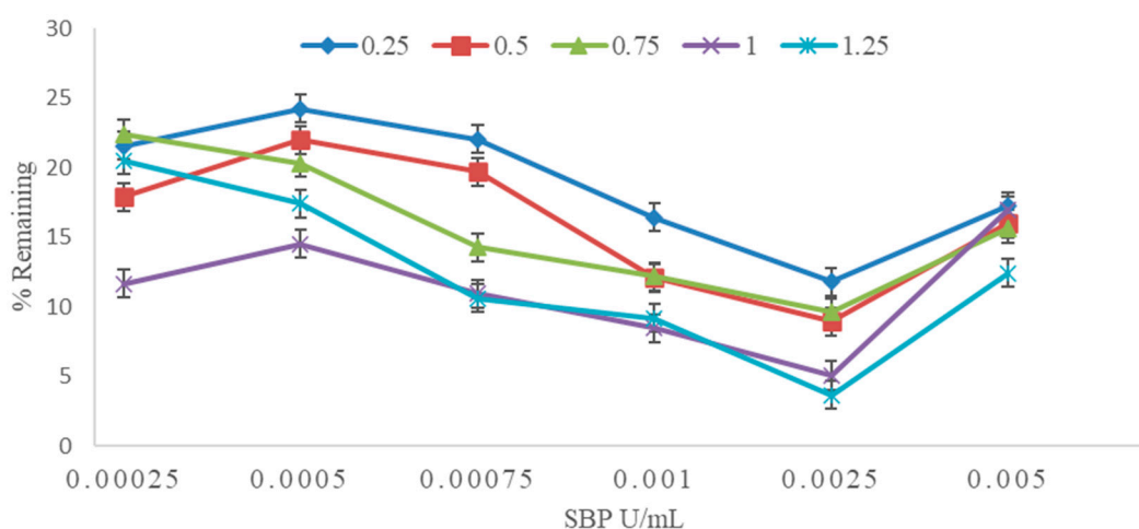
Figure 8. SBP and peroxide optimization for AO20. Reaction conditions: 50 \mu M dye, 40 mM citrate buffer, pH 3.5, varying concentration of \text{H}_2\text{O}_2 for 3 h; analysis by HPLC. Numbers in the legend are molar ratios, [peroxide]/[dye]. Triplicate results presented as mean \pm SD, where error bars represent the SD.
