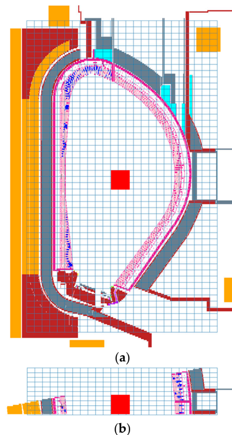
Figure 3. The mesh tally dimensions were used for the neutron spectra distribution. The vertical (a) and horizontal (b) cross-section through the VV midplane.
