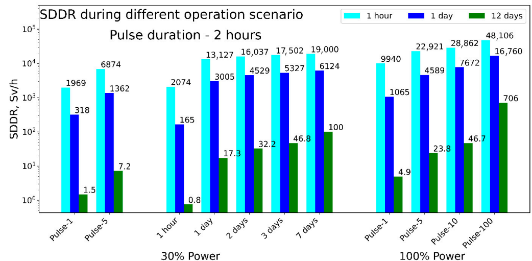
Figure 8. The SDDR after the different irradiation scenarios, for the different cooling times (1 h, 1 day, 12 days).
