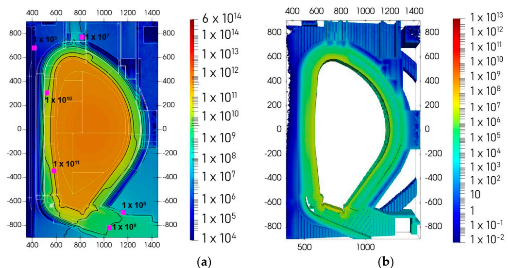
Figure 5. The total neutron flux (a) during the base D–D irradiation, \text{n}\cdot\text{cm}^{-2}\cdot\text{s}^{-1} , and the decay gamma source intensity after 12 days of cooling (b), 1/sec.
