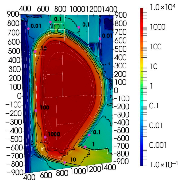
Figure 6. The SDDR in Sv/h after 12 days of cooling, for the D–T Base irradiation scenario with 2000 MW of the fusion power inside the VV of the DEMO tokamak.
