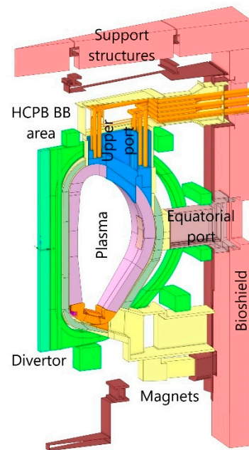
Figure 2. Three-dimensional CAD geometry model: 11°25'—degree DEMO Base model with the HCPB BB concept.
