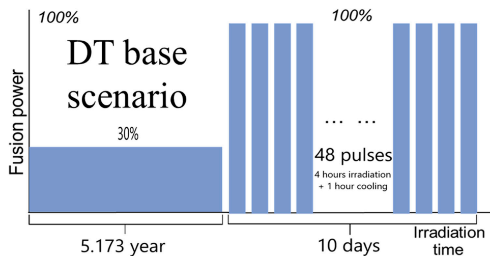
Figure 1. Phase 1 of the DEMO irradiation scenario used for the activation calculations.
