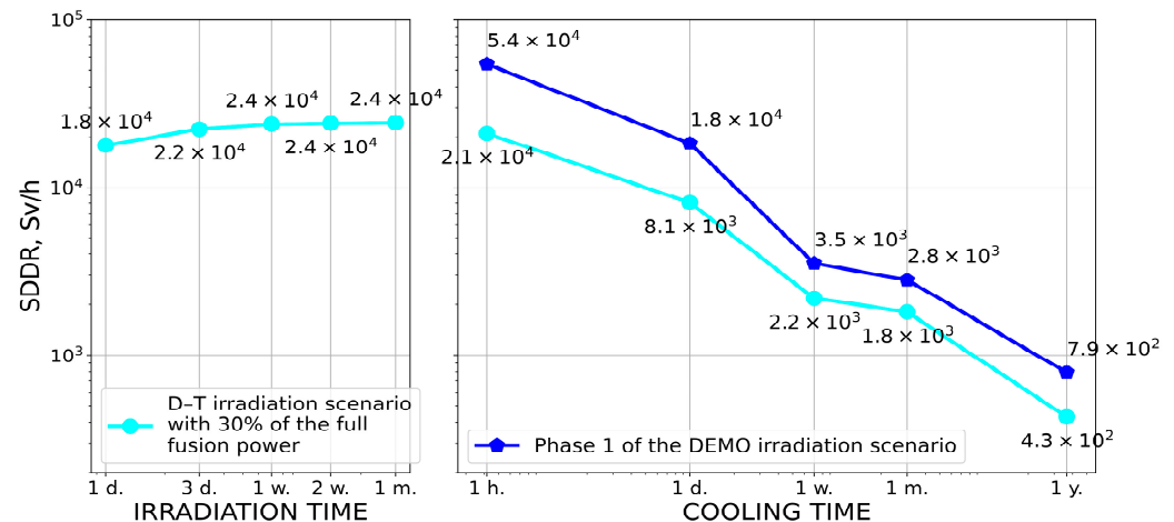
Figure 7. The SDDRs in the centre of the VV, during Phase 1 of the DEMO irradiation scenario with 2000 MW fusion power, and the continuous D-T irradiation scenarios with 30% of the full fusion power.
