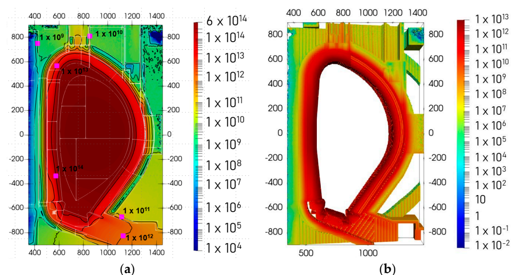
Figure 4. The total neutron flux (a) during the base D–T irradiation, n \cdot \text{cm}^{-2} \cdot \text{s}^{-1} , and the decay gamma source intensity after 12 days of cooling (b), 1/sec.
