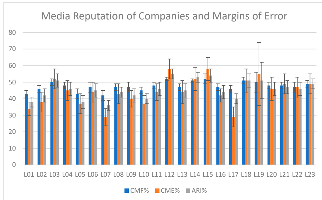
Figure 5. Media reputation of companies and margins of error presented according to different indices using Google API combined with Stanford CoreNLP.
