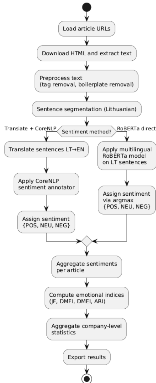
Figure 1. The workflow of the proposed method for determining media reputation.
