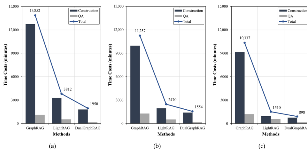
Figure 2. Execution time comparison of graph-based methods across datasets and different stages. (a) NQ; (b) HotpotQA; (c) 2WikiMultihopQA.
