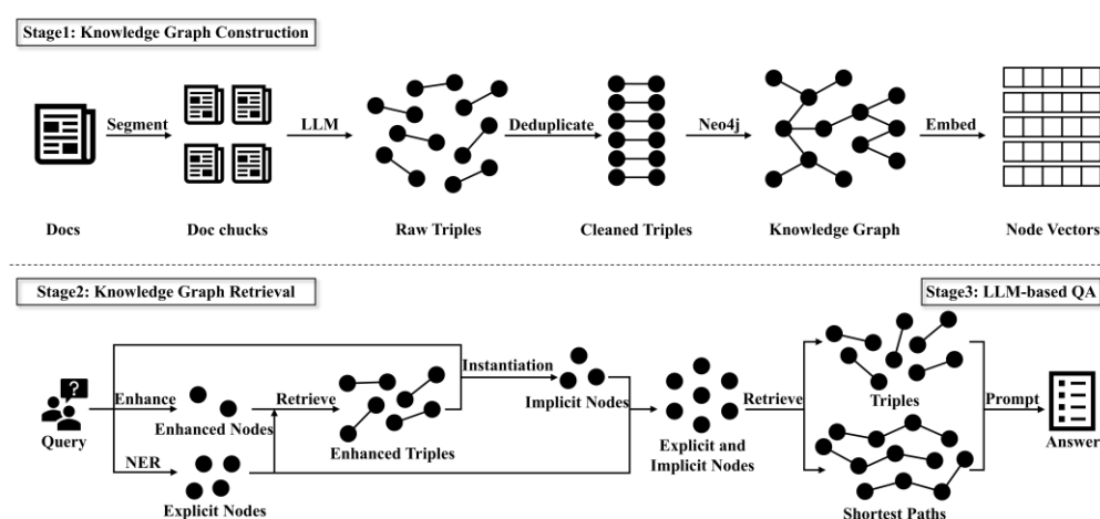
Figure 1. Overview of the DualGraphRAG framework.
