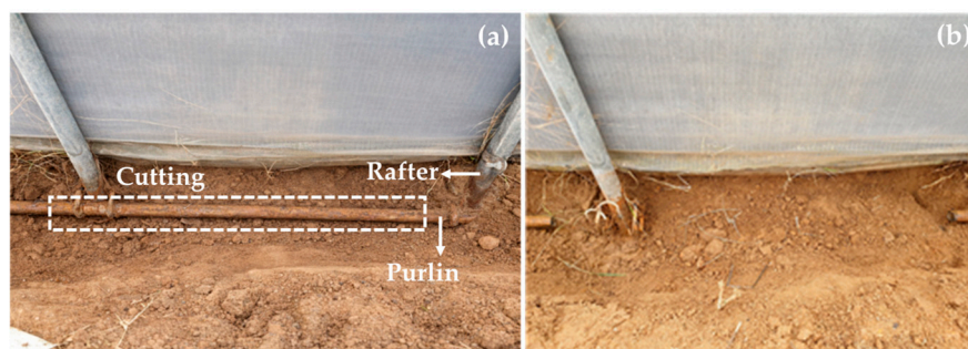
Figure 1. Example of collecting buried rafters or purlins in a greenhouse: (a) rafter and purlin before cutting; (b) section of a purlin after cutting and harvesting from the buried installation.
