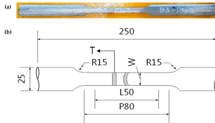
Figure 2. Specimen for tensile test used in this study. (a) Specimen; (b) specimen size (W: width, T: thickness, L: gauge length, P: length of the parallel section, R: radius).
