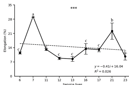
Figure 4. Elongation of buried specimens by pipe service life. Vertical bars represent the standard errors. Different letters indicate significant differences among groups (one-way ANOVA followed by LSD test; n = 6 ). Significance level: *** p < 0.001 .
