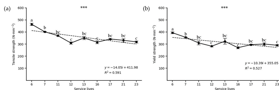
Figure 3. Tensile strength (a) and yield strength (b) of buried specimens by pipe service life. Vertical bars represent the standard errors. Different letters indicate significant differences among groups (one-way ANOVA followed by LSD test; n = 6 ). Significance level: *** p < 0.001 .
