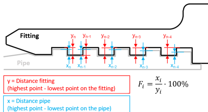
Figure 2. Definition of the groove filling levels.
