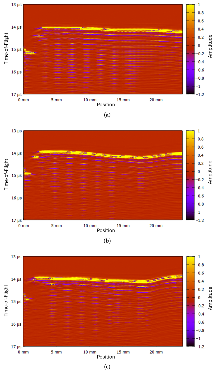
Figure 11. US B-Scans of pipe-fitting connections: (a) Pressed with low force. (b) Pressed with medium force. (c) Pressed with high force.
