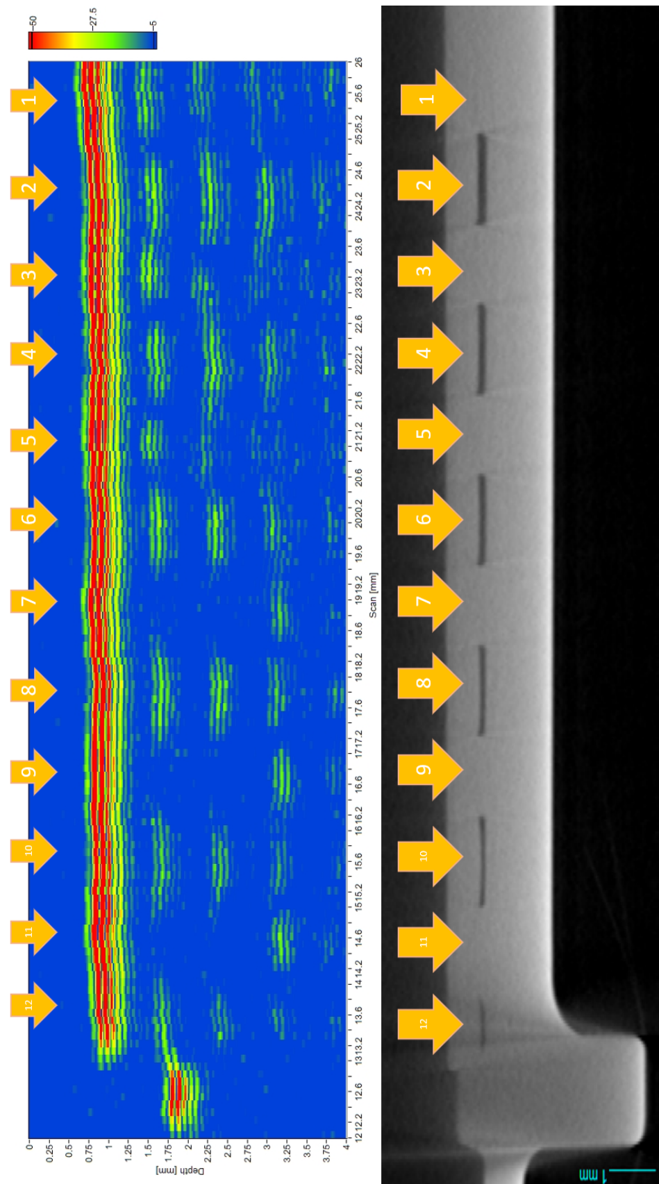
Figure 9. Comparison of HF-US-B image (left) and CT cross-section (right) of a pipe-fitting connection with several probe positions (numbered 1 to 12) marked (yellow arrows).
