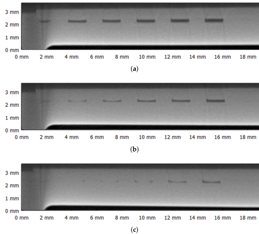
Figure 5. CT images of pipe-fitting connections: (a) Pressed with low force. (b) Pressed with medium force. (c) Pressed with high force.
