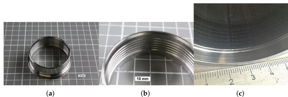
Figure 3. Photos of the specimens: (a,b) photos of the fittings with annular grooves on the inside. (c) Photo of a pressed pipe-fitting connection.
