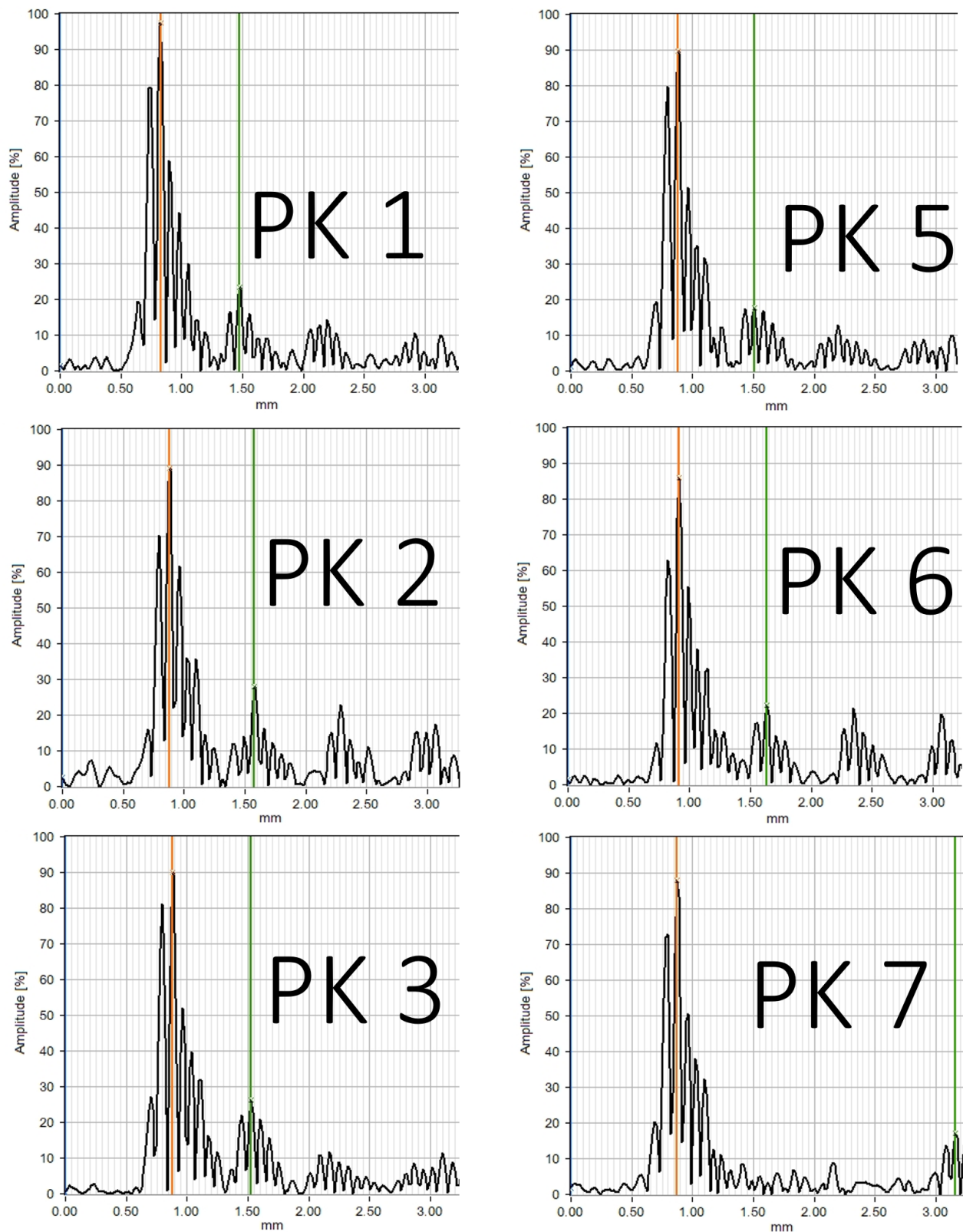
Figure 10. Manually evaluated transit time measurements for probe positions 1, 2 and 3 (left) and 5, 6 and 7 (right) of the single-sensor measurements. The orange line indicates the entry echo, while the green line indicates the echo of the groove or the adjacent bump.
