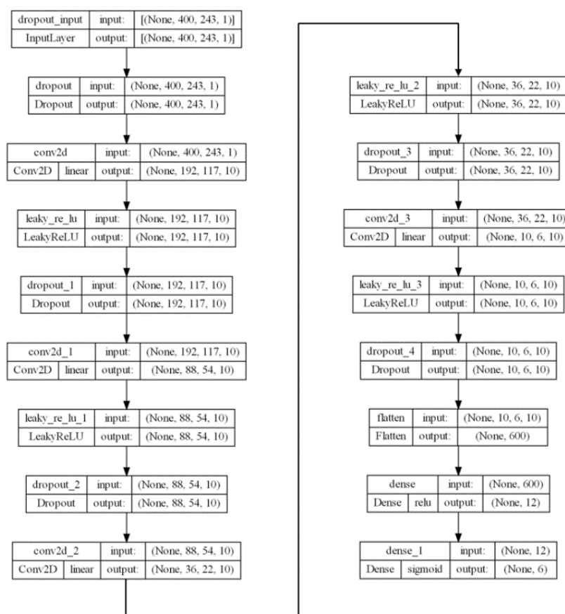
Figure 12. Architecture of the convolutional neural network employed.
