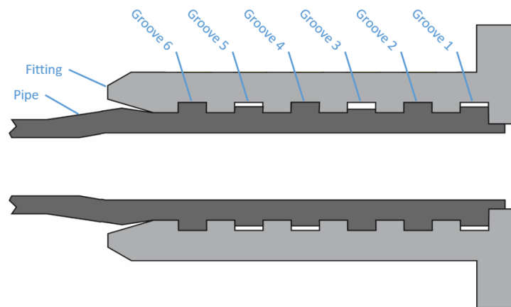
Figure 1. Schematic cross-section of a pipe-fitting connection with grooves.
