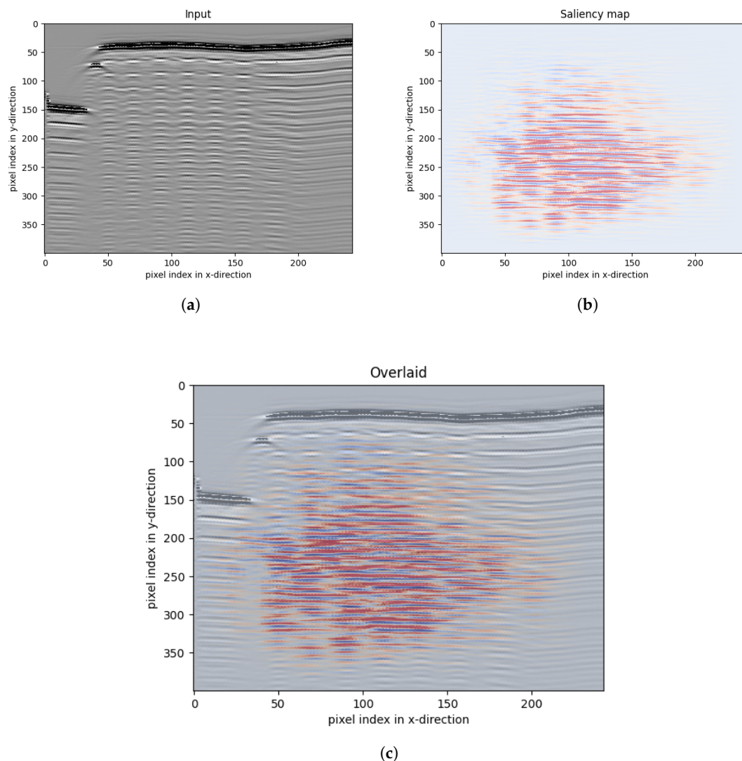
Figure 14. Visualization of Grad-CAM results for a BScan: (a) Input BScan. (b) Saliency map for this BScan. (c) BScan and saliency map overlaid.
