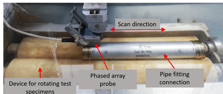
Figure 4. Test setup for phased array testing using HF-US from the outside of the pipe.
