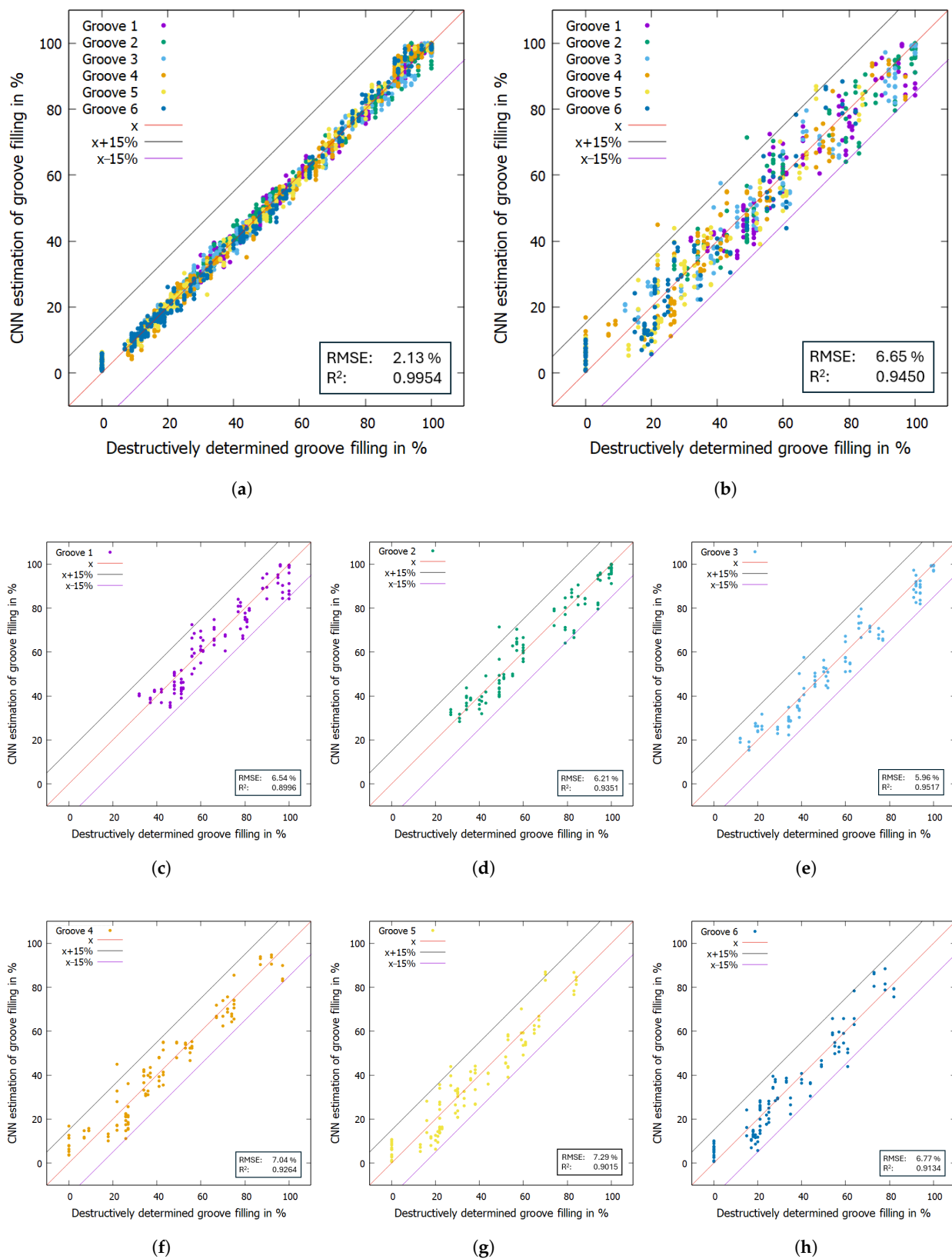
Figure 13. Comparison of the destructively determined groove fill levels and the output of the neural network: (a) training data; (b) test data; (c) test data—only first grooves; (d) test data—only second grooves; (e) test data—only third grooves; (f) test data—only fourth grooves; (g) test data—only fifth grooves; and (h) test data—only sixth grooves.
