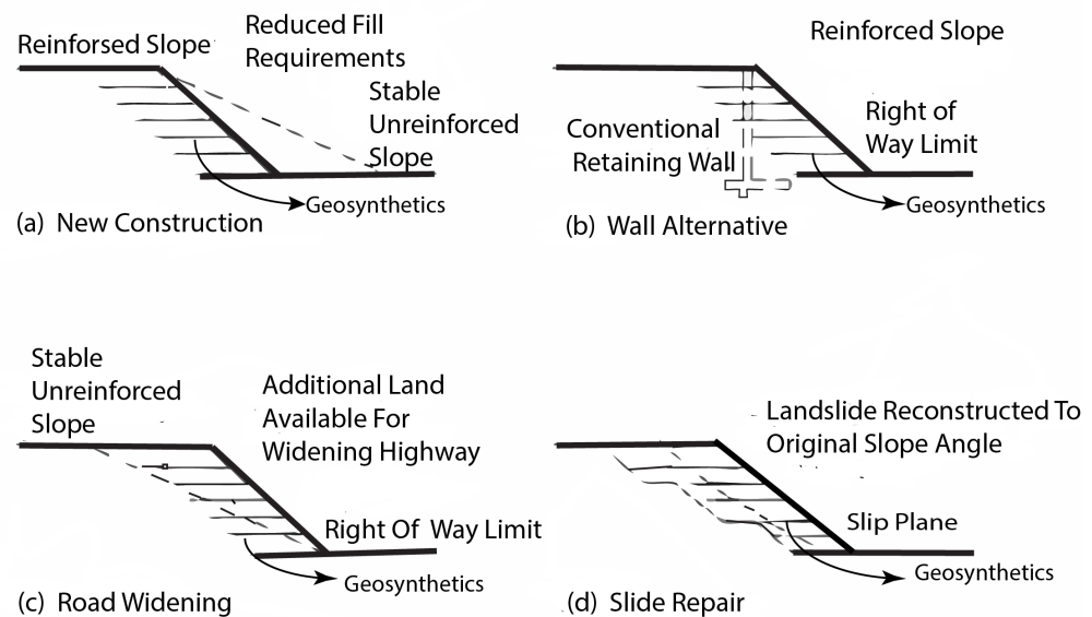
Figure 1. Geosynthetic reinforced steep slope applications [1].
