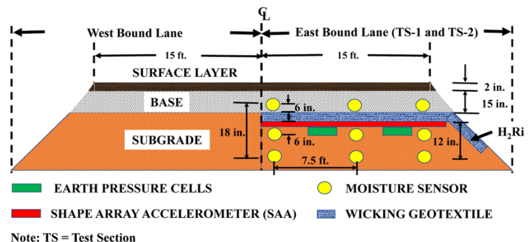
Figure 5. Schematic of test sections for evaluating the drainage performance of wicking geotextile in flexible pavements [24].
