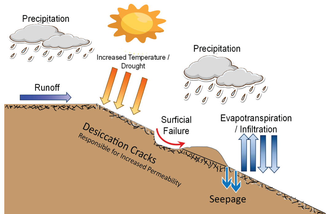
Figure 2. Schematic illustrating how climate-driven processes interact with slope conditions to influence surficial slope failure.
