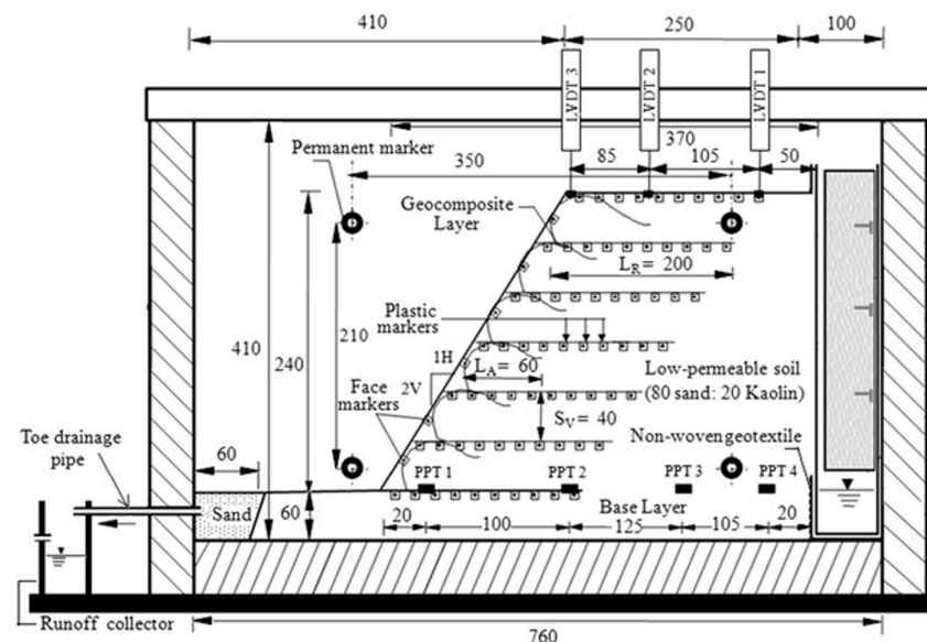
Figure 7. Illustration of the physical slope model with geocomposite layers used for slope stability analysis under rainfall conditions (all dimensions in mm) [33].
