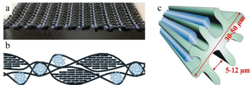
Figure 4. Wicking fabric. (a) fabric photo, (b) schematics of fabric cross-section, (c) schematics of a single wicking yarn [26].
