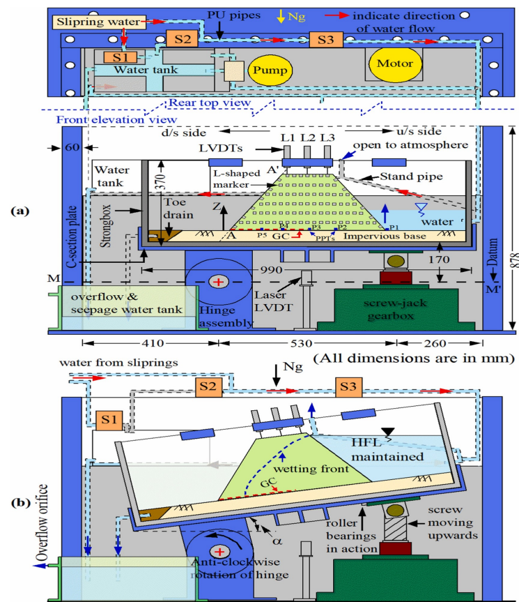
Figure 6. Schematic of the experimental setup illustrating (a) reservoir filling and (b) tilting at an angle [168].
