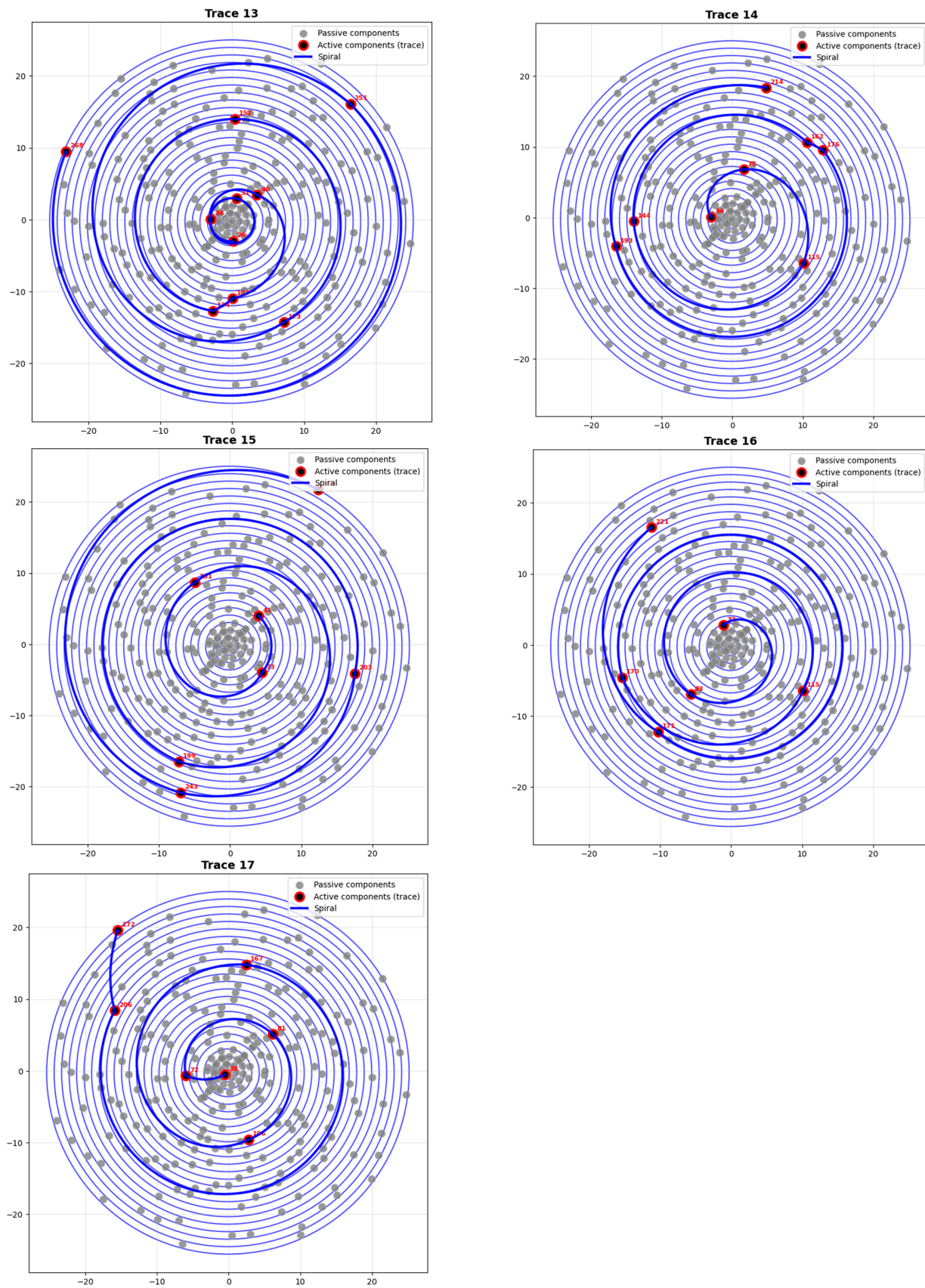
Figure 6. Seventeen traces of spirals on the coordinate plane.
