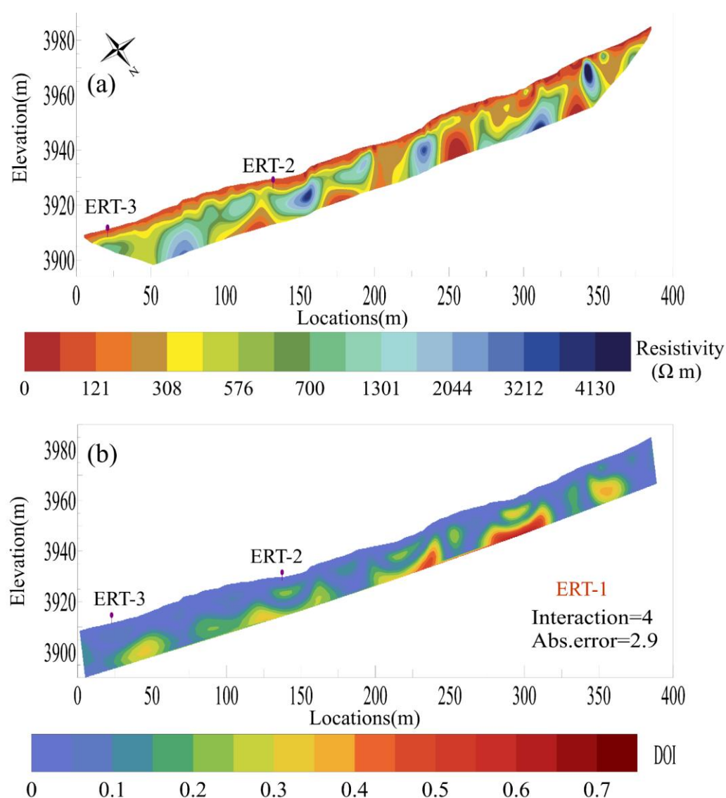
Figure 4. Longitudinal geoelectrical characterization of the active-layer detachment: (a) 2D inverted resistivity tomogram and (b) spatial distribution of the depth-of-investigation (DOI) index, demonstrating the data reliability and depth constraints of the geophysical inversion.
