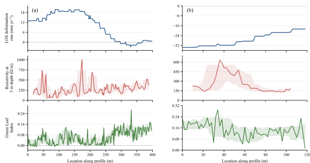
Figure 10. Spatial alignment of surface kinematics, subsurface geoelectrical structures, and eco-geomorphic indices along the primary landslide axes. (a) Longitudinal profile ERT1 of the active-layer detachment and (b) longitudinal profile ERT4 of the freeze–thaw-induced shallow creep landslide, illustrating the coupled relationships among multi-temporal InSAR-derived line-of-sight deformation rates (blue line), electrical resistivity values at a 5 m depth (red line), and the UAV-derived green leaf index (green line). The shaded envelopes indicate the local 10th–90th percentile range calculated within a 30 m moving window along each profile.
