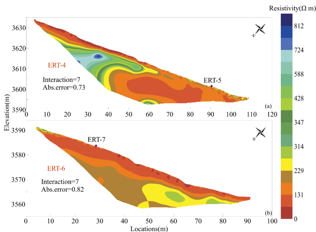
Figure 6. Longitudinal ERT inverted profiles across the upper part (a) and lower part (b) of the freeze–thaw-induced shallow creep landslide.
