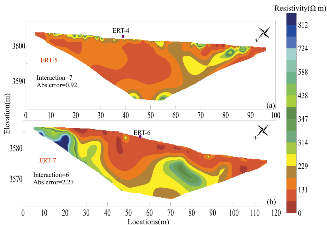
Figure 7. Transversal ERT inverted profiles across the (a) upper part and (b) lower part of the freeze–thaw-induced shallow creep landslide.
