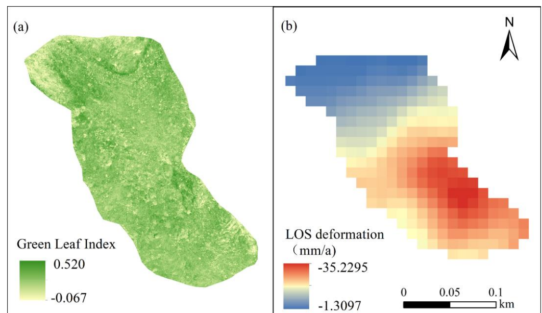
Figure 9. Eco-geomorphic characteristics and kinematic activity of the freeze–thaw-induced shallow creep landslide: (a) UAV-derived green leaf index map and (b) annual line-of-sight (LOS) ground deformation rate map computed from SBAS-InSAR processing.
