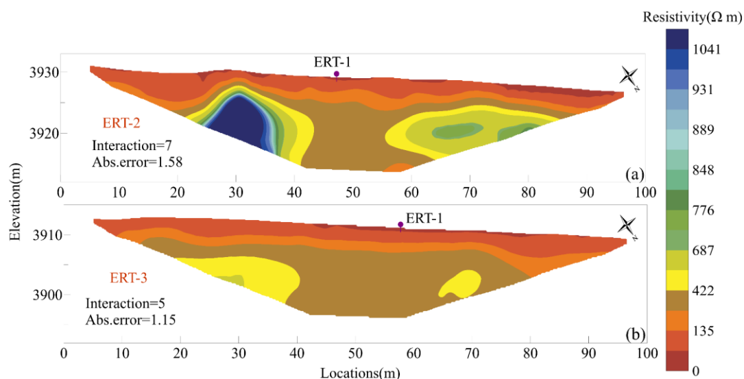
Figure 5. Transverse ERT inverted profiles in the frontal accumulation lobe (a) and outside the frontal margin (b) of the active-layer detachment.
