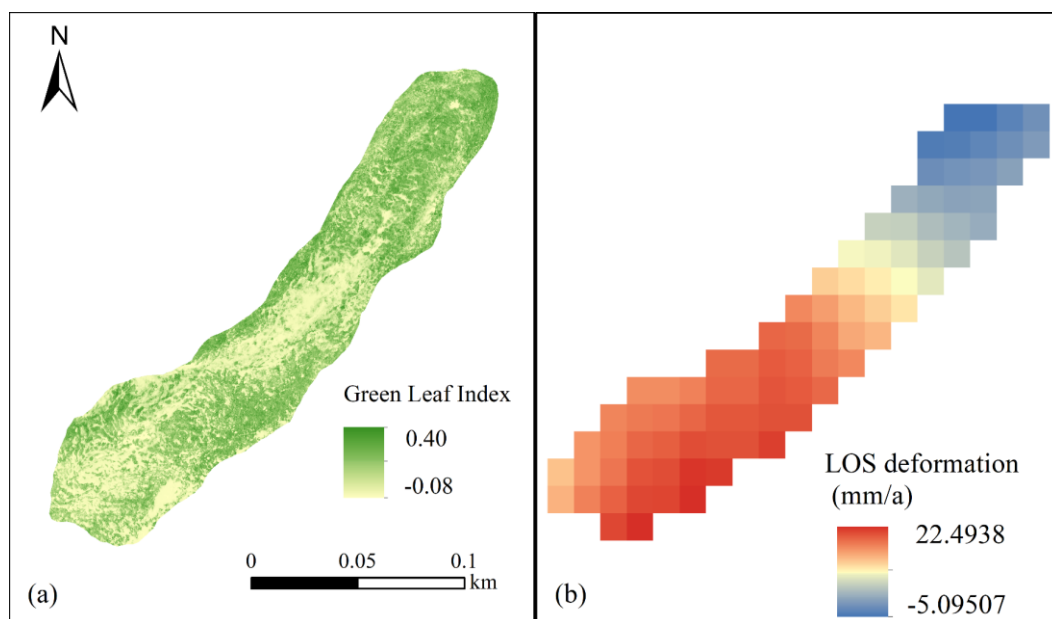
Figure 8. Eco-geomorphic characteristics and kinematic activity of the active-layer detachment complex: (a) UAV-derived green leaf index map and (b) annual line-of-sight (LOS) ground deformation rate map computed from SBAS-InSAR processing.
