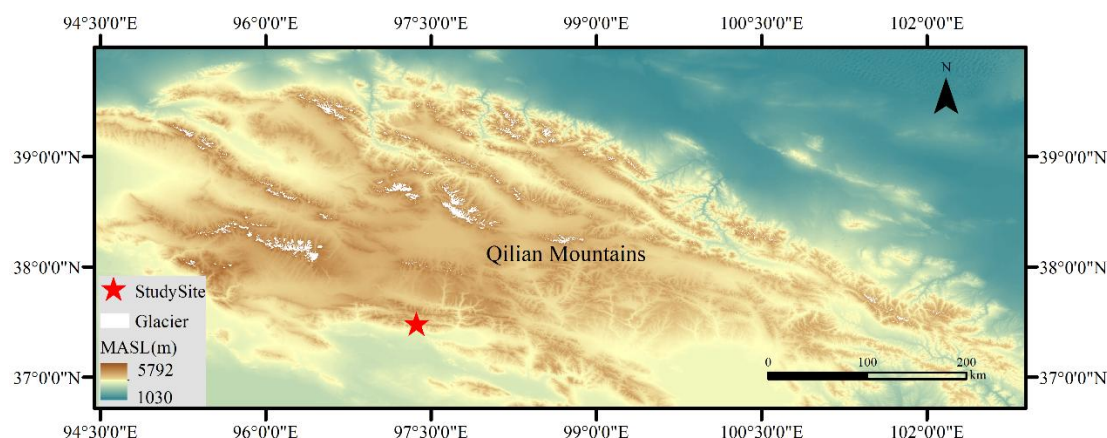
Figure 1. Study site in the western subrange of the Qilian Mountains, Qinghai Province, China. Notes: Elevation data were downloaded from STER V4 DEM accessed on 23 September 2014 ( http://gdex.cr.usgs.gov/gdex ).
