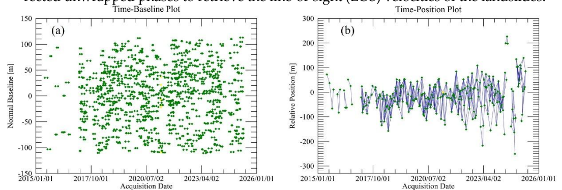
Figure 2. Connections between the Sentinel-1 SAR acquisitions with the spatial (a) and temporal baselines (b).
