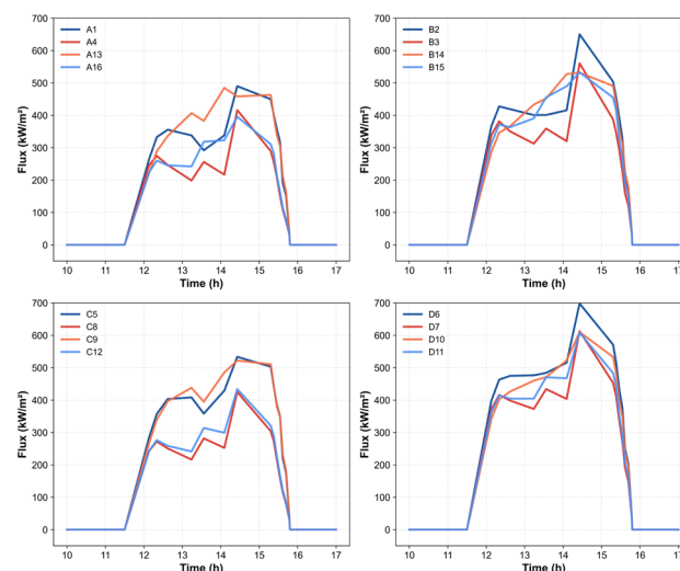
Figure 9. Transient operating conditions. Evolution of incident solar flux across individual modules.
