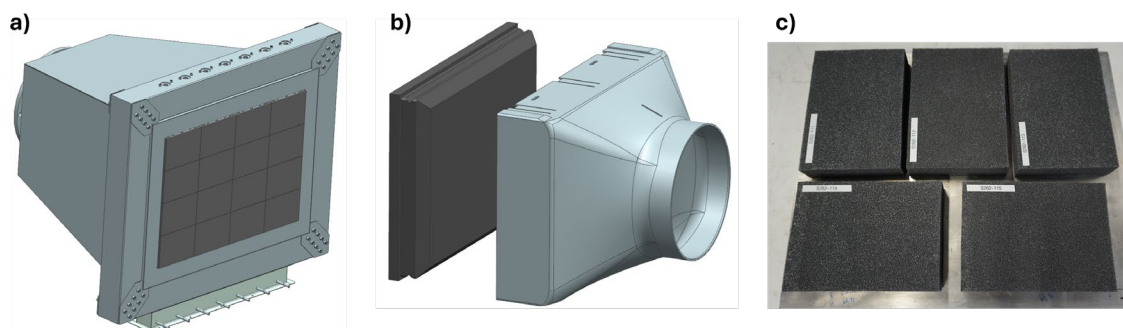
Figure 4. (a) 500\text{ kW}_{\text{th}} receiver design composed of 16 modules, each measuring 24.65\text{ cm} \times 17.5\text{ cm} . (b) Rear view of one unassembled module consisting of a ceramic foam absorber and one cup. (c) Photograph of ceramic foam absorbers awaiting installation in the receiver front frame.
