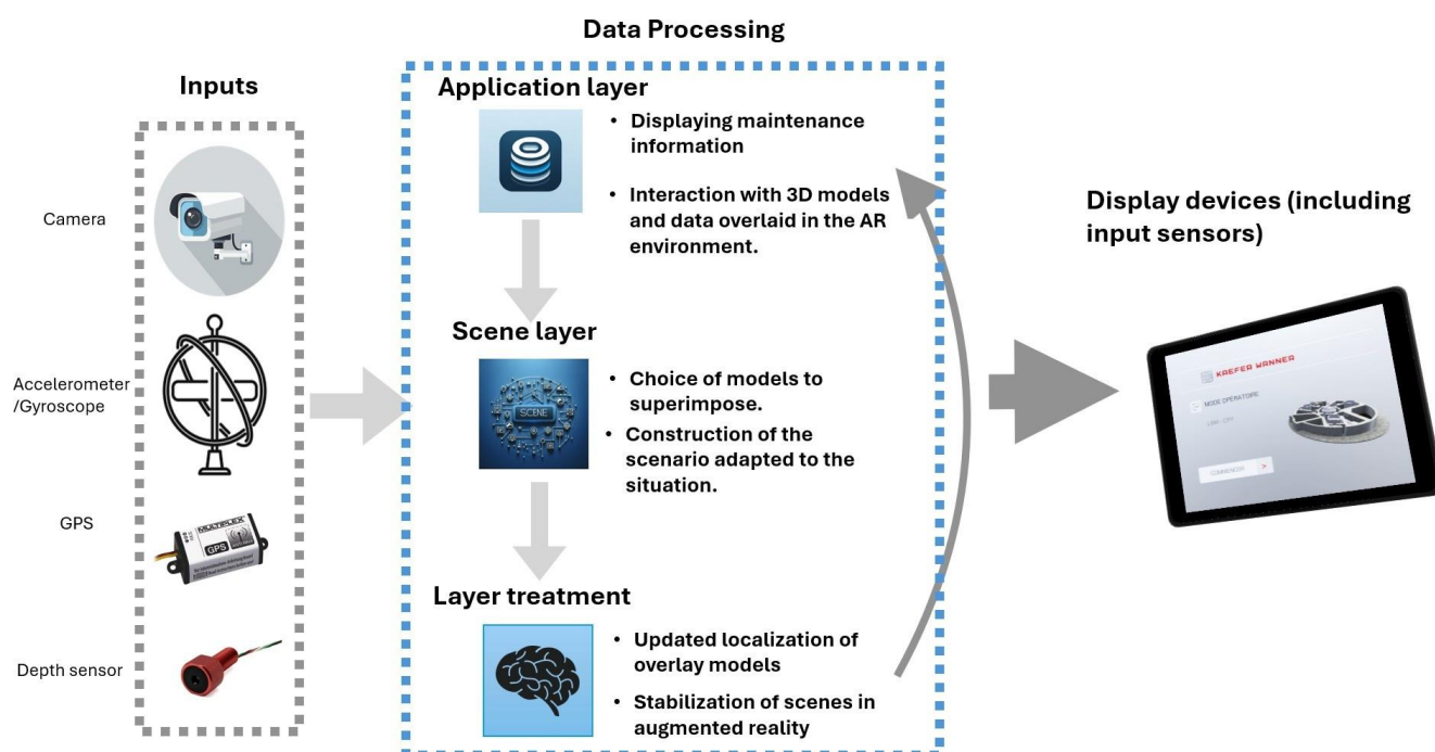
Figure 11. Overall Flow Diagram for Software Development Process.
