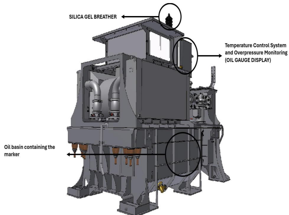
Figure 9. Components of the MT Modeled for Accurate Oil Level Measurement.
