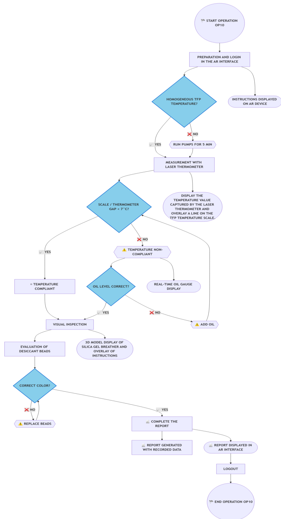
Figure 10. Implementation Framework and Reasoning for Integrating AR into OP10 Maintenance Steps.
