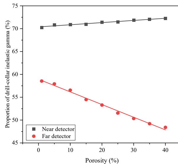
Figure 3. Proportion of drill-collar inelastic gamma.
