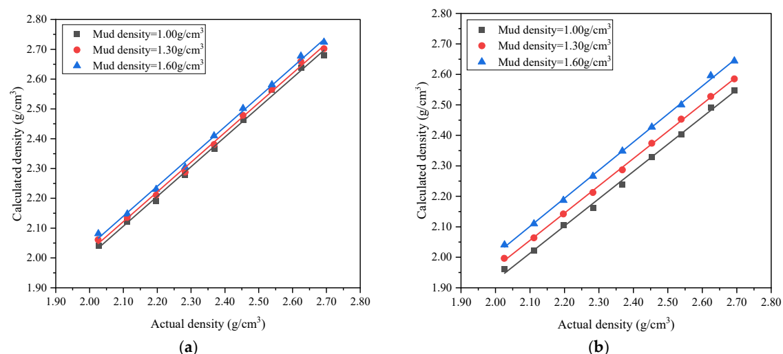
Figure 9. The effect of borehole environment on DNGD. (a) Borehole size is 20 cm. (b) Borehole size is 30 cm.
