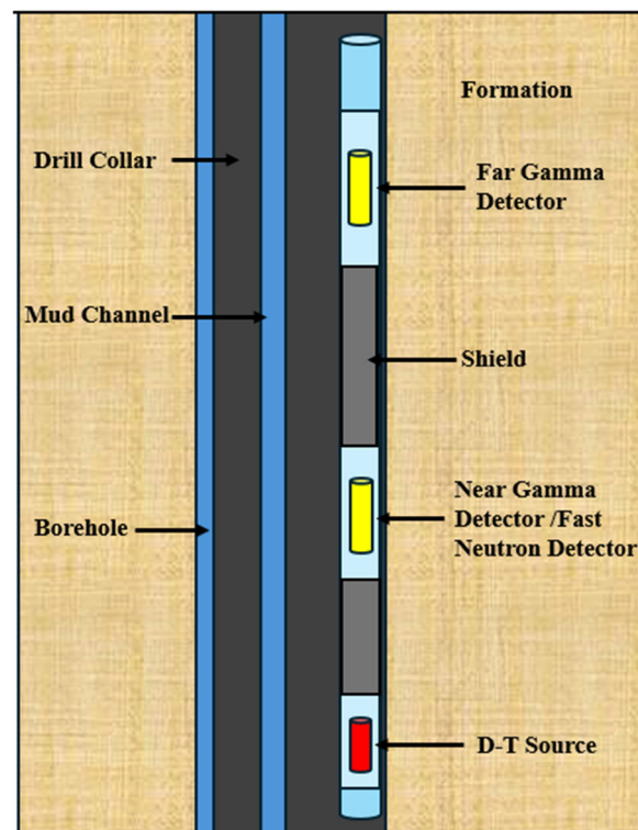
Figure 1. Simulation model example.
