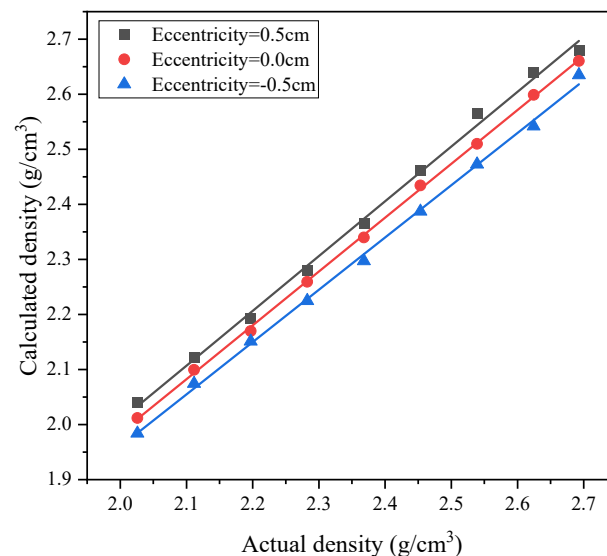
Figure 12. The effect of tool eccentricity on DNGD.
