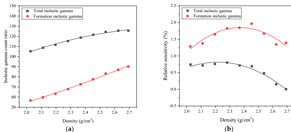
Figure 4. Comparison between the total inelastic gamma and the formation inelastic gamma. (a) Variation in the inelastic gamma count ratio with density. (b) Comparison of the relative sensitivity of the formation inelastic gamma and drill-collar inelastic gamma.
