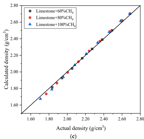
Figure 7. Calculated density results for gas-bearing formations. (a) Results of the DNGD in gas-bearing formations. (b) Results of the CNGD in gas-bearing formations. (c) Results of the FNGD in gas-bearing formations.
