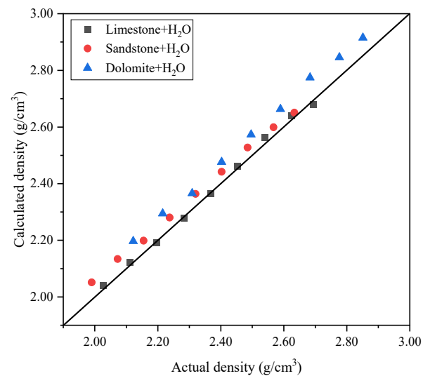
Figure 10. The effect of different lithologies on DNGD.
