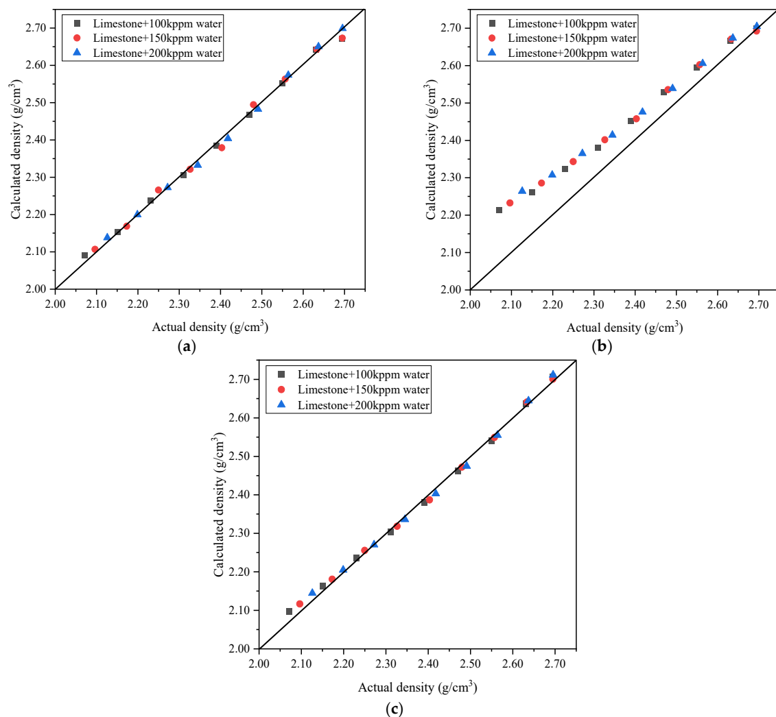
Figure 8. Calculated density results for high-salinity formations. (a) Results of the DNGD in high-salinity formations. (b) Results of the CNGD in high-salinity formations. (c) Results of the FNGD in high-salinity formations.
