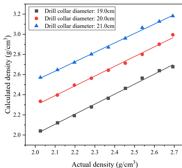
Figure 13. The effect of drill-collar diameter on DNGD.
