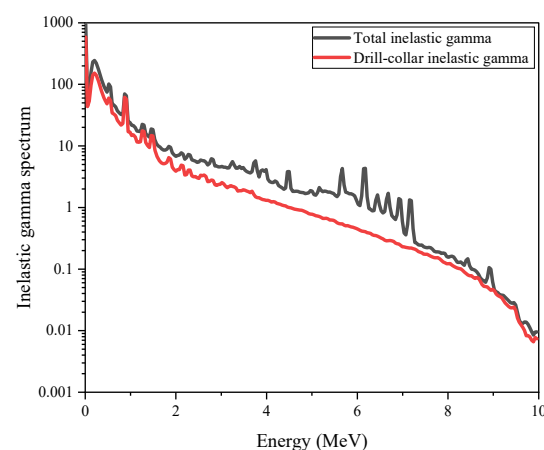
Figure 2. Comparison of different inelastic gamma spectra.
