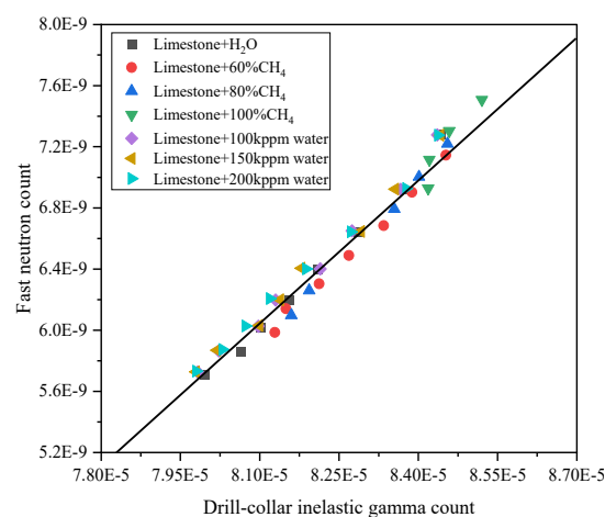
Figure 5. Relationship between drill-collar inelastic gamma count and fast neutron count.
