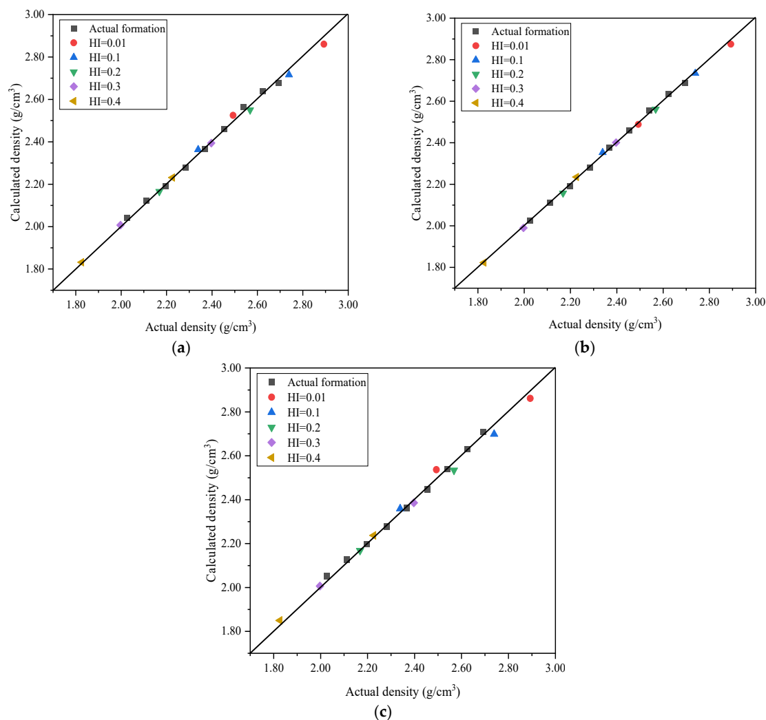
Figure 6. Calculated density results for limestone with different densities and HI. (a) Results of DNGD application in freshwater-saturated limestone. (b) Results of CNGD application in freshwater-saturated limestone. (c) Results of FNGD application in freshwater-saturated limestone.
