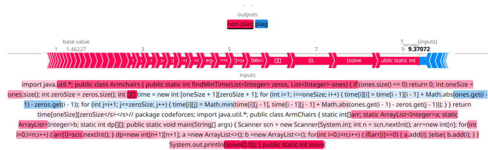
Figure A5. UniXcoder TN example.
