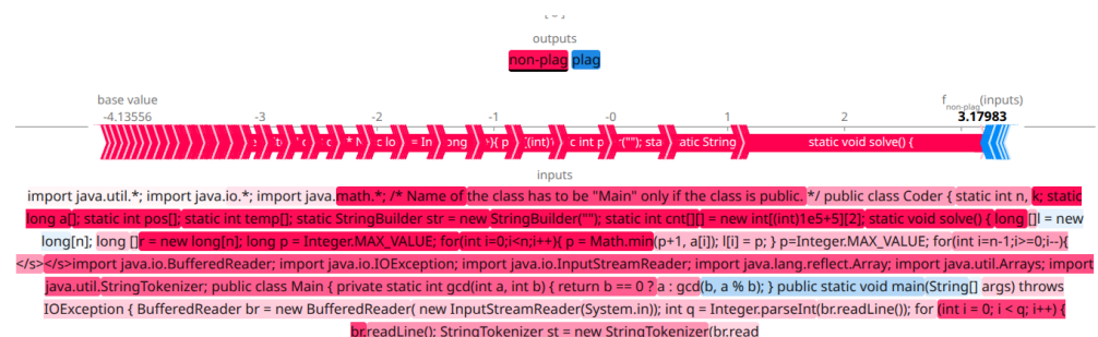
Figure A7. GraphCodeBERT FN example.
