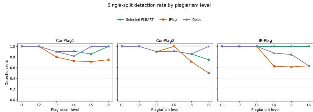
Figure 6. Single-split plagiarism-level detection for the selected PLBART, JPlag, and Dolos.
