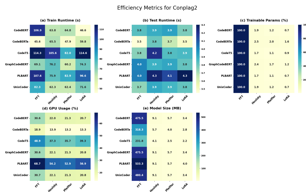
Figure A9. ConPlag template-free efficiency comparison heat maps. The colour bars show the value scale, and darker blue cells indicate larger values within each metric. (a) Training time in seconds. (b) Inference time in seconds. (c) Percentage of trainable parameters. (d) Percentage of GPU usage. (e) Model size in MB for the pre-trained models and adapters.
