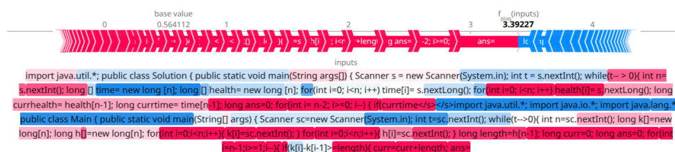
Figure A8. CodeT 5 FP example.
