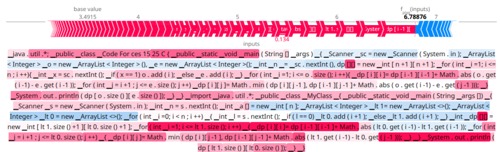
Figure A6. PLBART TP example.
