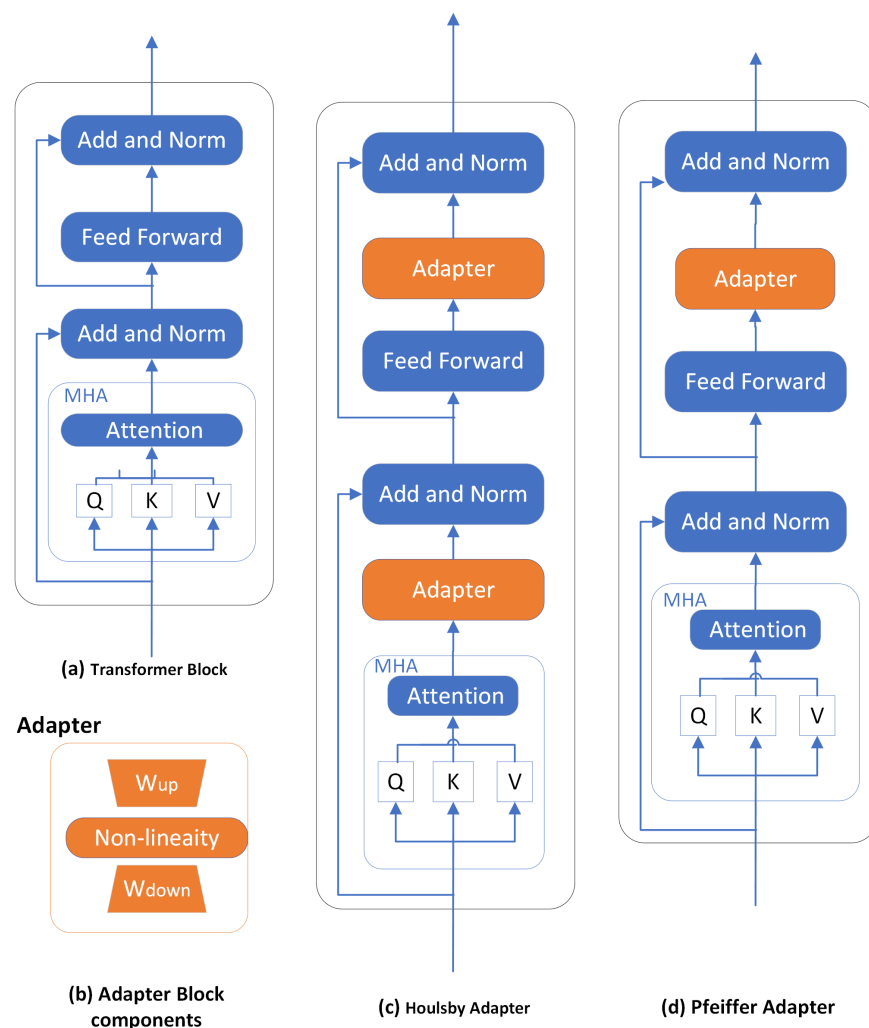
Figure 3. A single Transformer block architecture, adapters, and adapter block [4,14,40,41]. (a) Transformer encoder architecture. (b) Adapter block components. (c) Houlsby adapter. (d) Pfeiffer adapter.
