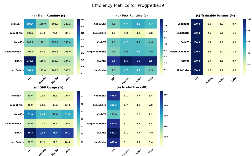
Figure A11. Progpedia-19 efficiency comparison heat maps. The colour bars show the value scale, and darker blue cells indicate larger values within each metric. (a) Training time in seconds. (b) Inference time in seconds. (c) Percentage of trainable parameters. (d) Percentage of GPU usage. (e) Model size in MB for the pre-trained models and adapters.
