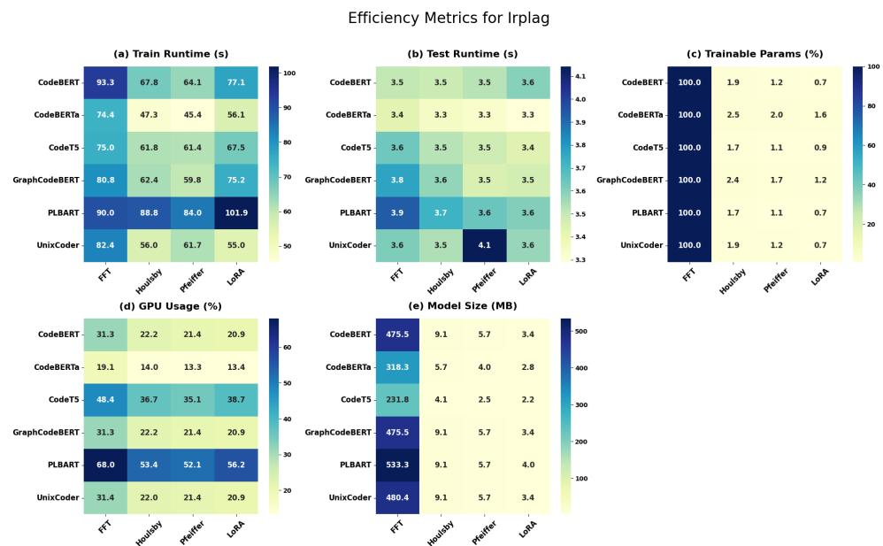
Figure A10. IR-Plag efficiency comparison heat maps. The colour bars show the value scale, and darker blue cells indicate larger values within each metric. (a) Training time in seconds. (b) Inference time in seconds. (c) Percentage of trainable parameters. (d) Percentage of GPU usage. (e) Model size in MB for the pre-trained models and adapters.
