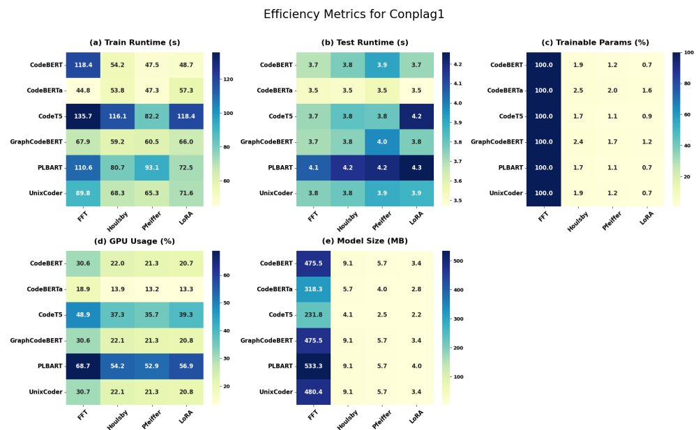
Figure 5. ConPlag raw efficiency comparison heat maps. The colour bars show the value scale, and darker blue cells indicate larger values within each metric. (a) Training time in seconds. (b) Inference time in seconds. (c) Percentage of trainable parameters. (d) Percentage of GPU usage. (e) Model size in MB for the pre-trained models and adapters.
