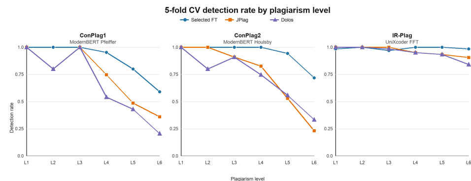
Figure 7. Five-fold cross-validation plagiarism-level detection for the best fine-tuned, JPlag, and Dolos.
