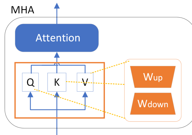
Figure 4. LoRA adapter architecture [6].
