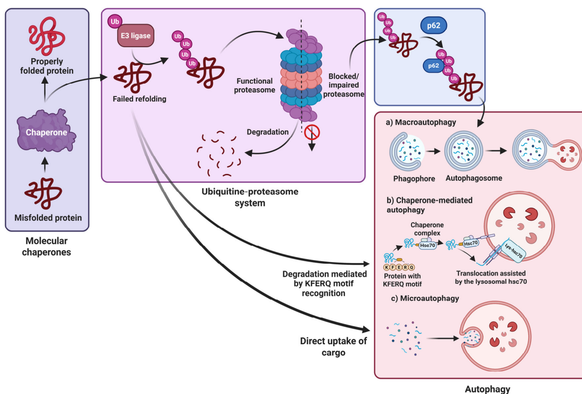
Figure 3. Schematic overview of the cellular proteostasis network (Molecular chaperones, the UPS, and autophagy cooperate to preserve protein quality control. Misfolded proteins are initially subjected to chaperone assisted refolding. If refolding fails, proteins are ubiquitinated and targeted for proteasomal degradation. When proteasomal capacity is exceeded, autophagy provides a complementary degradative pathway through macroautophagy, CMA, and microautophagy. Age-
