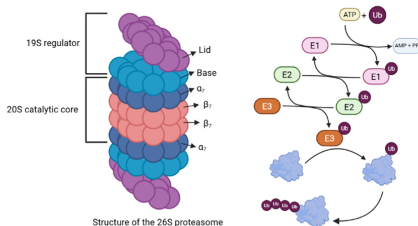
Figure 2. Structure of the 26S proteasome and mechanism of ubiquitination.
