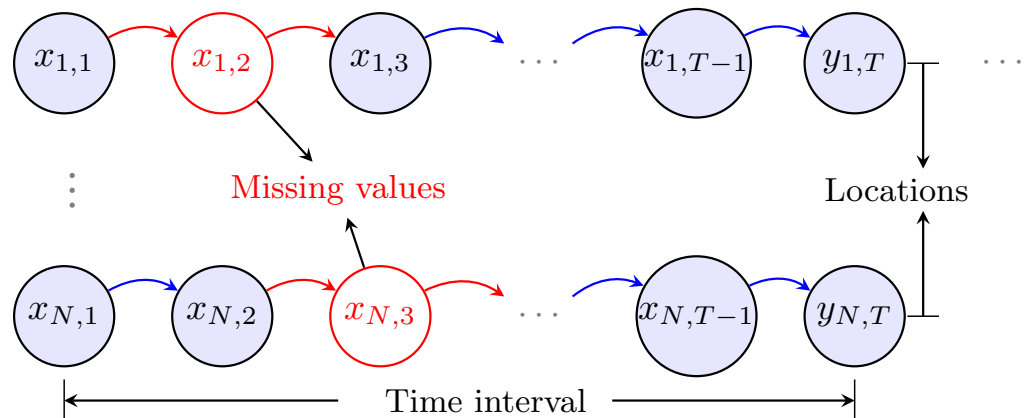
Figure 1. Example of electricity load multivariate time series.
