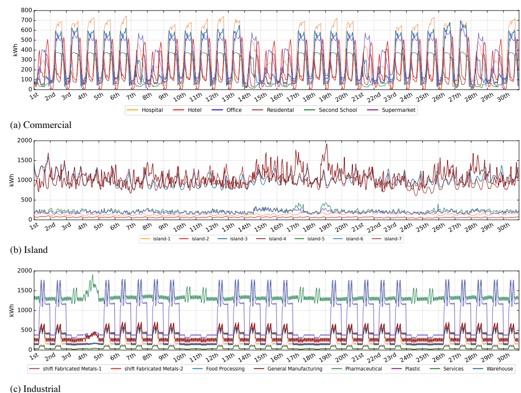
Figure 3. The first month's plots of three benchmark datasets with 720 timestamps.
