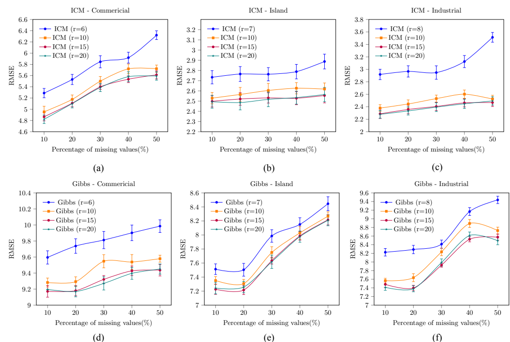
Figure 4. Performance of Gibbs sampling and ICM with different ranks on three datasets.
