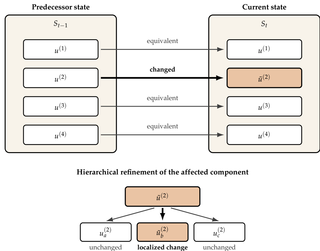
Figure 5. State equivalence, component-level change, and hierarchical refinement in the proposed change model. Equality is first evaluated at the document-state level. If inequality is detected, refinement proceeds within the hierarchy to localize the affected component and, if necessary, the changed subcomponent. In the example, the second component differs between S_{t-1} and S_t , and refinement localizes the change further to \tilde{u}_b^{(2)} .
