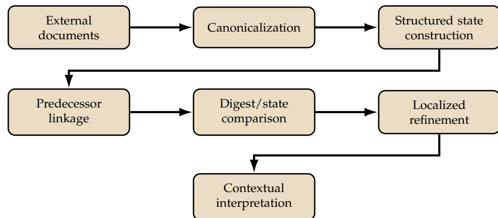
Figure 6. Operational flow of the proposed state-centric framework. External document artifacts are transformed into canonical structured states, linked to predecessor versions, compared through digest- or state-based mechanisms, refined locally in the case of detected differences, and finally interpreted with respect to contextual relevance.
