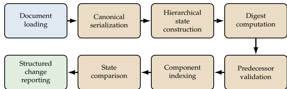
Figure 7. Processing pipeline of the Python reference prototype used in the reproducible operational case study. Each input document is loaded and transformed into a canonical serialization from which a hierarchical document state and its associated digests are constructed. After validation of the predecessor relation, components are indexed to establish the correspondence required for comparison. The resulting current and predecessor states are then compared recursively, and detected differences are returned as a structured change report.
