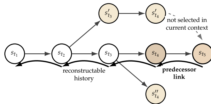
Figure 4. Predecessor-based historical reconstruction in a branching state graph. Although several branches may exist, the predecessor mapping identifies the contextually valid path for the current state s_{t_5} . Repeated application of \text{pred}(\cdot) reconstructs the corresponding evolution history until an initial state is reached.
