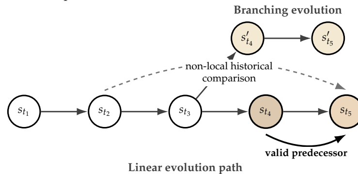
Figure 3. Temporal evolution in the proposed framework. Document states form linear or branching paths in the state graph G_{\mathcal{R}} . For the current state s_{t_5} , comparison is anchored to the valid predecessor s_{t_4} rather than to a non-local historical state such as s_{t_2} .
