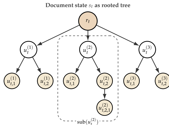
Figure 2. Hierarchical tree representation of a document state. The root node r_t represents the complete state s_t , internal and leaf nodes represent structural components, and directed edges encode parent–child relations. Highlighted subtrees define localized regions for comparison and refinement. Nodes represent document components, edges encode hierarchy. subtrees define local comparison regions.
