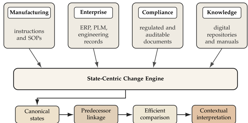
Figure 8. Application-oriented view of the proposed state-centric framework. The upper row uses a neutral color to indicate heterogeneous application domains that can provide evolving document artifacts. The lower row uses the same functional color sequence as the conceptual architecture: representation through canonical states, temporal organization through predecessor linkage, comparison through efficient state evaluation, and interpretation through contextual assessment. The figure illustrates how heterogeneous document-driven domains can be mapped to a common change engine while preserving domain-specific interpretation.
