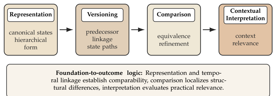
Figure 1. Conceptual architecture and workflow of the proposed framework. External document artifacts are first transformed into canonical hierarchical states. These states are then embedded in explicit predecessor relations, compared through deterministic equivalence and refinement operations, and finally interpreted according to application-specific relevance criteria. The figure therefore summarizes the complete progression from representation to contextual interpretation and serves as a roadmap for the methodological sections that follow.
