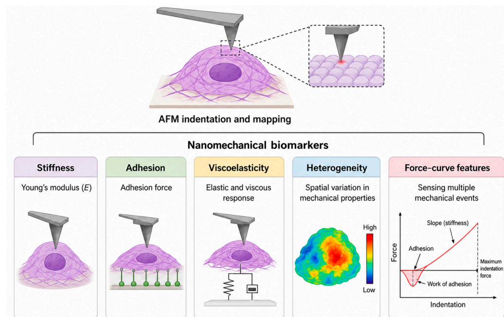
Figure 1. Overview of AFM-derived nanomechanical biomarkers. AFM indentation and mapping of biological samples generate key nanomechanical biomarkers, including Young's modulus, adhesion, viscoelasticity, and mechanical heterogeneity. Together, these multiparametric readouts define nanomechanical fingerprints that can be used for cell and tissue phenotyping, disease classification, and treatment monitoring. A multiparametric AI model should ideally include complementary AFM-derived features rather than a single mechanical descriptor. Relevant inputs may include Young's modulus, adhesion force, work of adhesion, viscoelastic descriptors, roughness, force-curve hysteresis, stiffness-distribution parameters, and spatial heterogeneity. The most appropriate
