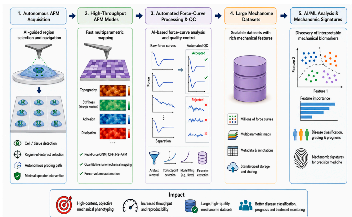
Figure 4. Automated and high-throughput AFM mechanics workflow. AI-assisted AFM mechanomics enables scalable and reproducible nanomechanical phenotyping by integrating autonomous AFM acquisition, high-throughput mapping modes, automated force-curve processing, quality control, and large mechanome dataset generation. These standardized multiparametric datasets can then be analyzed using AI/ML approaches to extract interpretable mechanomic signatures for disease classification, grading, prognosis, treatment monitoring, and precision mechanobiology.
