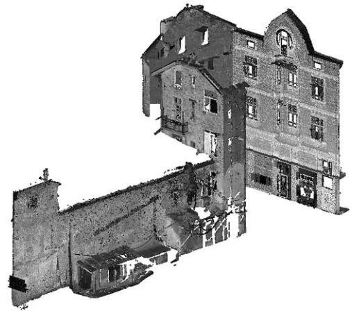
3a. 3D laser scan of façade facing Blvd. “Christo Botev” and digital model, -2025
