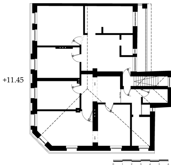
Restorative architectural survey plan level +11.45
