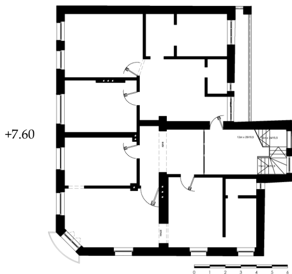
Restorative architectural survey plan level +7.60
