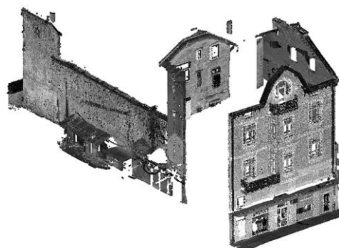
2a 3D laser scan of façade facing Blvd. “Christo Botev” and digital model, -2025
