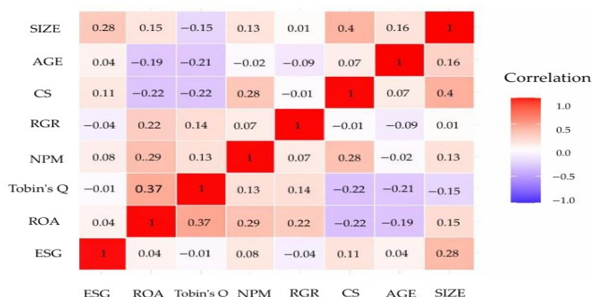
Figure 2. Correlation matrix heatmap of ESG score and financial indicators.
