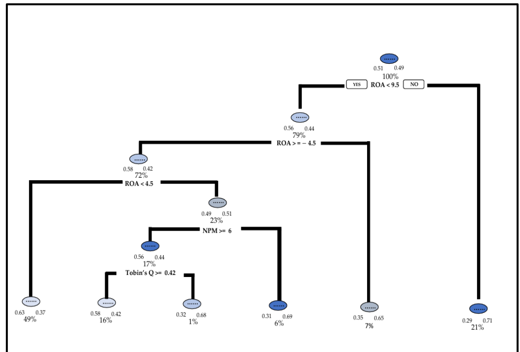
Figure 1. Decision Tree splitting process for the full Sample.
