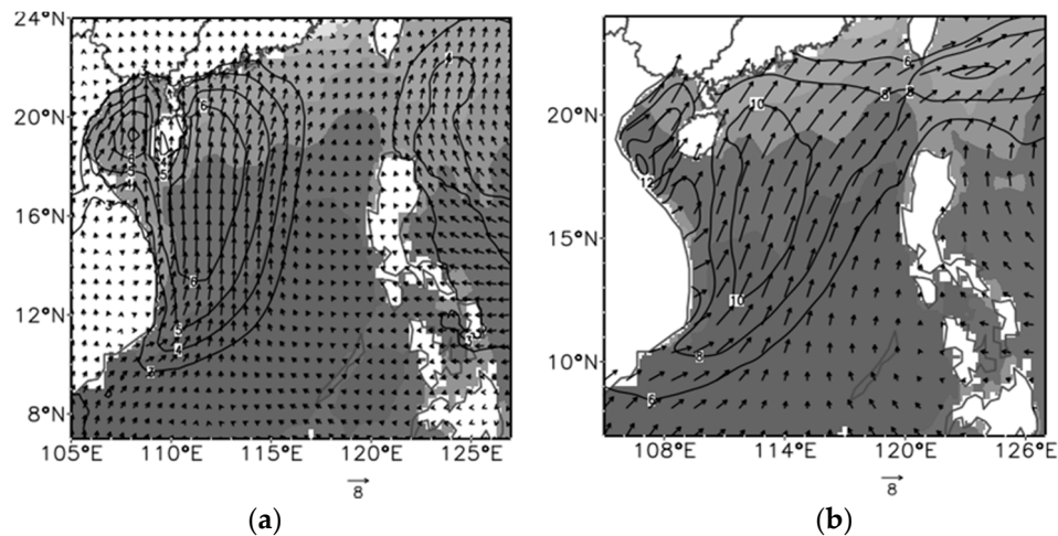
Figure 12. (a) ERA interim fields of the synoptic monthly means of the sea surface temperature (shaded, °C), 10 m wind speed (contour, \text{ms}^{-1} ), and wind barbs of May 2015. (b) ERA interim daily fields at 0000 UTC in late May (from 20 May to 30 May) of the sea surface temperature (shaded, °C), horizontal wind speed (contour, \text{ms}^{-1} ), and wind barbs at 950 hPa.
