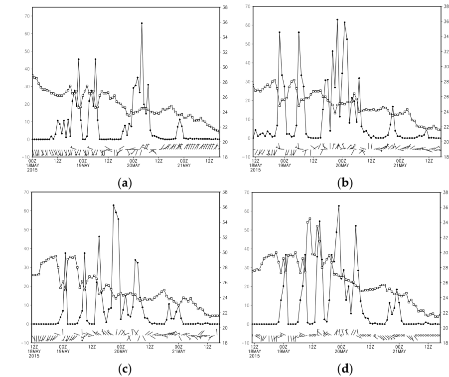
Figure 2. Time series of the hourly precipitation, temperature, and horizontal wind at four weather stations in the WSTR: (a) Haifeng, (b) G1803, (c) G1827, and (d) G1847. The line with empty squares represents the temperature, and the line with filled dots represents the precipitation.
