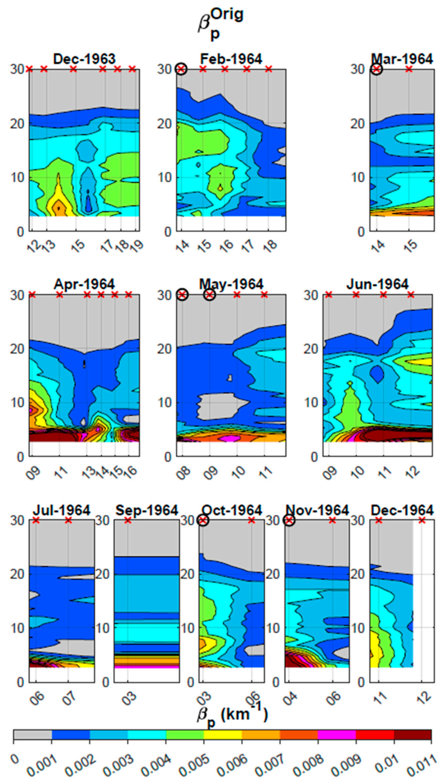
Figure 6. Cross sections of the original aerosol extinction profiles ( \beta_p^{\text{Orig}}(z) ) for the set of days available each month. The red crosses on top of the panels, at the 30 km altitude, indicate the dates the daily average observations were conducted. The red crosses inside a black circle indicate that blowing dust (visibility less than 11 km) was reported at nearby weather stations the day the nocturnal searchlight measurement was conducted.
