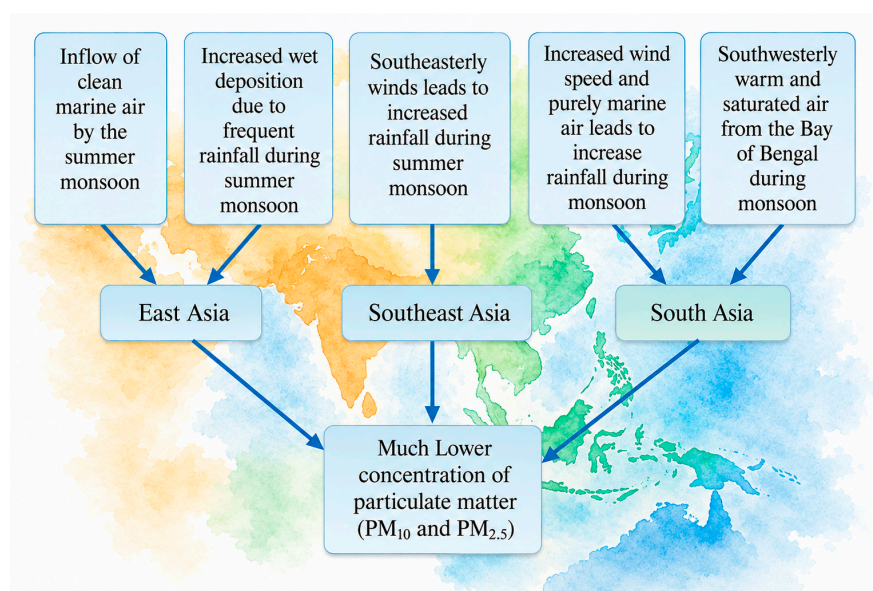
Figure 4. Schematic diagram of factors impacting air pollution in the monsoon.
