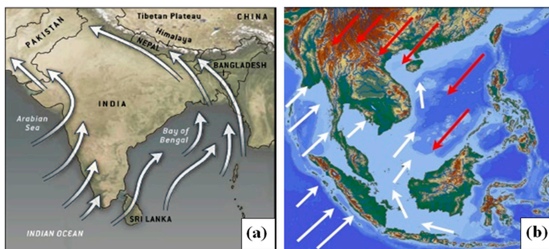
Figure 7. (a). Warm, saturated air from the Indian Ocean and the Bay of Bengal results in the summer monsoon in South Asia (Source: [111]); (b). Southeast Asian monsoon system where the red arrows
