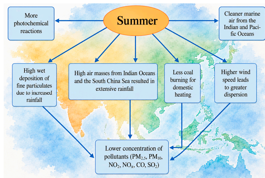
Figure 5. Schematic diagram of air pollution status in summer in Asia.
