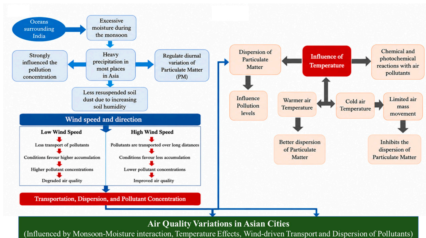
Figure 2. Schematic illustration of the effects of monsoonal moisture, wind speed and direction, and temperature on pollutant transport, dispersion, atmospheric accumulation, photochemical reactions, and seasonal air quality in Asian cities.
