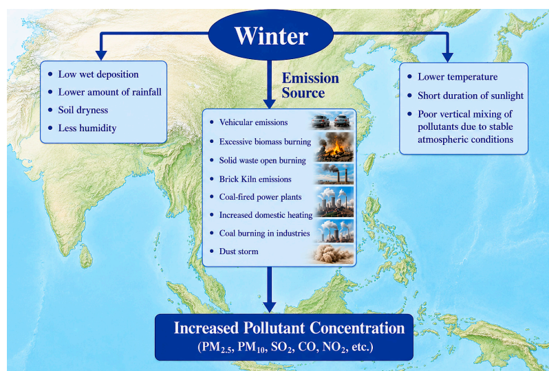
Figure 3. Schematic diagram of air pollution status in winter with primary emission sources.
