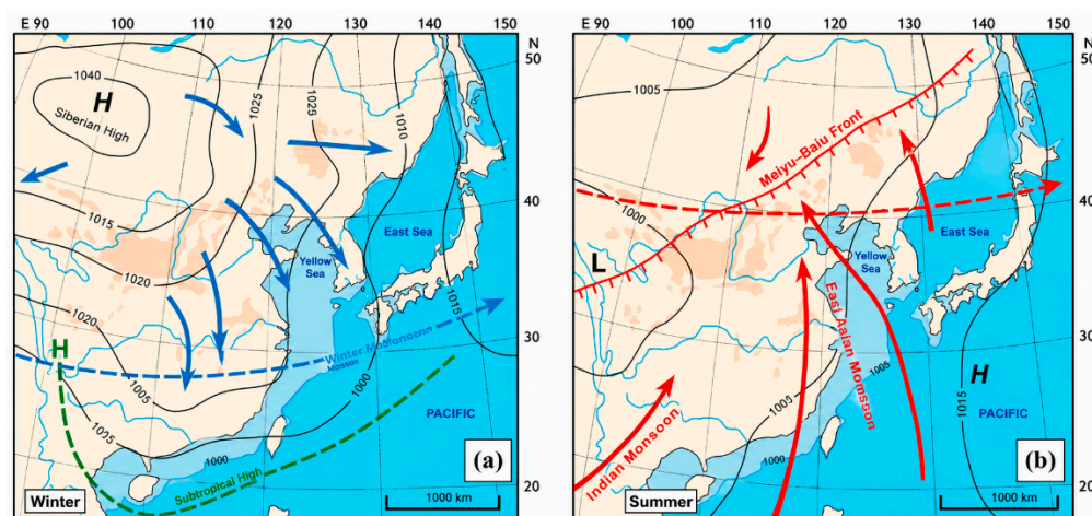
Figure 6. (a) East Asian winter and (b) summer monsoon system (Source: [106]).
