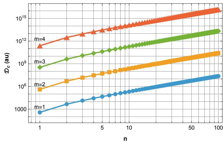
Figure 8. ECSC neoclassically estimated critical \mathcal{D}_c for l = 0 states for the upper wells (secondary: m = 1 and tertiary: m = 2, \dots ) residing between z = 2\pi m \pm (-\pi/2, +\pi/2) . The values shown were calculated by numerical integration of the phase-space integrals, followed by the neoclassical quantization condition. Similarly accurate results can be obtained from the simple formula, with small adjustments to the shape factors c (for the higher wells, c \approx 1.17 ). The manifolds corresponding to different wells ( m ) overlap above n_m \approx 13 , which will affect interpretation of spectra at macroscopic length scales.
