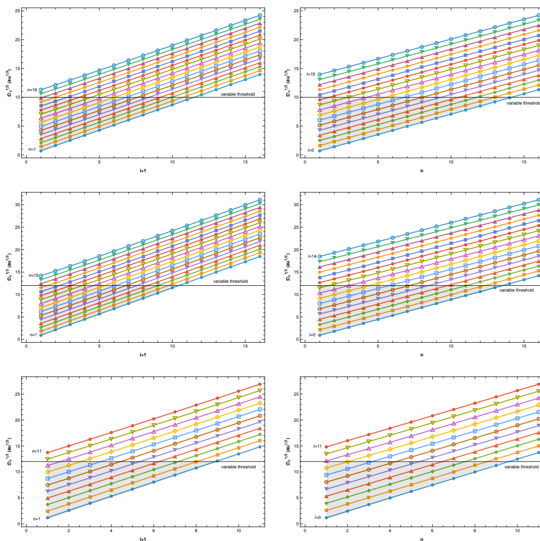
Figure 14. \sqrt{\mathcal{D}_c} vs. l + 1 and n for (from top): Hulthén, Yukawa, and ECSC potentials. The curves in the left panels correspond to increasing values of n starting with n=1 . Each curve increments n by 1 between n=1 and the upper n values as shown, which differ for the three potentials. The curves in the right panels similarly correspond to increasing values of l starting with l=0 . Each curve increments l by 1 between l=0 and the upper l values as shown, which differ for the three potentials. Note the near-constant density of states vs. l and n , which extends indefinitely in both n and l (modulo tick-tock glitches). As the threshold \sqrt{\mathcal{D}} is varied, the number of states is proportional to the shaded area, which grows as \propto (\sqrt{\mathcal{D}})^2 = \mathcal{D} . This explains the linearity seen by Rogers et al., Figure 5, and Lam and Varshni, Figure 2, as well as our extensions to them.
