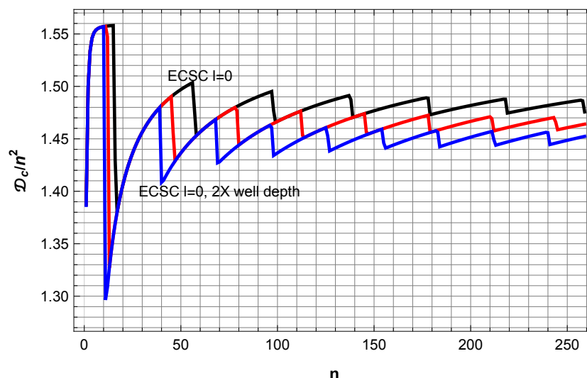
Figure 4. \mathcal{D}_c/n^2 vs. n for ECSC l=0 potential with well depths increased by well scale factors of \text{wsf} = 1, \frac{3}{2}, 2 , which respectively have colors black, red, and blue. The well depth reduces the period approximately as 1/\sqrt{\text{wsf}} .
