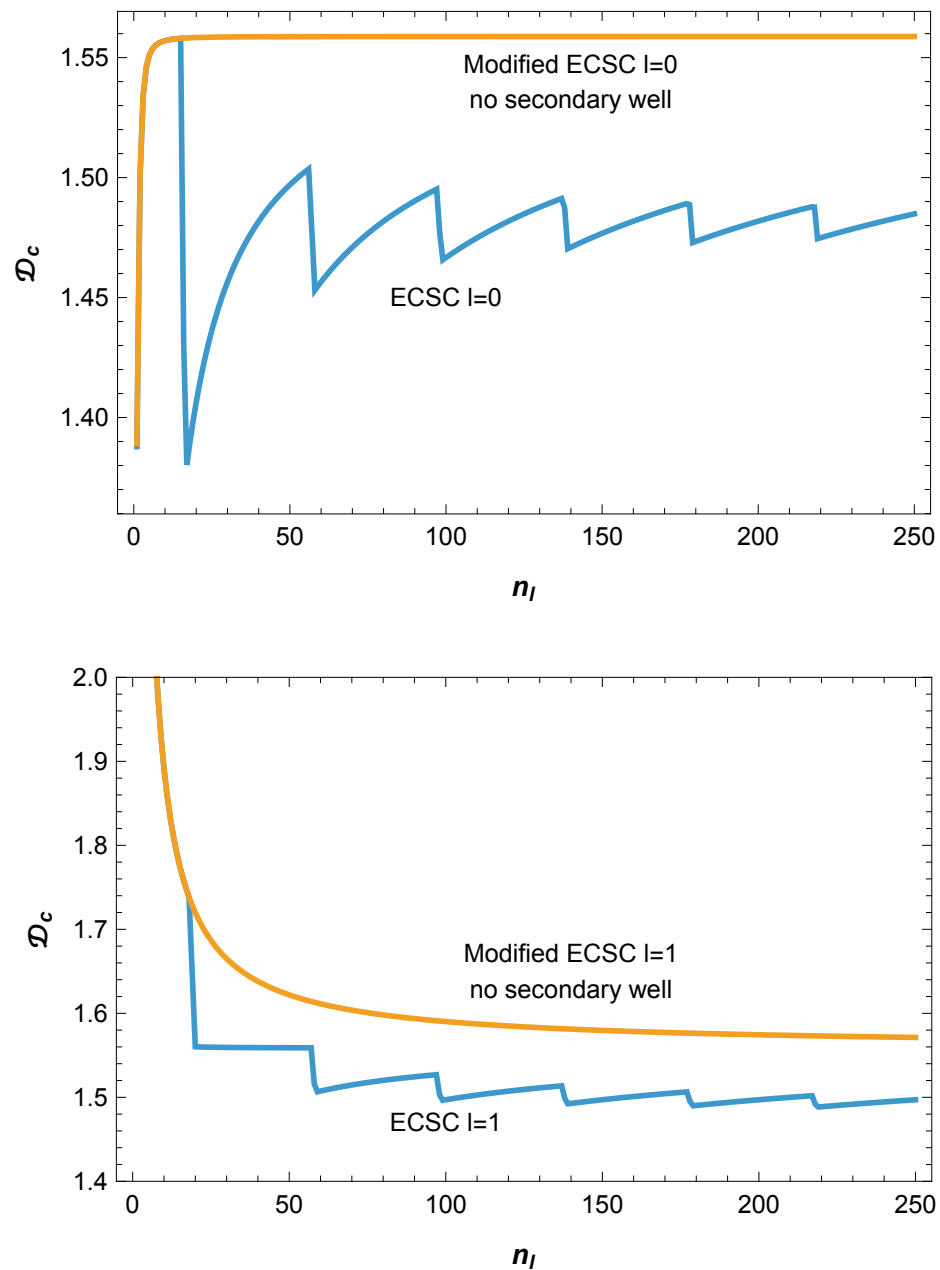
Figure 3. Comparison of \mathcal{D}_c/n^2 vs. n PM—calculated with and without secondary well for l = 0 and l = 1 . The blue curves refer to the well with the secondary well, and the orange curves without the secondary well. The secondary well is evidently necessary for the sawtooth structure to appear for \mathcal{D} \leq 10^5 au.
