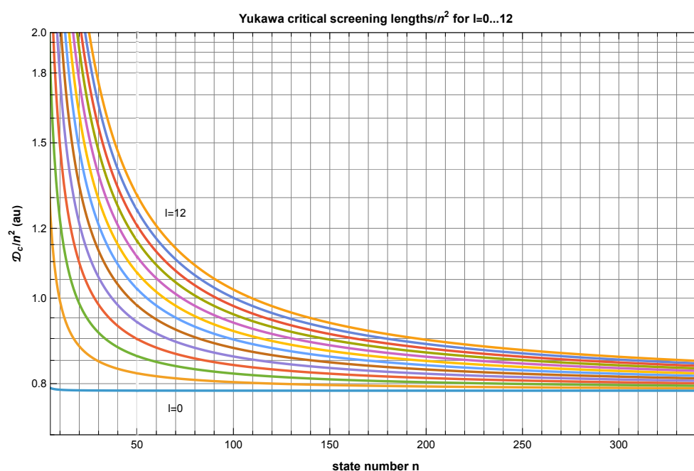
Figure 1. Yukawa \mathcal{D}_c/n^2 vs. state number n_l . The relatively featureless curves correspond to angular momenta increasing between l = 0 and l = 12 , each curve incrementing l by 1 between those limits. Colors are to aid in visually distinguishing the curves.
