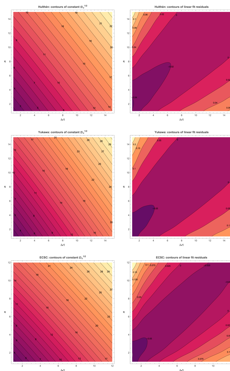
Figure 16. Contour plot of \sqrt{\mathcal{D}_c} vs. l + 1 and n , and residuals from bivariate linear fit to PM-calculated values computed to 30-digit accuracy. The nearly parallel and equally spaced contours indicate near-linearity.
