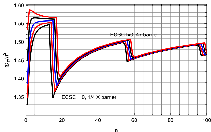
Figure 5. \mathcal{D}_c/n^2 vs. n for ECSC l=0 potential with barrier height between primary and secondary wells ( z = (\pi/2, 3\pi/2) ) changed by barrier scale factors of (from top curve) \text{bsf} = 1/4, 1/2, 1, 2, 4 . Colors are to aid in visually distinguishing the curves. Reducing the barrier height lowers the n of first onset of the sawtooth structure, but does not appreciably change its period. In this plot the range of n is reduced to better show the displacements between the curves.
