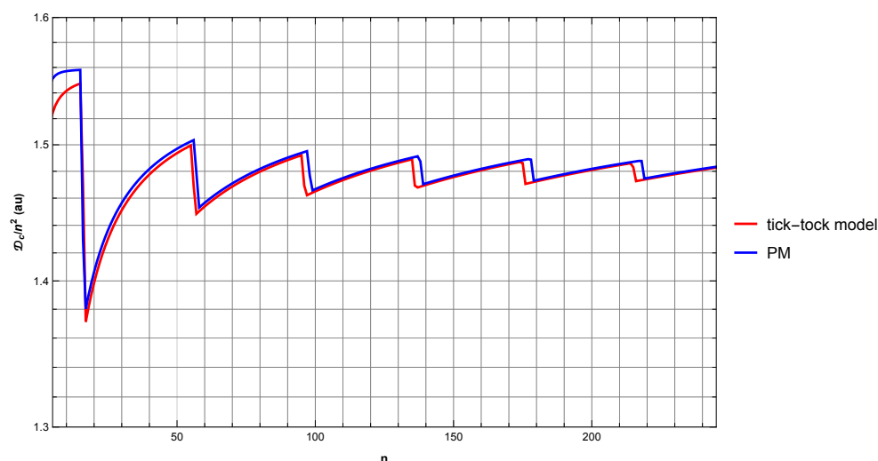
Figure 6. \mathcal{D}_c/n^2 vs. n (red curve) theoretically calculated using neoclassical phase-space quantization, with nominal value neoclassical parameters ( \nu_1 = 1/18 , \nu_2 = 6/10 ) for comparison. These represent intentional small deviations from canonical semiclassical values (0, 1/2 ), as described in the text. The PM-computed (essentially exact) result is shown in blue. Agreement could be improved by allowing \nu_1 and \nu_2 to be functions of n but, for simplicity, here we take them as constants. Our purpose is to show the basic origin of the sawtooth structure.
