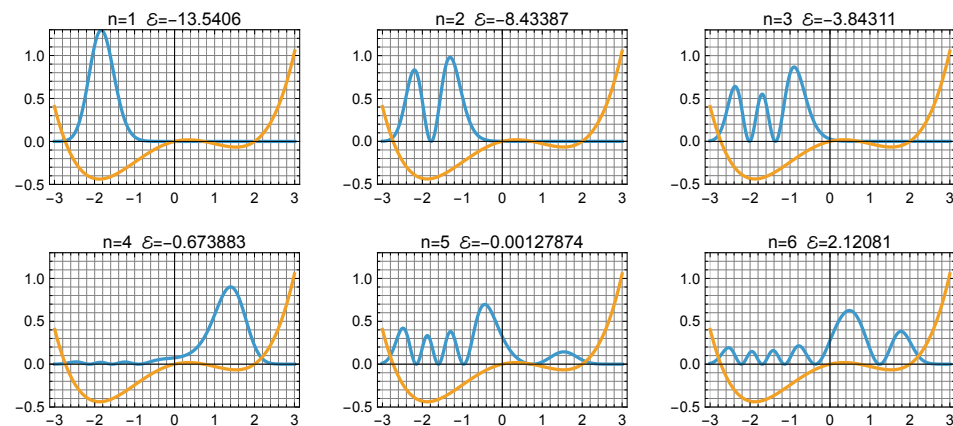
Figure 10. PM-calculated probability distributions (squared wavefunctions) for the asymmetric quartic double-well potential. The probability (squared wave function, blue curve) is shown, superimposed on the potential (orange curve) to show where it is spatially distributed
