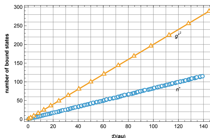
Figure 13. Plot of g^{*2} (square of maximum number of bound l = 0 states and n^* (total number of bound states of all l ) as a function of screening length \mathcal{D} , for the Hulthén potential. The range is limited so that no states for l > 12 fall within the data range as they are not represented in the dataset. Calculations were done by the Phase Method, as described previously. The same kind of linear behavior is found as was found for Yukawa and ECSC potentials.
