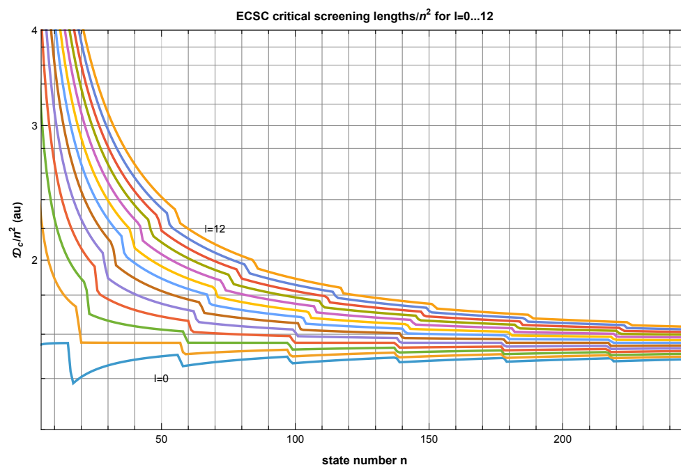
Figure 2. ECSC \mathcal{D}_c/n^2 vs. state number n_l . The curves correspond to angular momenta increasing between l = 0 and l = 12 , each curve incrementing l by 1 between those limits. Colors are to aid in visually distinguishing the curves. The structure repeats \Delta n_l \approx 40 states.
