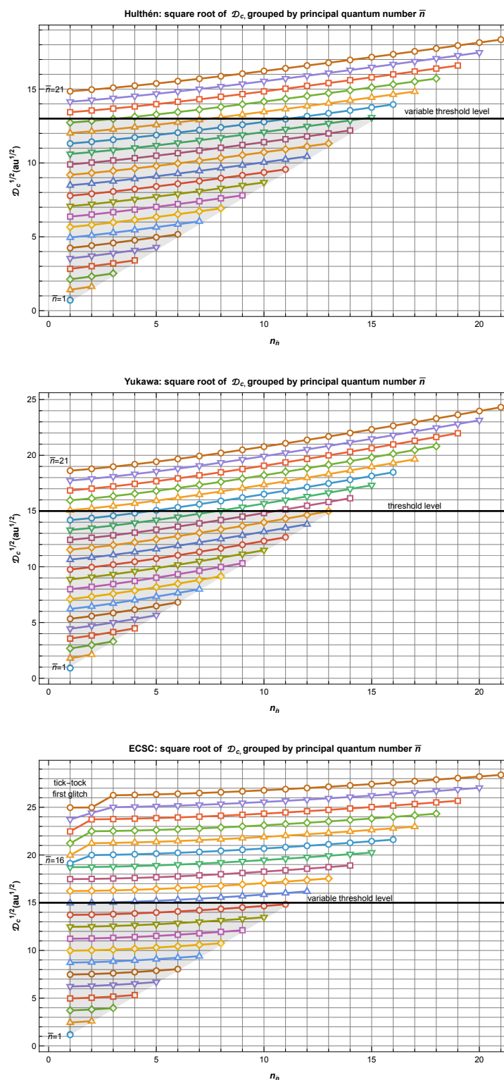
Figure 15. \sqrt{\mathcal{D}_c} vs. n_{\bar{n}} and l . The curves in the left panels correspond to increasing values of n starting with n=1 . Each curve increments n by 1 between n=1 and the upper n values as shown, which differ for the three potentials. The curves in the right panels similarly correspond to increasing values of l starting with l=0 . Each curve increments l by 1 between l=0 and the upper l values as shown, which differ for the three potentials. The average density of states is approximately constant in this representation also, extending indefinitely in n and l (modulo tick-tock glitches). The lowest state is 1s, the second pair is 2s, 2p, etc. Note the tick-tock glitch at n > 15 for ECSC potential.
