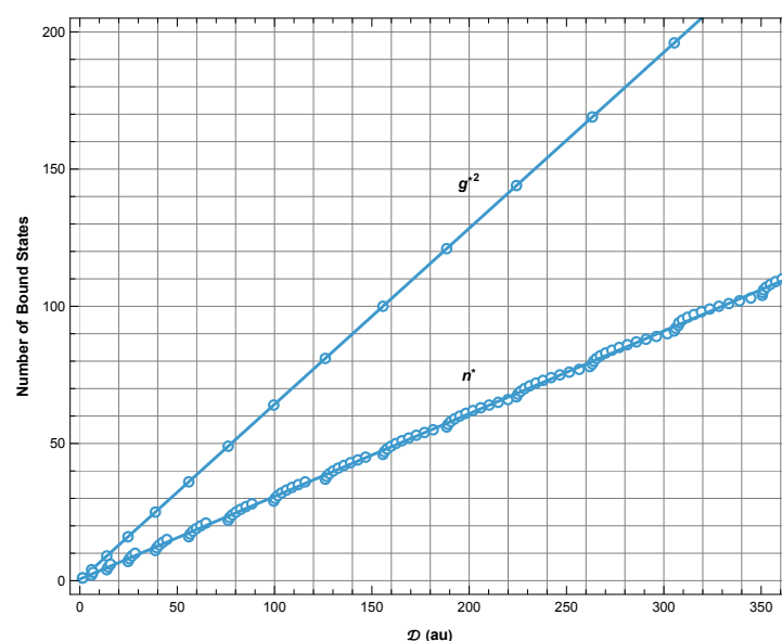
Figure 12. Plot of g^{*2} (square of maximum number of bound l = 0 states and n^* (total number of bound states of all l ) as a function of screening length \mathcal{D} , for the ECSC potential. The range is chosen for comparison with Lam and Varshni [3], Figure 2. The first tick-tock glitch is slightly above this range. Calculations were done by the Phase Method, as previously described. Note the 1-2-3-4... state-binding pattern observed along the n^* line. These correspond to (1s), (2s, 2p), (3s, 3p, 3d), etc. A similar pattern is not found for the other potentials because the states of different principal quantum number overlap for them.
