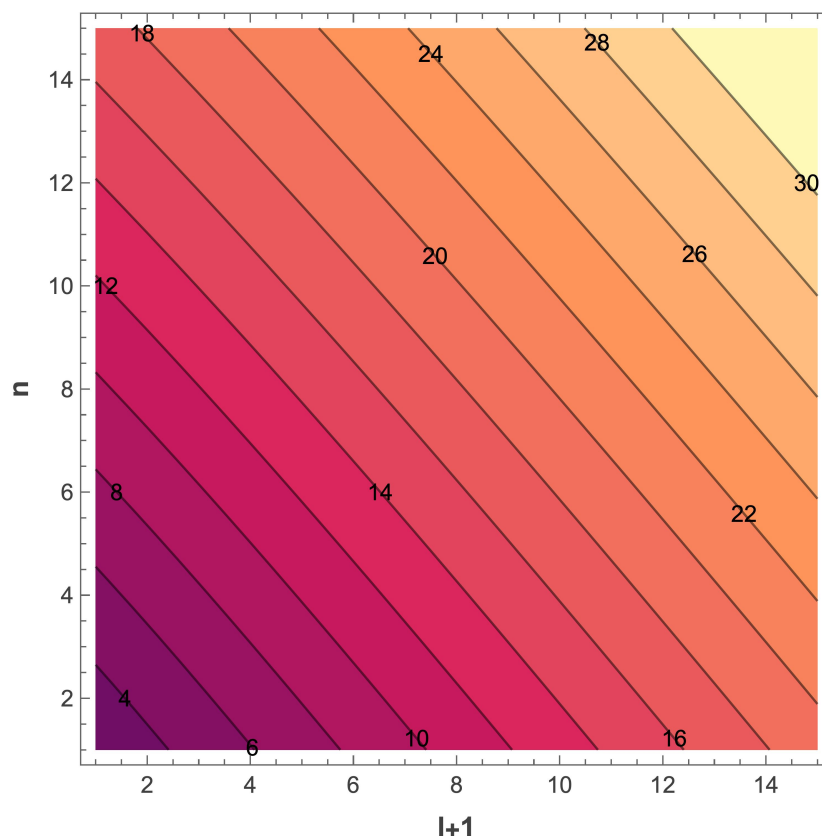
Figure 17. \sqrt{\mathcal{D}_c} vs. n_{\bar{n}} and l + 1 for Yukawa potential, as calculated by first-order perturbation theory. The unperturbed potential is Coulomb, and the difference between the Yukawa and Coulomb potentials was used as a perturbation. The displayed \mathcal{D}_c values are those values required for the perturbed eigenvalues to be shifted up to zero energy. Computations were done analytically in Mathematica, but are rough in comparison with the PM-calculated values in Figure 9. The key feature of interest is the striking linear relationship between \mathcal{D}_c^{1/2} and n and l , which is maintained despite the rough and approximate nature of this first-order PT calculation.
