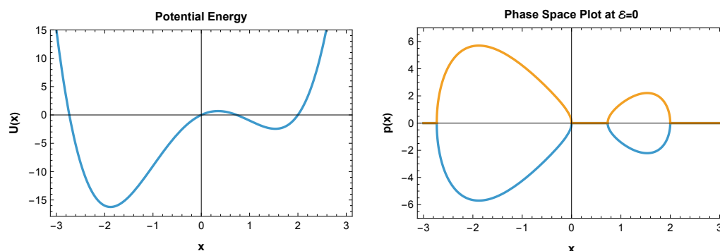
Figure 9. Asymmetric quartic double-well potential is shown. The right panel shows a plot of the phase space accessible at \mathcal{E} = 0 . The left (right) region corresponds to the left (right) well. p(x) is the momentum, with the positive (orange) and negative (blue) branches shown on the right.
