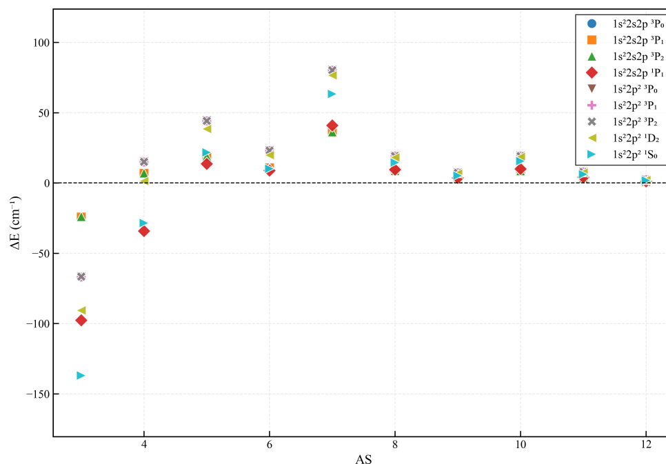
Figure 1. Convergence for excitation energies with enlarging active set (AS), where \Delta E represents the energy change between AS_{n-1} and AS_n .
